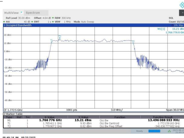
N66-15KHz-15MHz-DFT-s-OFDM QPSK-354500-75RB#0-13.5-14.6
