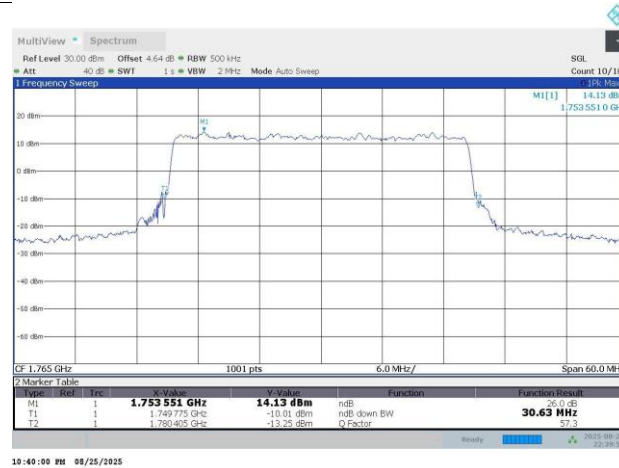
N66-15KHz-30MHz-CP-OFDM QPSK-353000-160RB#0-28.61-30.63
