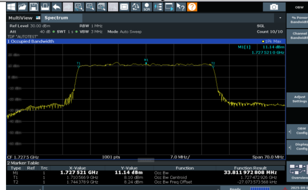
N66-15KHz-35MHz-CP-OFDM 256QAM-345500-188RB#0-33.81-37.20
