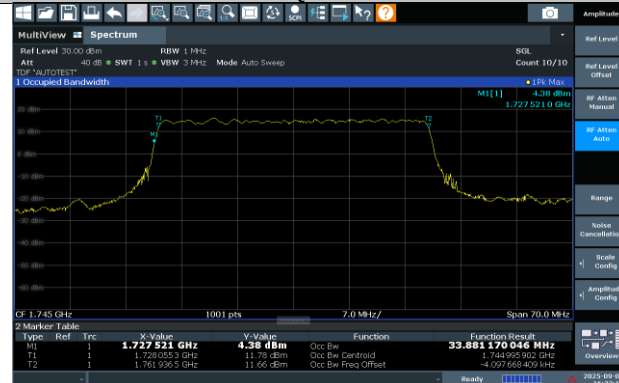
N66-15KHz-35MHz-CP-OFDM QPSK-349000-188RB#0-33.88-36.85
