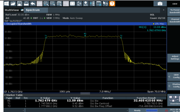
N66-15KHz-35MHz-DFT-s-OFDM 256QAM-352500-180RB#0-32.41-35.94
