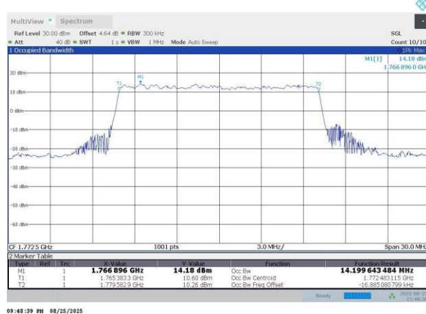
N66-15KHz-15MHz-CP-OFDM QPSK-354500-79RB#0-14.2-15.4
