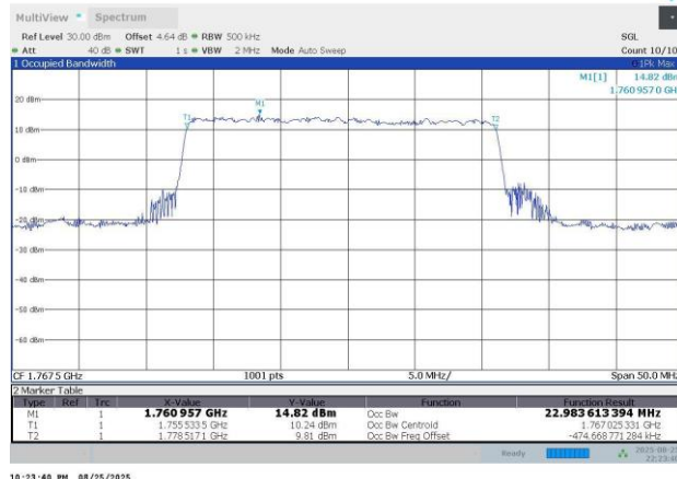
N66-15KHz-25MHz-DFT-s-OFDM QPSK-353500-128RB#0-22.98-24.48
