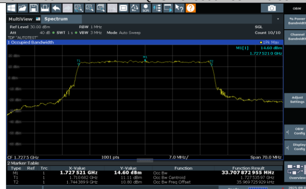
N66-15KHz-35MHz-CP-OFDM QPSK-345500-188RB#0-33.71-37.48
