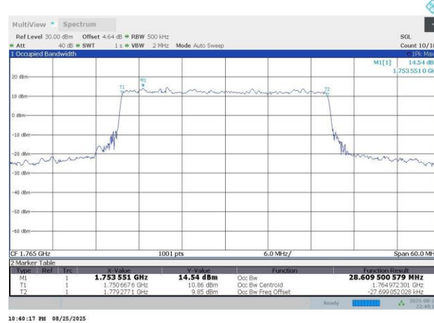
N66-15KHz-30MHz-CP-OFDM QPSK-353000-160RB#0-28.61-30.63
