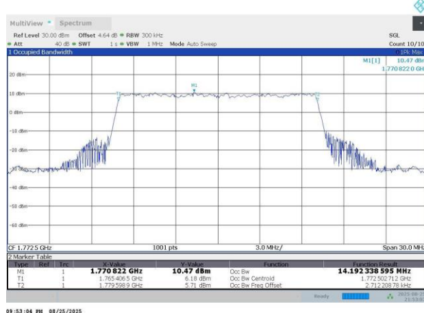
N66-15KHz-15MHz-CP-OFDM 256QAM-354500-79RB#0-14.19-15.52
