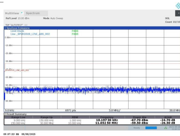
N66-15KHz-5MHz-DFT-s-OFDM PI/2 BPSK-342500-1RB#0-PASS
