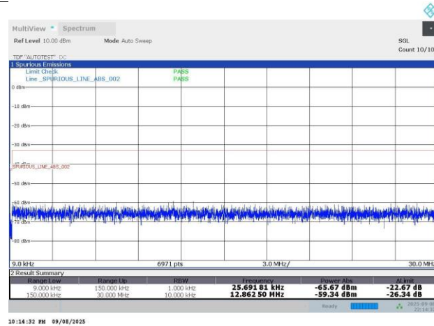
N66-15KHz-20MHz-DFT-s-OFDM QPSK-349000-1RB#105-PASS
