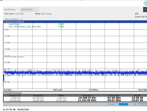
N66-15KHz-40MHz-DFT-s-OFDM PI/2 BPSK-346000-1RB#215-PASS
