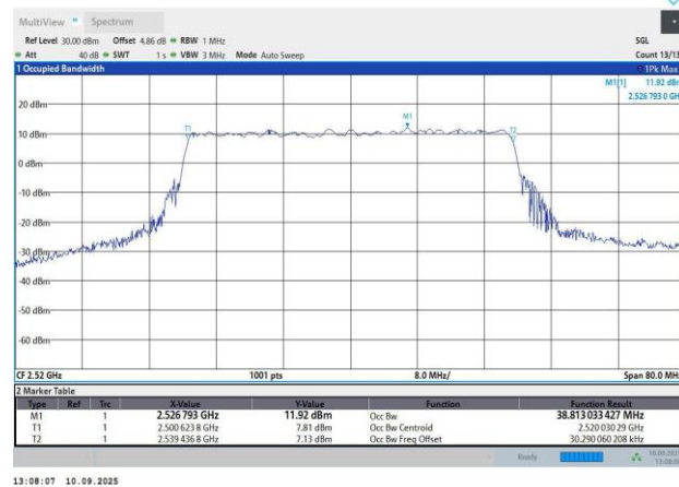
N7-15KHz-40MHz-CP-OFDM 256QAM-504000-216RB#0-38.81-41.64
