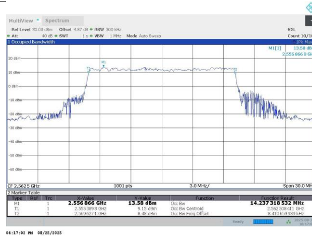
N7-15KHz-15MHz-CP-OFDM QPSK-512500-79RB#0-14.24-15.46
