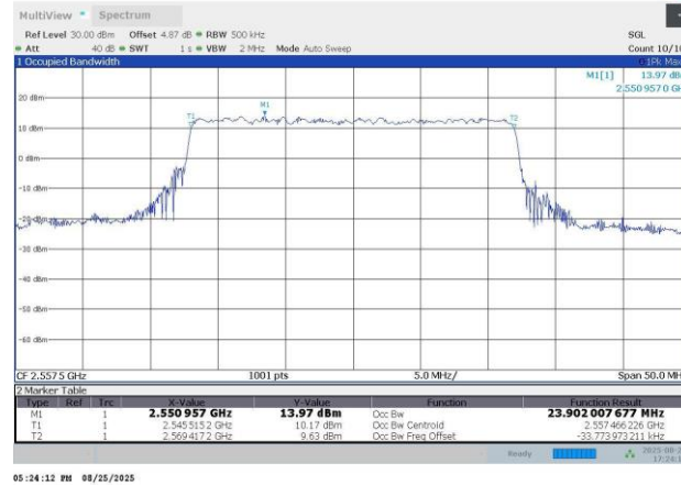
N7-15KHz-25MHz-CP-OFDM QPSK-511500-133RB#0-23.9-25.97
