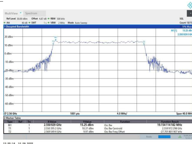
N7-15KHz-20MHz-CP-OFDM QPSK-512000-106RB#0-19.15-21.26
