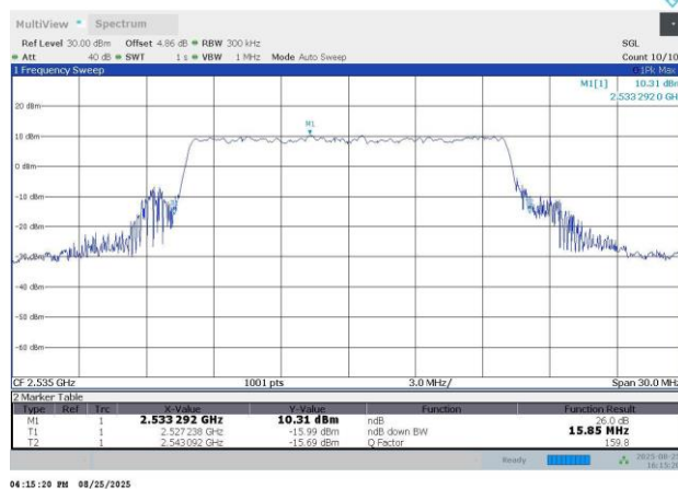
N7-15KHz-15MHz-CP-OFDM 256QAM-507000-79RB#0-14.22-15.85
