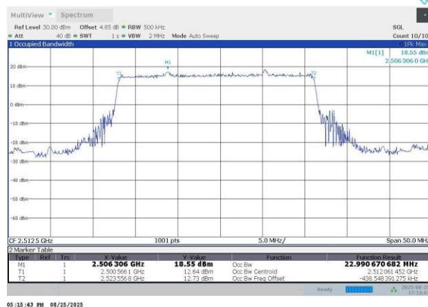
N7-15KHz-25MHz-DFT-s-OFDM PI/2 BPSK-502500-128RB#0-22.99-25.18
