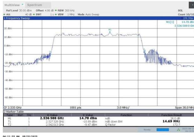
N7-15KHz-15MHz-DFT-s-OFDM QPSK-507000-75RB#0-13.55-14.69
