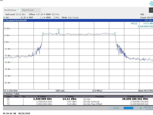
N7-15KHz-30MHz-CP-OFDM QPSK-511000-160RB#0-28.7-31.53
