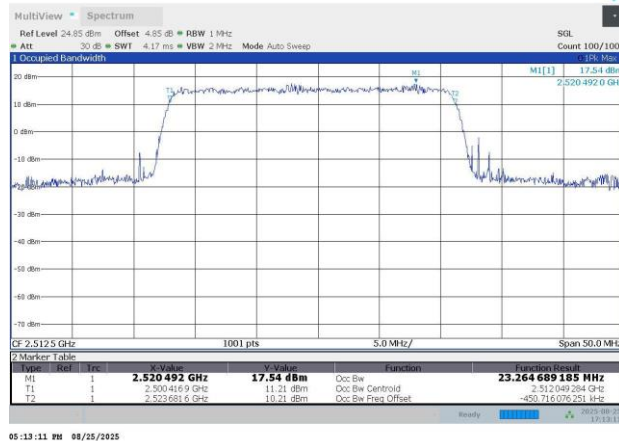
N7-15KHz-25MHz-DFT-s-OFDM QPSK-502500-128RB#0-23.26-28.12
