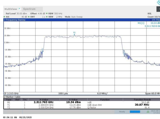
N7-15KHz-30MHz-CP-OFDM 256QAM-503000-160RB#0-28.71-30.87
