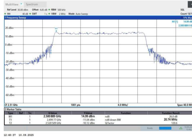
N7-15KHz-20MHz-CP-OFDM QPSK-502000-106RB#0-19.16-20.74
