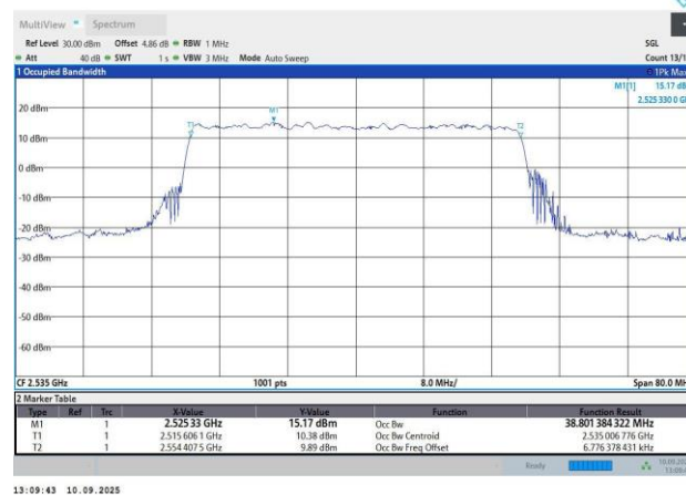
N7-15KHz-40MHz-CP-OFDM QPSK-507000-216RB#0-38.8-41.64
