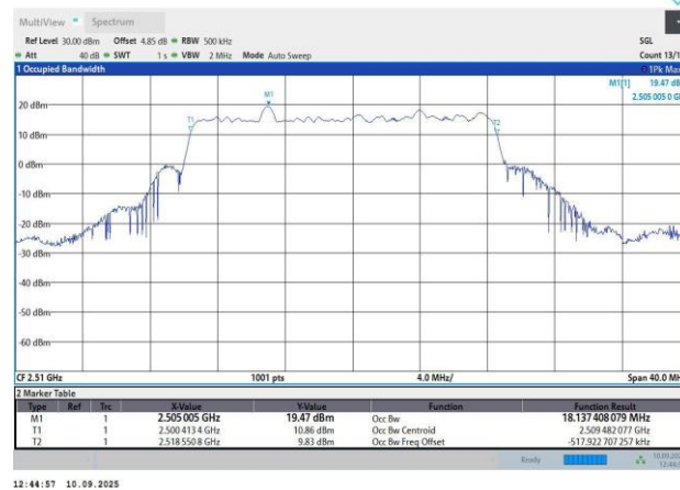
N7-15KHz-20MHz-DFT-s-OFDM PI/2 BPSK-502000-100RB#0-18.14-20.46
