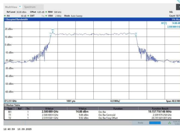
N7-15KHz-20MHz-CP-OFDM QPSK-502000-106RB#0-19.16-20.74
