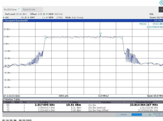
N7-15KHz-25MHz-CP-OFDM 256QAM-502500-133RB#0-23.81-25.43
