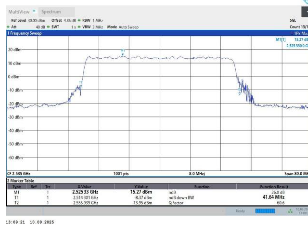
N7-15KHz-40MHz-CP-OFDM QPSK-507000-216RB#0-38.8-41.64
