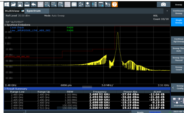
N7-15KHz-20MHz-DFT-s-OFDM PI/2 BPSK-502000-1RB#0-PASS
