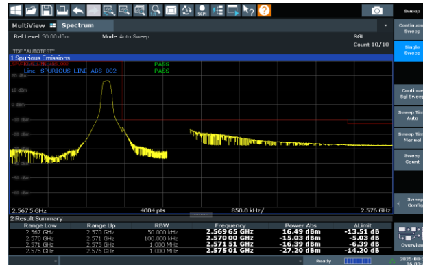
N7-15KHz-5MHz-DFT-s-OFDM PI/2 BPSK-513500-1RB#24-PASS
