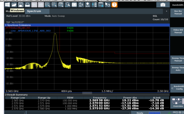
N7-15KHz-10MHz-DFT-s-OFDM PI/2 BPSK-513000-1RB#51-PASS
