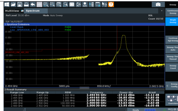
N7-15KHz-5MHz-CP-OFDM QPSK-500500-1RB#0-PASS
