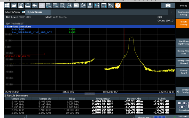
N7-15KHz-5MHz-DFT-s-OFDM QPSK-500500-1RB#0-PASS
