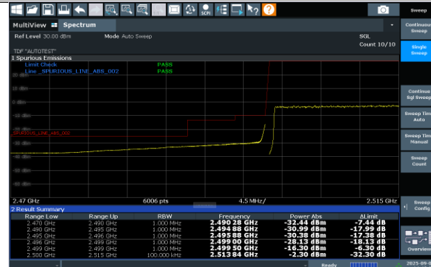
N7-15KHz-30MHz-DFT-s-OFDM QPSK-503000-160RB#0-PASS
