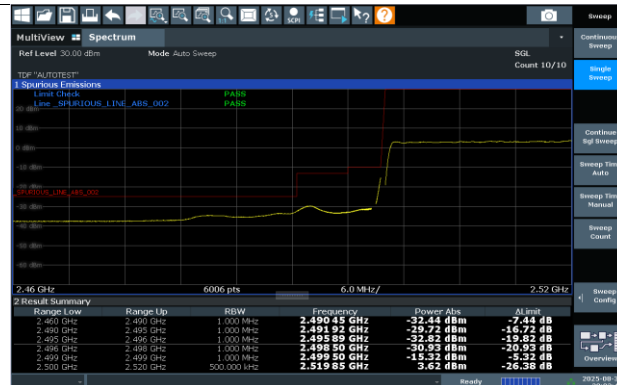
N7-15KHz-40MHz-DFT-s-OFDM PI/2 BPSK-504000-216RB#0- PASS
