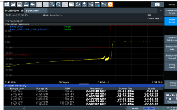
N7-15KHz-20MHz-DFT-s-OFDM QPSK-502000-100RB#0-PASS
