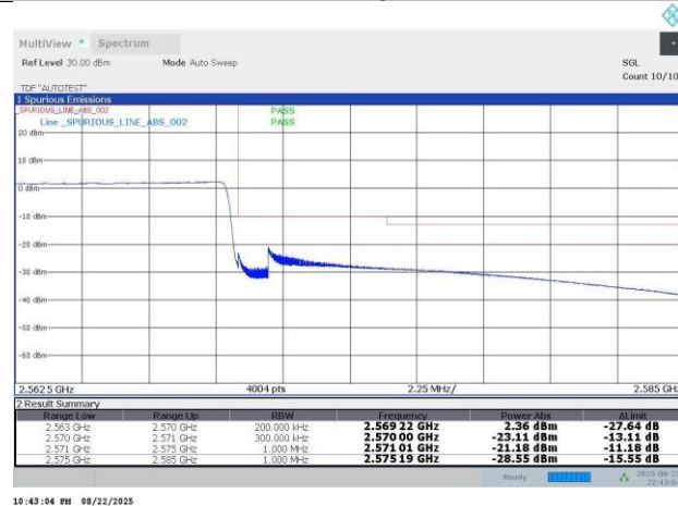
N7-15KHz-15MHz-CP-OFDM QPSK-512500-79RB#0-PASS
