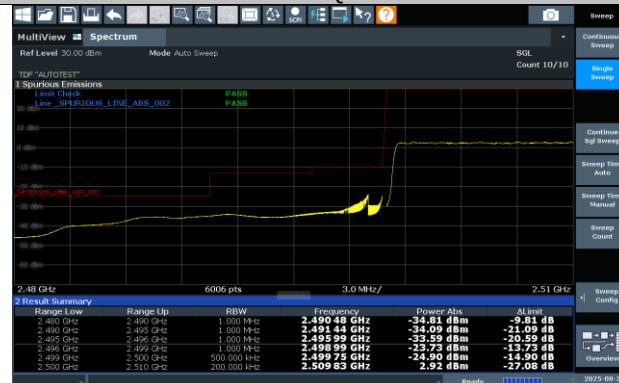
N7-15KHz-20MHz-DFT-s-OFDM PI/2 BPSK-502000-100RB#0-PASS
