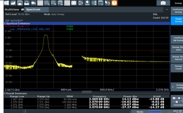
N7-15KHz-5MHz-CP-OFDM QPSK-513500-1RB#24-PASS
