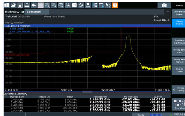
N7-15KHz-5MHz-DFT-s-OFDM PI/2 BPSK-500500-1RB#0-PASS
