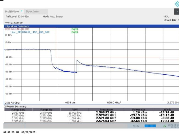
N7-15KHz-5MHz-CP-OFDM QPSK-513500-25RB#0-PASS
