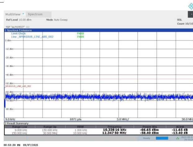
N7-15KHz-5MHz-DFT-s-OFDM PI/2 BPSK-500500-1RB#0-PASS
