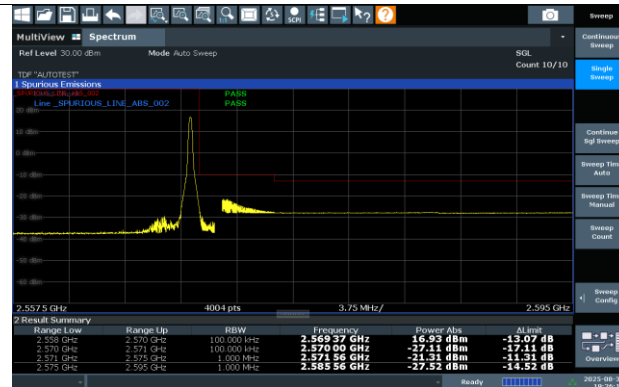
N7-15KHz-25MHz-CP-OFDM QPSK-511500-1RB#132- PASS
