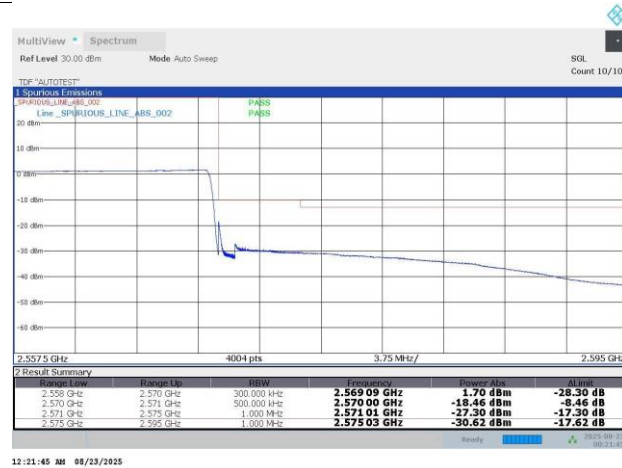
N7-15KHz-25MHz-CP-OFDM QPSK-511500-133RB#0-PASS
