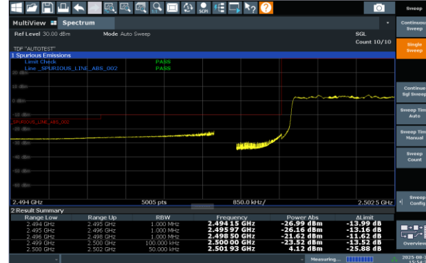
N7-15KHz-5MHz-DFT-s-OFDM PI/2 BPSK-500500-25RB#0-PASS
