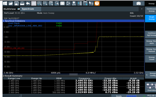
N7-15KHz-40MHz-CP-OFDM QPSK-504000-216RB#0- PASS
