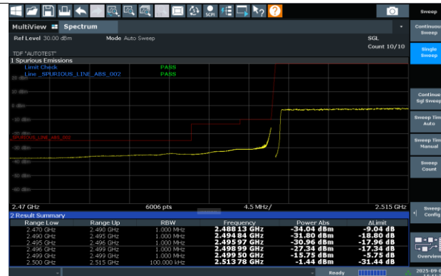
N7-15KHz-30MHz-DFT-s-OFDM PI/2 BPSK-503000-160RB#0-PASS
