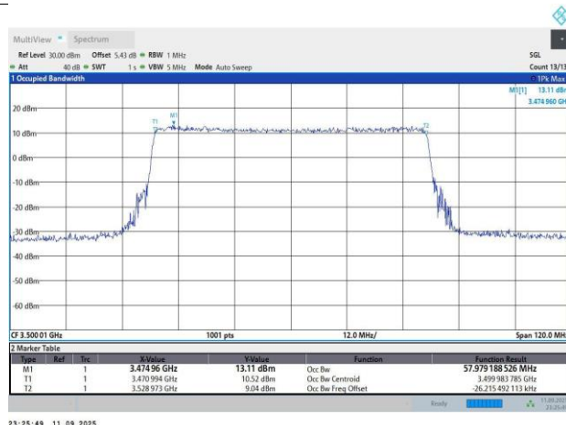
N77-30KHz-60MHz-CP-OFDM QPSK-633334-162RB#0-57.98-61.5
