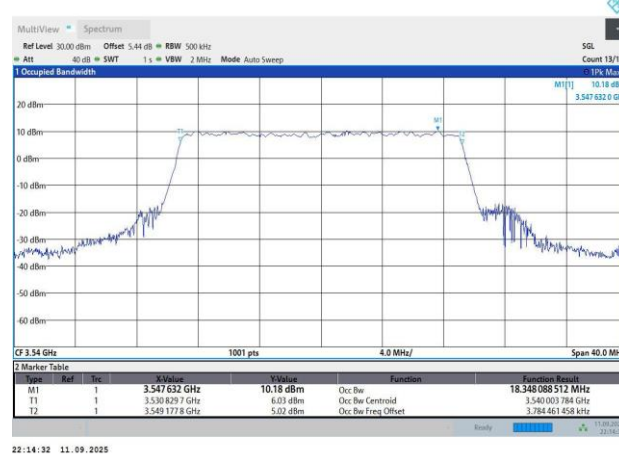
N77-30KHz-20MHz-CP-OFDM 256QAM-636000-51RB#0-18.35-20.42
