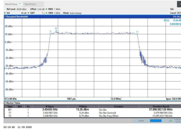
N77-30KHz-60MHz-DFT-s-OFDM QPSK-632000-162RB#0-58.0-61.14
