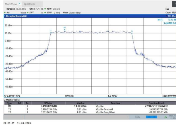
N77-30KHz-30MHz-CP-OFDM QPSK-633334-78RB#0-27.94-30.21
