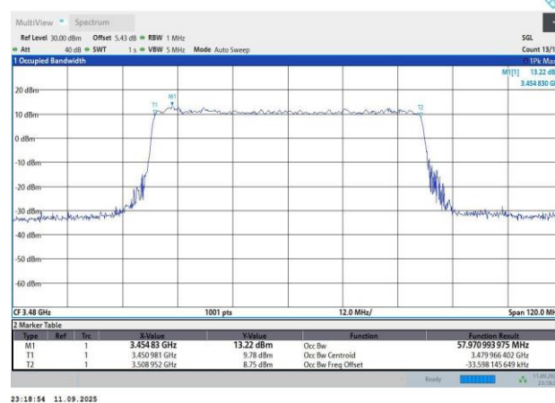
N77-30KHz-60MHz-CP-OFDM QPSK-632000-162RB#0-57.97-61.26
