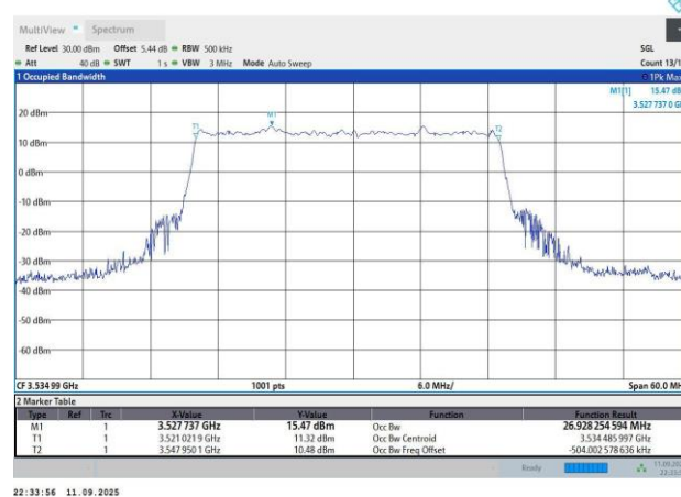
N77-30KHz-30MHz-DFT-s-OFDM PI/2 BPSK-635666-75RB#0-26.93-29.13
