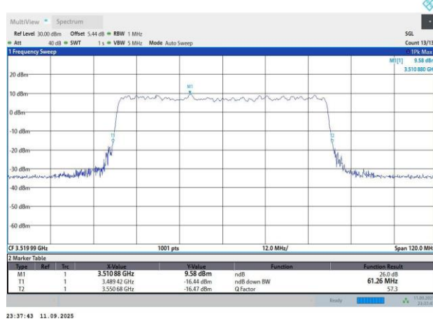
N77-30KHz-60MHz-CP-OFDM 256QAM-634666-162RB#0-57.81-61.26
