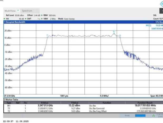
N77-30KHz-20MHz-DFT-s-OFDM QPSK-636000-50RB#0-18.02-19.94
