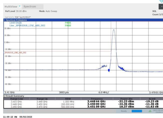
N77-30KHz-40MHz-DFT-s-OFDM PI/2 BPSK-631334-1RB#0-PASS
