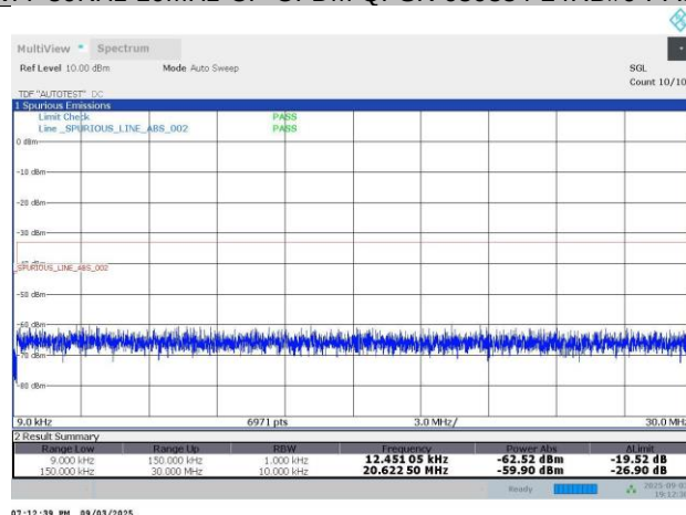
N77-30KHz-10MHz-DFT-s-OFDM PI/2 BPSK-633334-1RB#0-PASS
