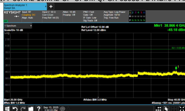
N77-30KHz-10MHz-CP-OFDM QPSK-630334-24RB#0-PASS
