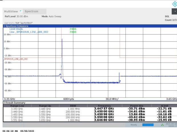
N77-30KHz-100MHz-DFT-s-OFDM QPSK-633334-1RB#0-PASS
