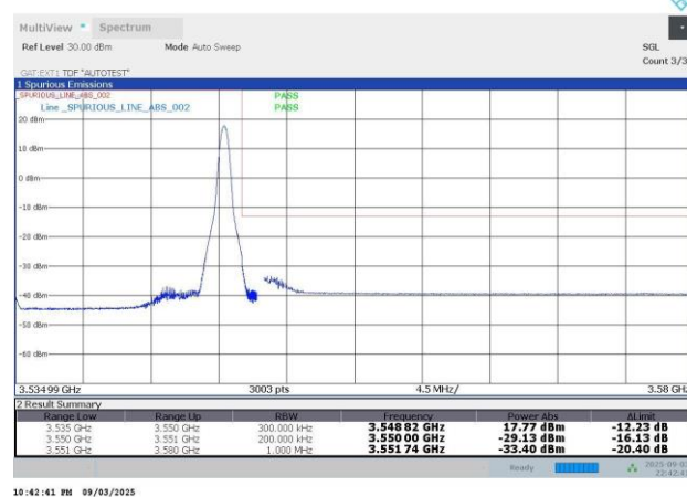
N77-30KHz-30MHz-DFT-s-OFDM PI/2 BPSK-635666-1RB#77-PASS
