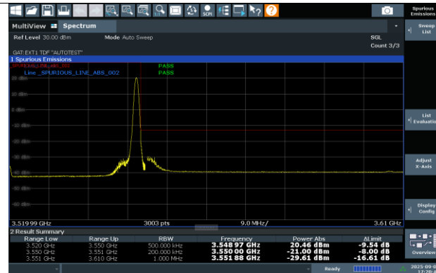
N77-30KHz-60MHz-DFT-s-OFDM QPSK-634666-1RB#161-PASS
