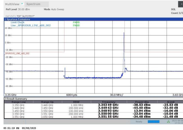
N77-30KHz-100MHz-CP-OFDM QPSK-633334-1RB#272-PASS
