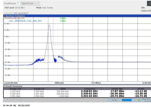
N77-30KHz-30MHz-DFT-s-OFDM QPSK-635666-1RB#77-PASS
