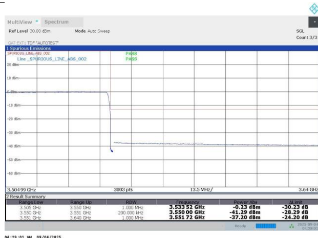
N77-30KHz-90MHz-CP-OFDM QPSK-633666-245RB#0-PASS
