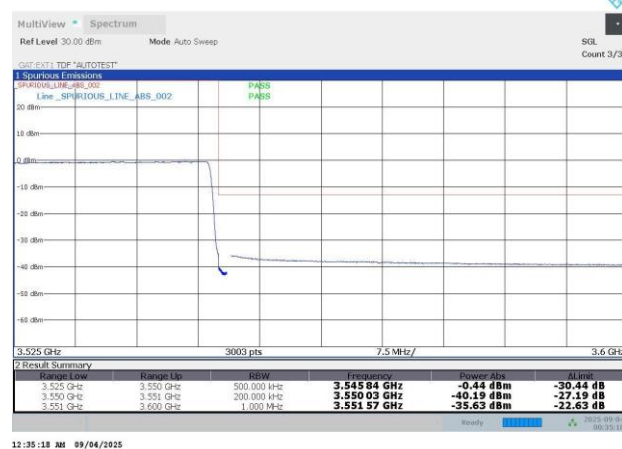
N77-30KHz-50MHz-CP-OFDM QPSK-635000-133RB#0-PASS
