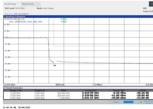
N77-30KHz-50MHz-DFT-s-OFDM QPSK-635000-128RB#0-PASS
