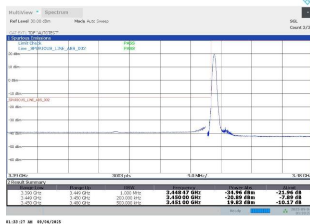
N77-30KHz-60MHz-DFT-s-OFDM PI/2 BPSK-632000-1RB#0-PASS
