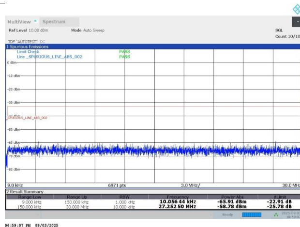
N77-30KHz-10MHz-DFT-s-OFDM PI/2 BPSK-630334-1RB#0-PASS
