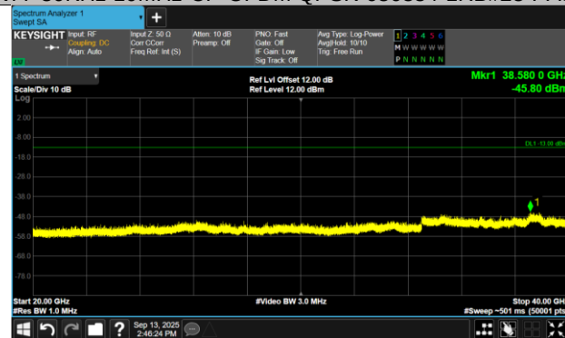
N77-30KHz-10MHz-CP-OFDM QPSK-636334-1RB#23-PASS
