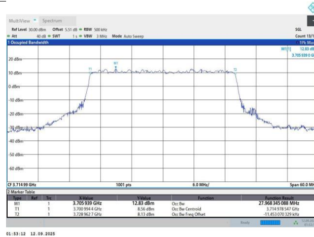
N77-30KHz-30MHz-CP-OFDM QPSK-647666-78RB#0-27.97-30.27
