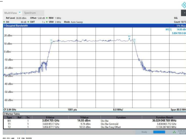
N77-30KHz-40MHz-DFT-s-OFDM QPSK-656000-100RB#0-36.02-39.4
