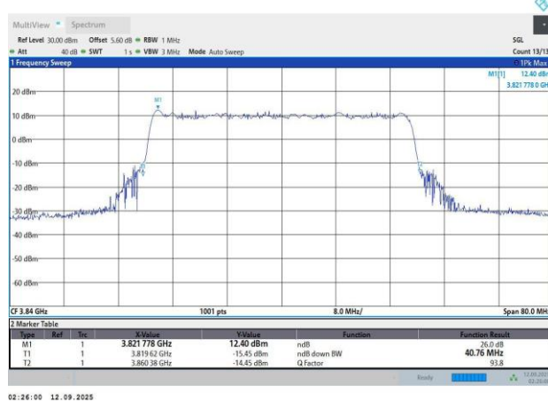
N77-30KHz-40MHz-CP-OFDM 256QAM-656000-106RB#0-38.11-40.76
