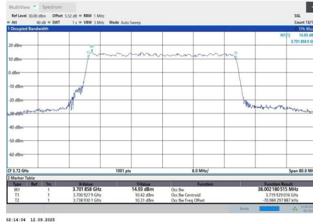
N77-30KHz-40MHz-CP-OFDM QPSK-648000-106RB#0-38.0-41
