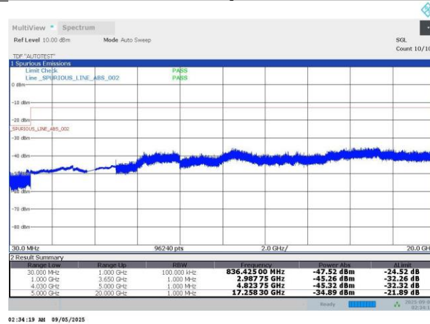
N77-30KHz-50MHz-CP-OFDM QPSK-648334-1RB#132-PASS
