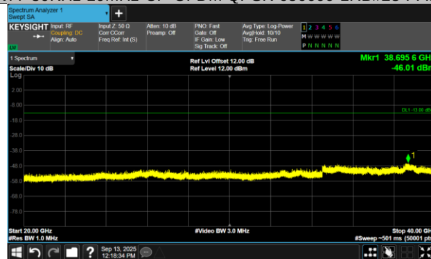
N77-30KHz-10MHz-CP-OFDM QPSK-656000-1RB#23-PASS
