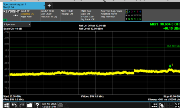
N77-30KHz-10MHz-DFT-s-OFDM QPSK-647000-1RB#0-PASS
