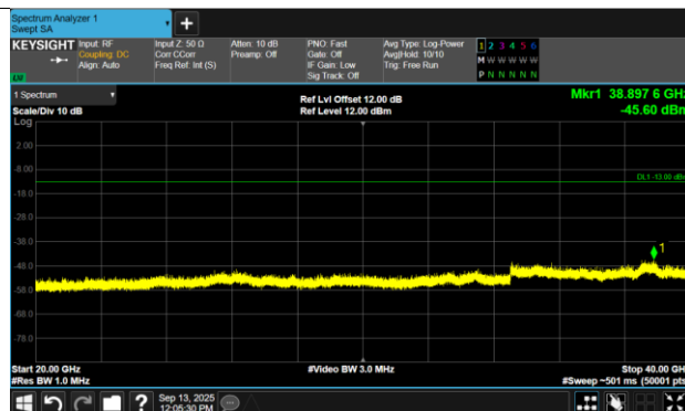
N77-30KHz-10MHz-DFT-s-OFDM PI/2 BPSK-647000-1RB#0-PASS
