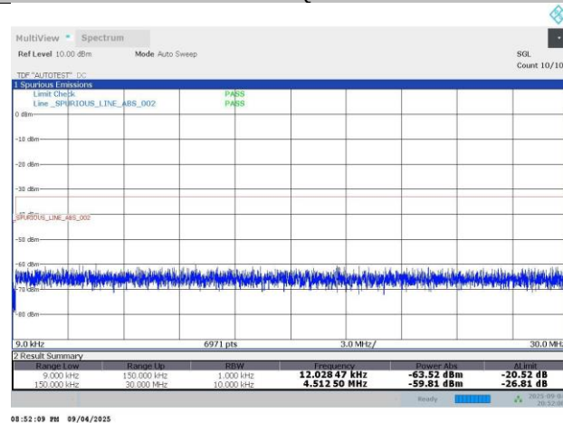
N77-30KHz-10MHz-DFT-s-OFDM PI/2 BPSK-656000-24RB#0-PASS
