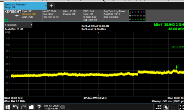
N77-30KHz-100MHz-CP-OFDM QPSK-662000-1RB#0-PASS
