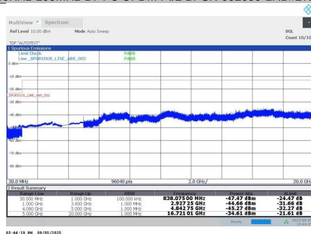
N77-30KHz-100MHz-DFT-s-OFDM PI/2 BPSK-662000-1RB#272-PASS
