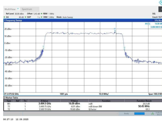
N78-30KHz-50MHz-CP-OFDM QPSK-631668-133RB#0-47.63-50.45
