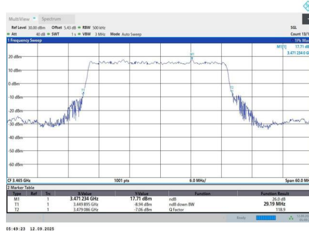
N78-30KHz-30MHz-DFT-s-OFDM PI/2 BPSK-631000-75RB#0-26.92-29.19
