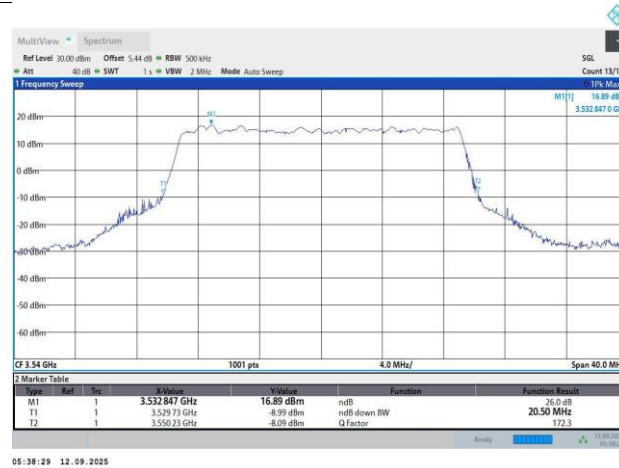
N78-30KHz-20MHz-CP-OFDM QPSK-636000-51RB#0-18.45-20.5
