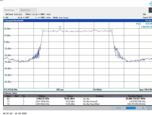
N78-30KHz-50MHz-DFT-s-OFDM PI/2 BPSK-631668-128RB#0-45.89-49.25
