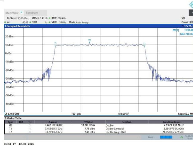
N78-30KHz-30MHz-CP-OFDM 256QAM-631000-78RB#0-27.92-30.15
