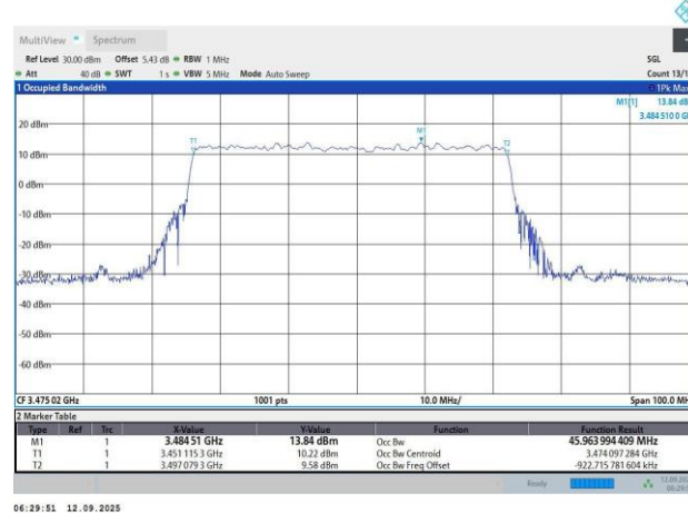
N78-30KHz-50MHz-DFT-s-OFDM 256QAM-631668-128RB#0-45.96-49.55
