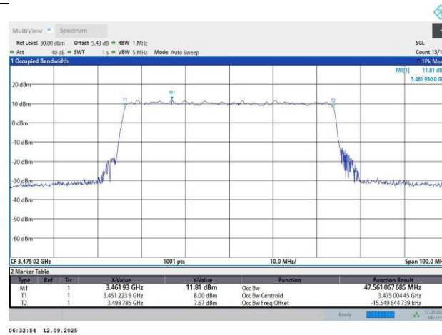
N78-30KHz-50MHz-CP-OFDM 256QAM-631668-133RB#0-47.56-50.85
