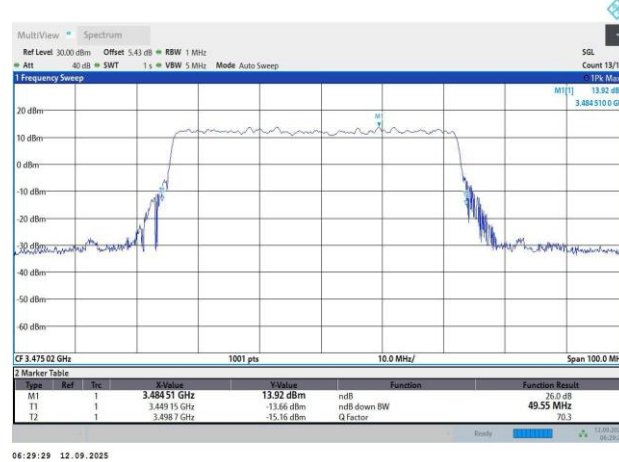
N78-30KHz-50MHz-DFT-s-OFDM 256QAM-631668-128RB#0-45.96-49.55
