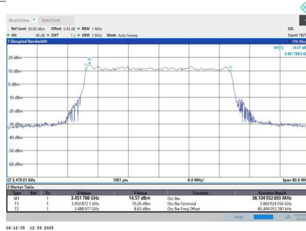
N78-30KHz-40MHz-CP-OFDM 256QAM-631334-106RB#0-38.1-41.40
