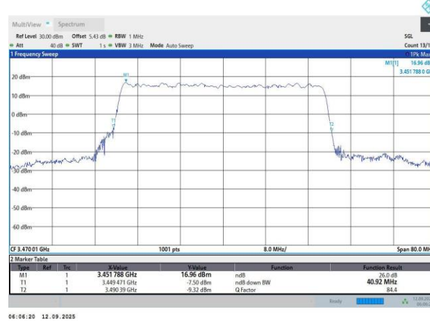
N78-30KHz-40MHz-CP-OFDM QPSK-631334-106RB#0-38.05-40.92
