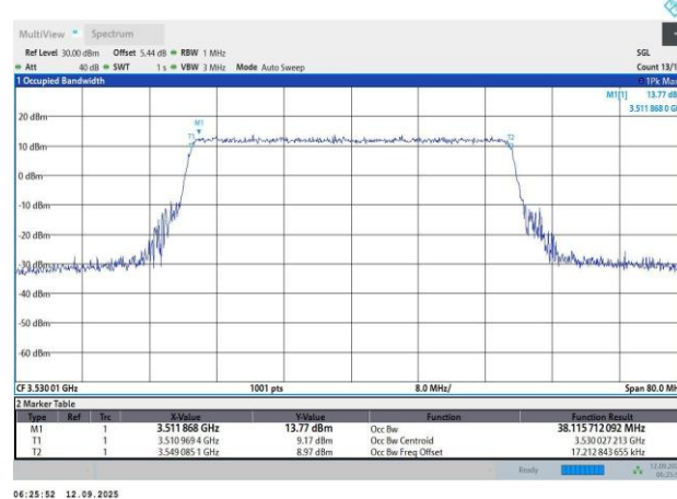
N78-30KHz-40MHz-CP-OFDM 256QAM-635334-106RB#0-38.12-41
