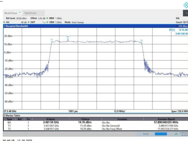
N78-30KHz-60MHz-DFT-s-OFDM QPSK-632000-162RB#0-57.89-61.74
