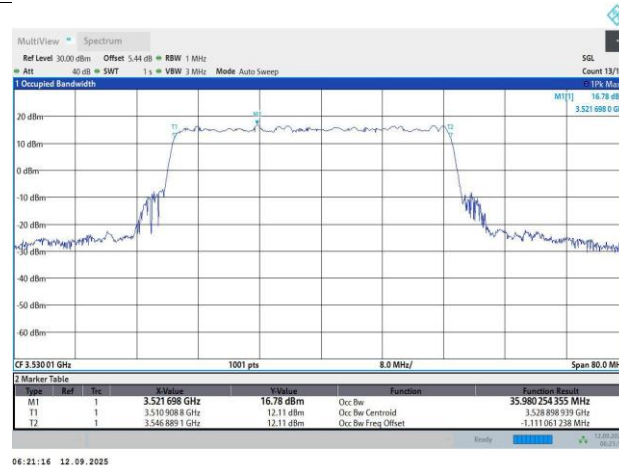
N78-30KHz-40MHz-DFT-s-OFDM QPSK-635334-100RB#0-35.98-39.32
