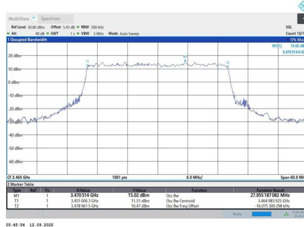
N78-30KHz-30MHz-CP-OFDM QPSK-631000-78RB#0-27.96-30.51
