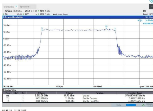
N78-30KHz-60MHz-CP-OFDM QPSK-632000-162RB#0-57.92-61.26
