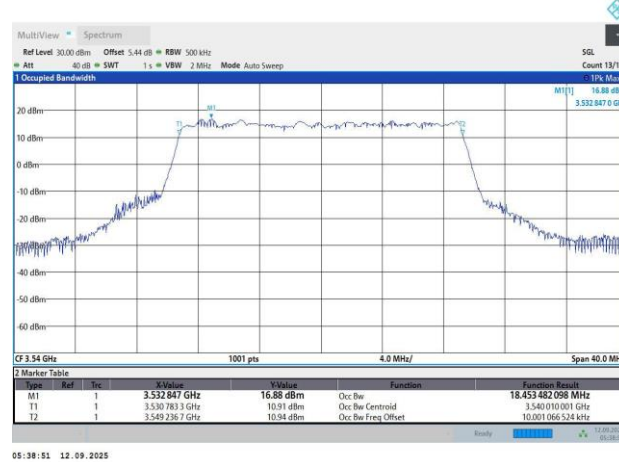
N78-30KHz-20MHz-CP-OFDM QPSK-636000-51RB#0-18.45-20.5
