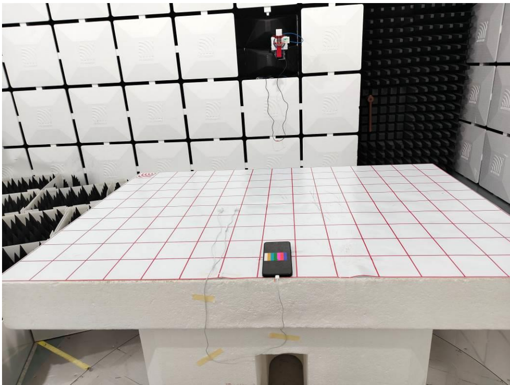
Radiated Disturbance Emissions (18GHz-40GHz)
