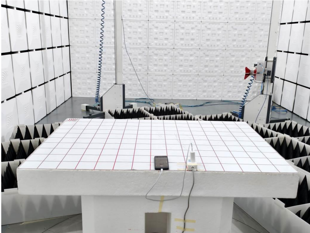
Radiated Disturbance Emissions (1GHz-18GHz)
