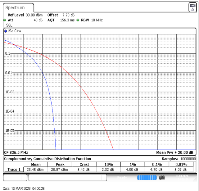
Band26(824-849)-10MHz-QPSK-26915-50RB#0-PASS
