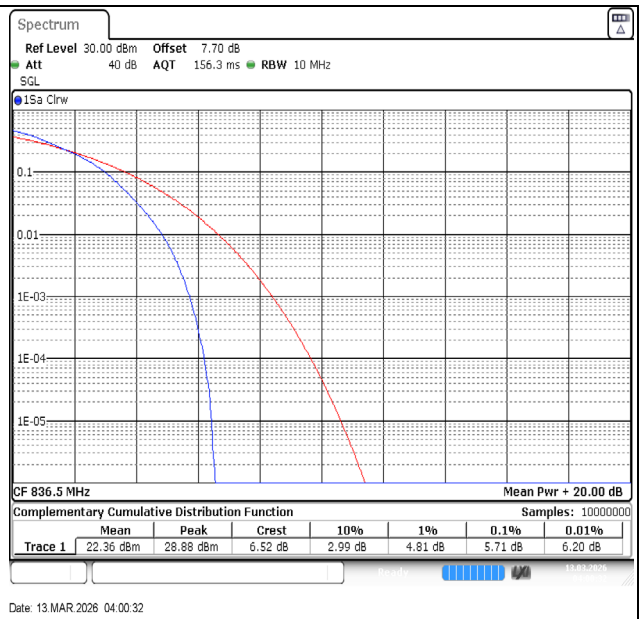
Band26(824-849)-10MHz-16QAM-26915-50RB#0-PASS
