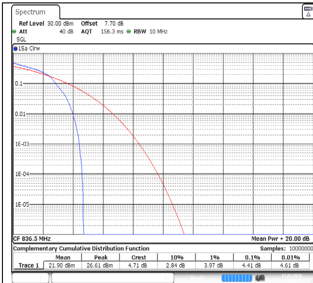
Band26(824-849)-10MHz-16QAM-26915-1RB#0-PASS
