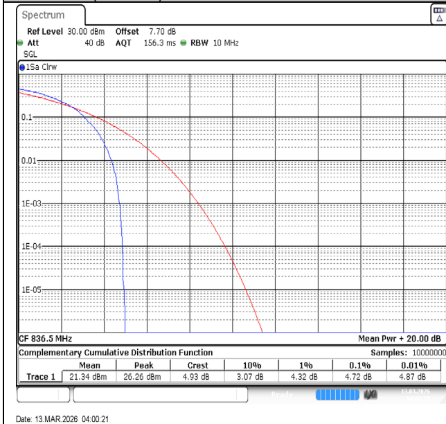
Band26(824-849)-10MHz-64QAM-26915-1RB#0-PASS
