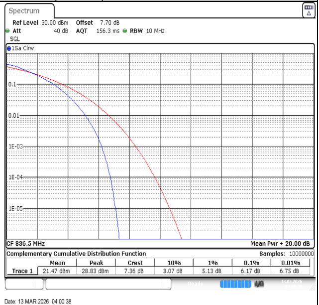
Band26(824-849)-10MHz-64QAM-26915-50RB#0-PASS
