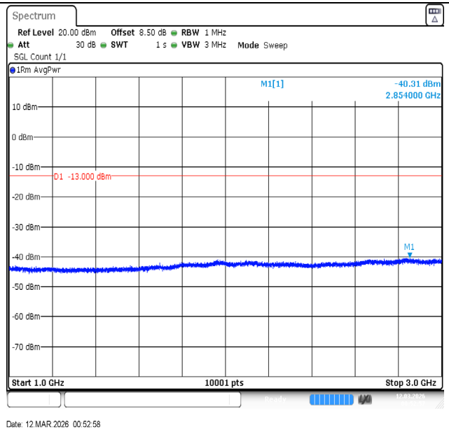
Band5-1.4MHz-QPSK-20643-6RB#0-1000~3000-PASS
