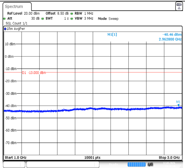
Band5-1.4MHz-QPSK-20525-1RB#5-1000~3000-PASS
