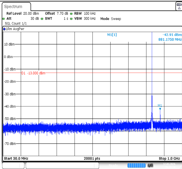
Band5-1.4MHz-QPSK-20525-1RB#5-30~1000-PASS
