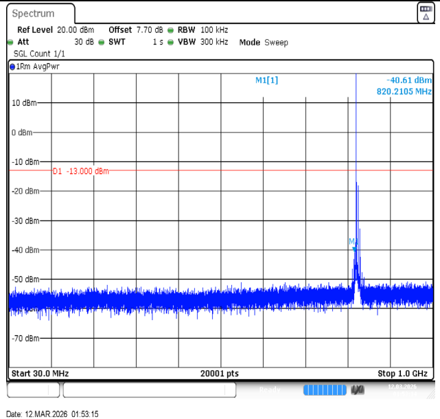
Band5-10MHz-QPSK-20450-1RB#0-30~1000-PASS
