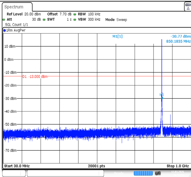
Band5-1.4MHz-QPSK-20643-6RB#0-30~1000-PASS
