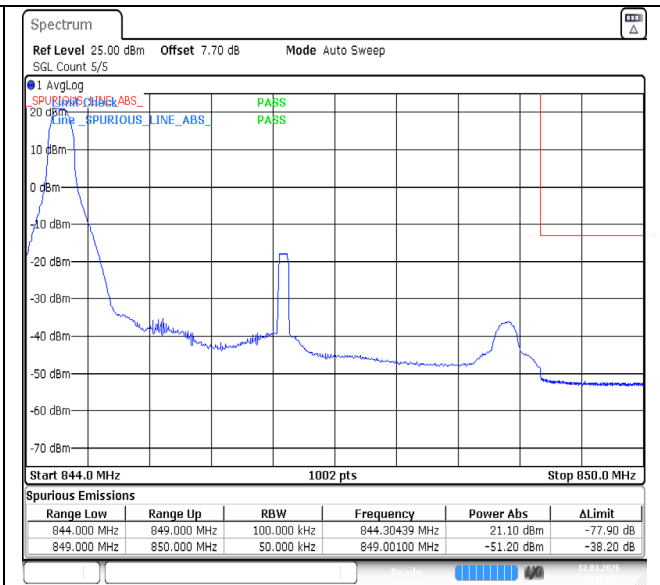
Band5-5MHz-QPSK-20625-1RB#0-PASS
