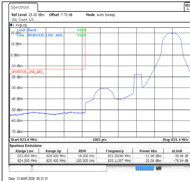
Band5-1.4MHz-64QAM-20407-1RB#5-PASS
