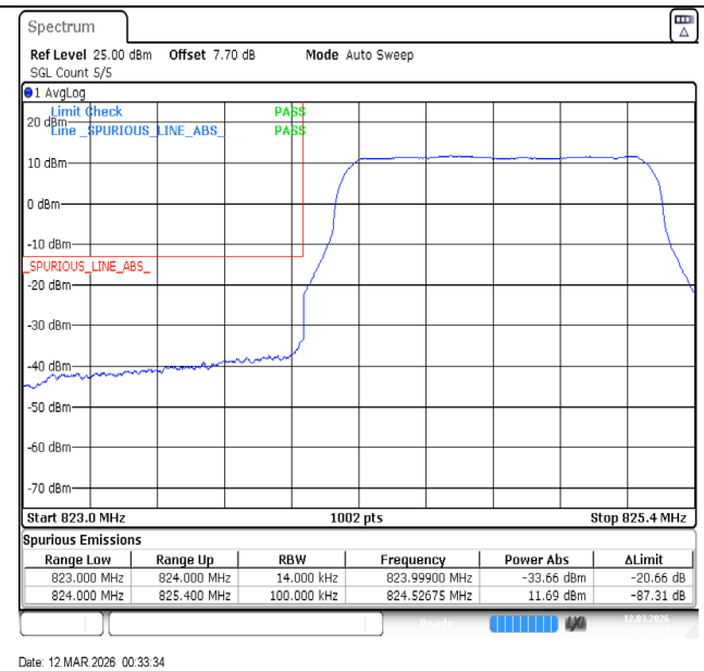
Band5-1.4MHz-64QAM-20407-6RB#0-PASS
