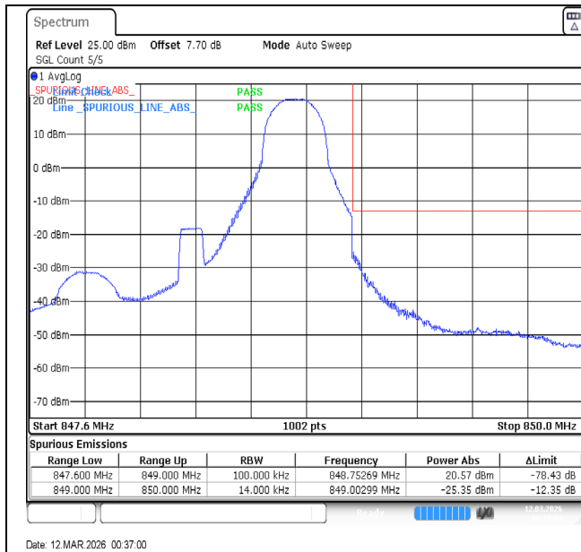
Band5-1.4MHz-16QAM-20643-1RB#5-PASS
