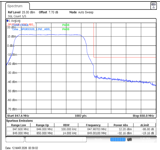
Band5-1.4MHz-16QAM-20643-6RB#0-PASS
