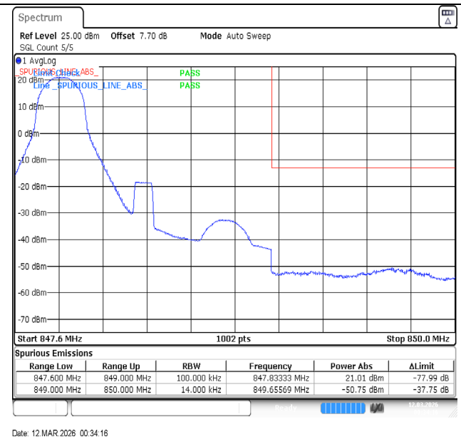
Band5-1.4MHz-QPSK-20643-1RB#0-PASS
