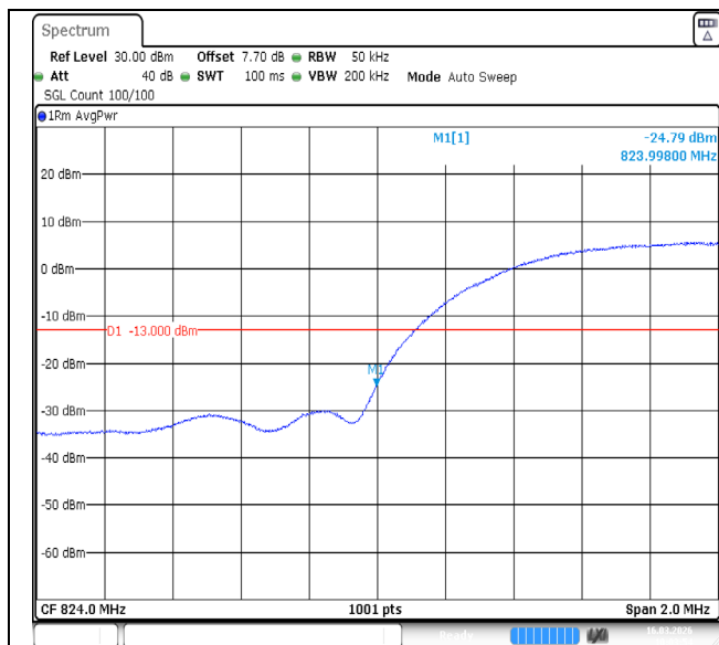
Band5-4132-PASS
