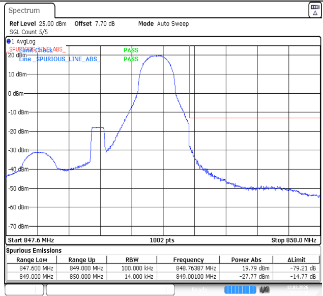
Band5-1.4MHz-64QAM-20643-1RB#5-PASS
