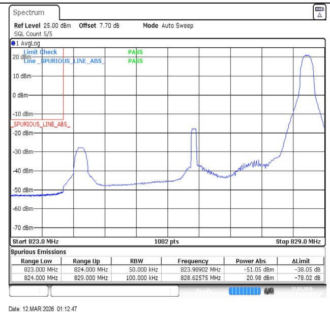
Band5-5MHz-QPSK-20425-1RB#24-PASS
