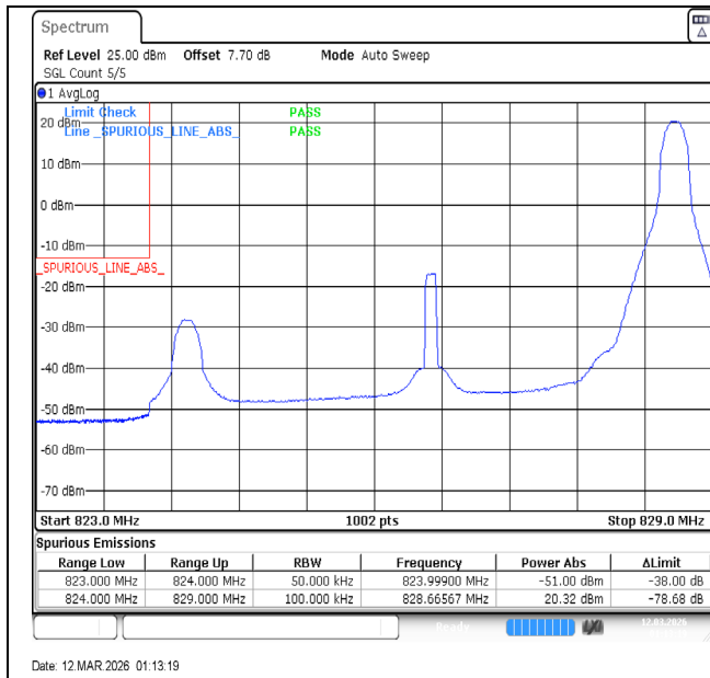
Band5-5MHz-64QAM-20425-1RB#24-PASS
