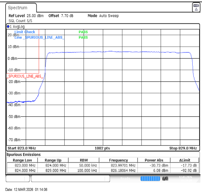
Band5-5MHz-64QAM-20425-25RB#0-PASS
