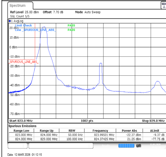
Band5-5MHz-16QAM-20425-1RB#0-PASS
