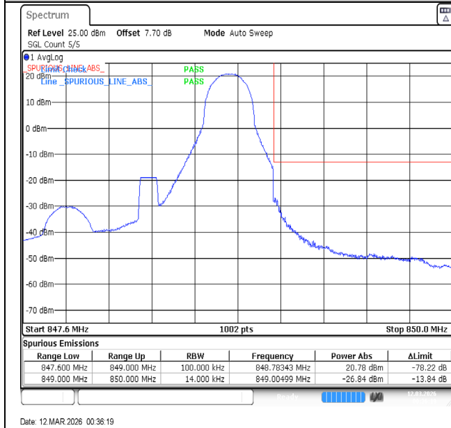
Band5-1.4MHz-QPSK-20643-1RB#5-PASS
