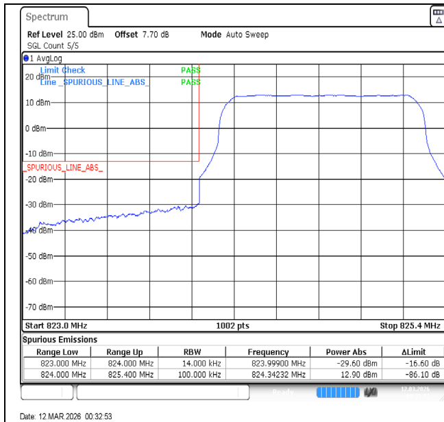
Band5-1.4MHz-16QAM-20407-6RB#0-PASS
