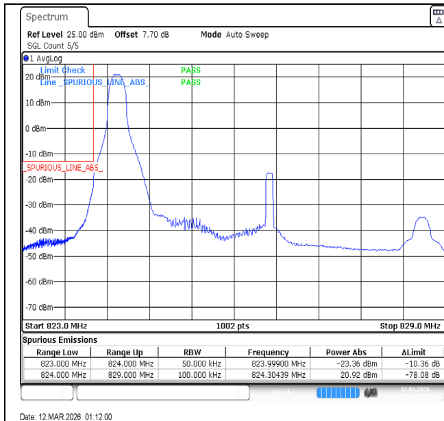
Band5-5MHz-QPSK-20425-1RB#0-PASS
