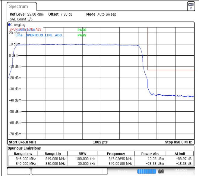
Band5-3MHz-QPSK-20635-1RB#0-PASS
