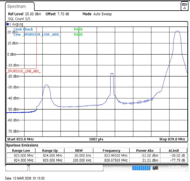
Band5-5MHz-16QAM-20425-1RB#24-PASS
