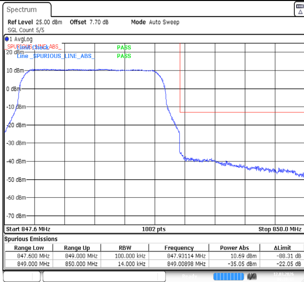
Band5-1.4MHz-64QAM-20643-1RB#0-PASS
