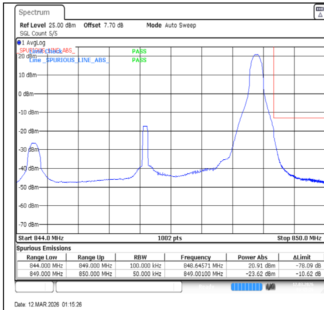
Band5-5MHz-16QAM-20625-1RB#24-PASS
