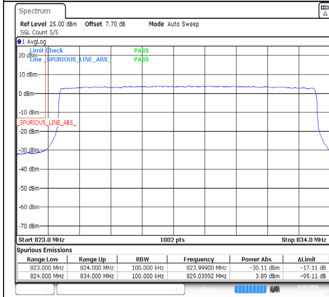
Band5-10MHz-16QAM-20450-1RB#0-PASS
