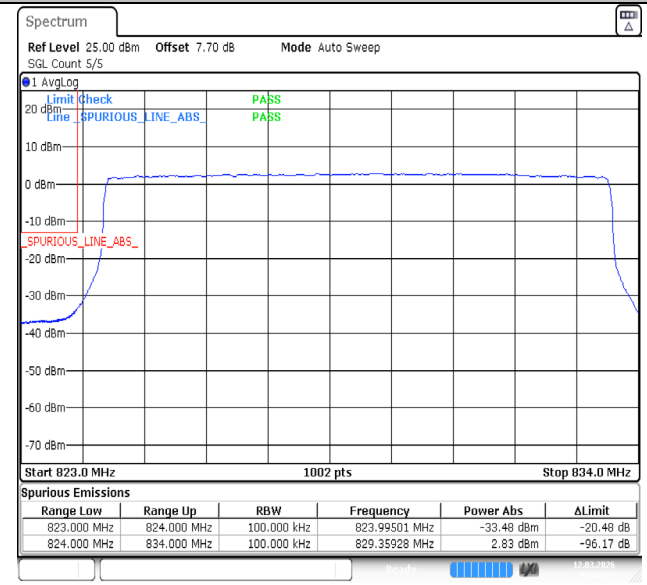
Band5-10MHz-64QAM-20450-1RB#0-PASS
