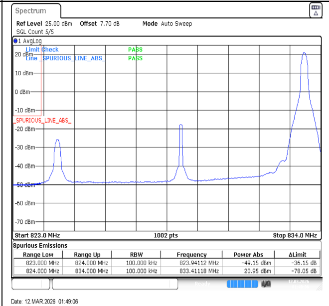
Band5-10MHz-QPSK-20450-1RB#49-PASS
