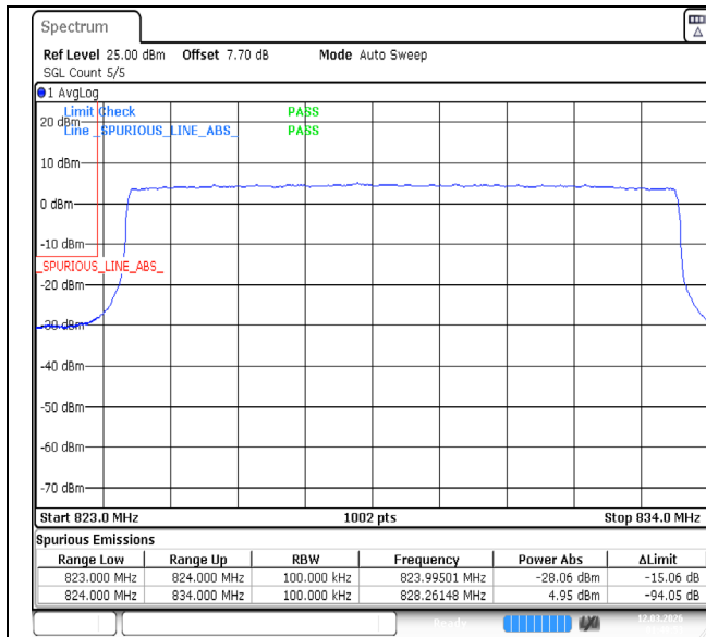
Band5-10MHz-QPSK-20450-50RB#0-PASS
