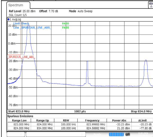
Band26(824-849)-5MHz-QPSK-27015-1RB#24-PASS
