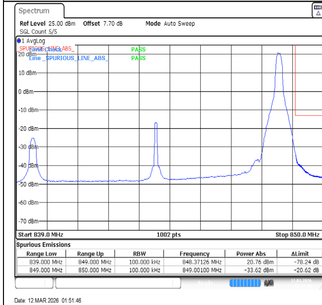
Band5-10MHz-16QAM-20600-1RB#49-PASS
