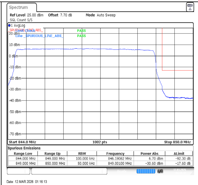
Band5-5MHz-16QAM-20625-25RB#0-PASS
