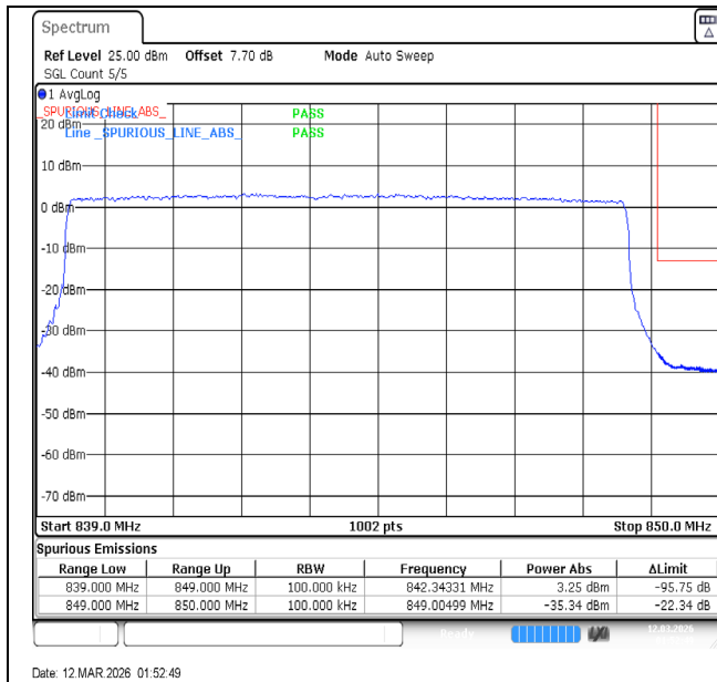
Band5-10MHz-64QAM-20600-50RB#0-PASS
