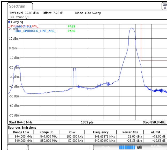
Band26(824-849)-5MHz-QPSK-27015-1RB#24-PASS
