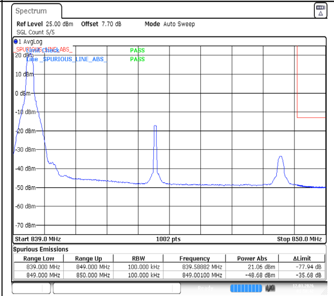
Band5-10MHz-16QAM-20450-1RB#49-PASS
