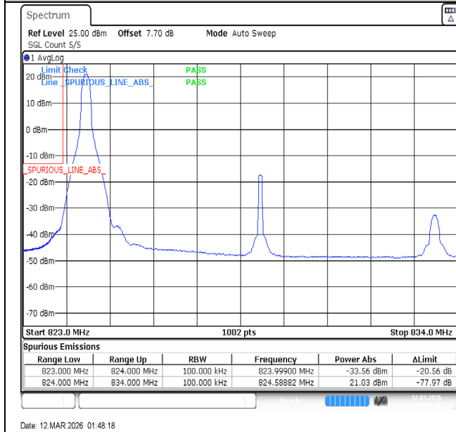
Band5-10MHz-QPSK-20450-1RB#0-PASS
