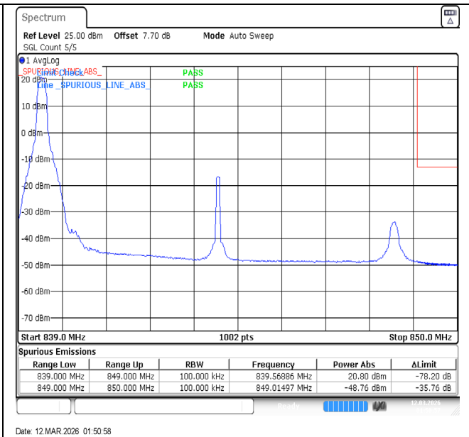
Band5-10MHz-16QAM-20600-1RB#0-PASS
