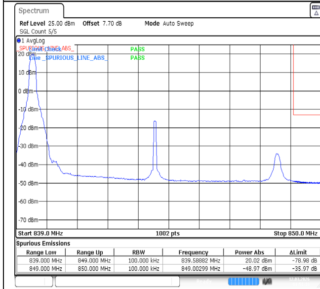
Band5-10MHz-QPSK-20600-1RB#49-PASS
