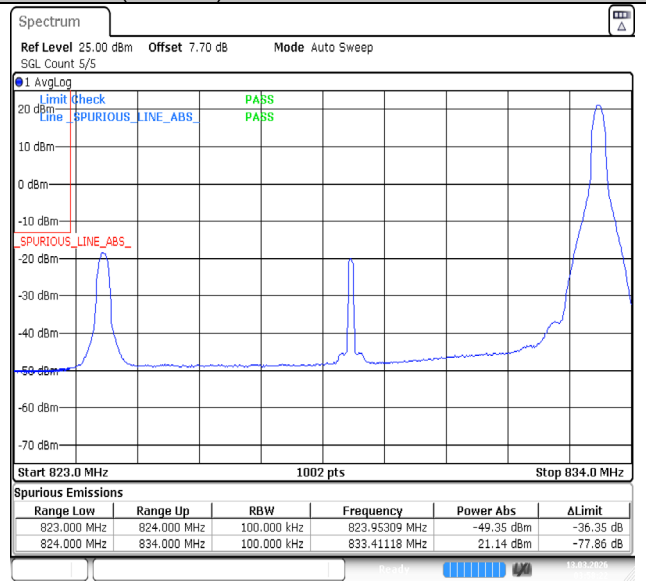
Band26(824-849)-5MHz-QPSK-27015-25RB#0-PASS
