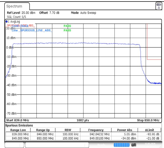
Band5-10MHz-QPSK-20600-50RB#0-PASS
