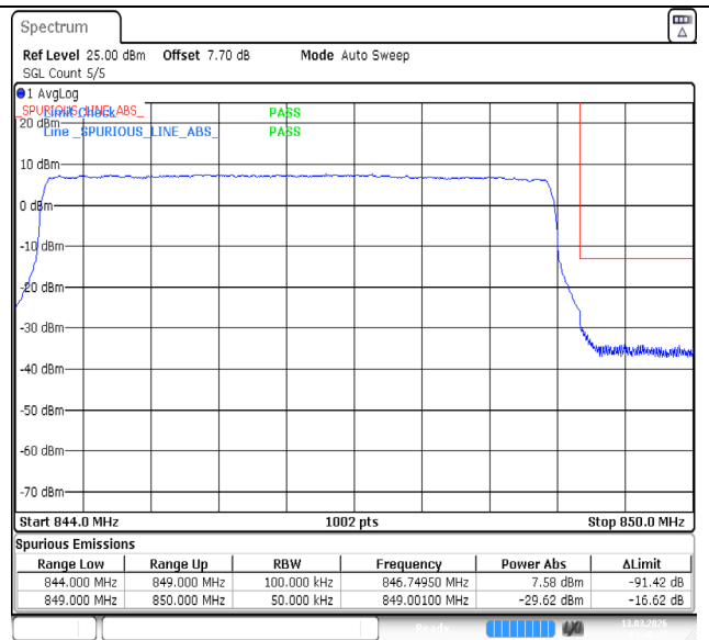
Band26(824-849)-5MHz-QPSK-27015-25RB#0-PASS
