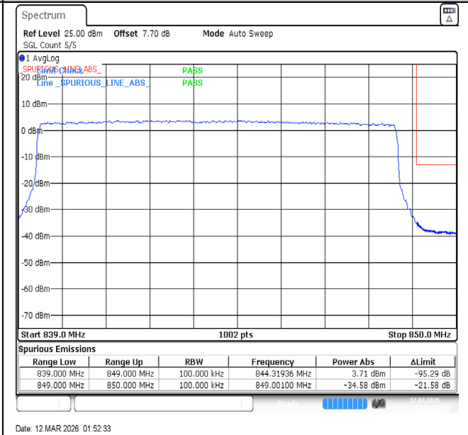
Band5-10MHz-16QAM-20600-50RB#0-PASS
