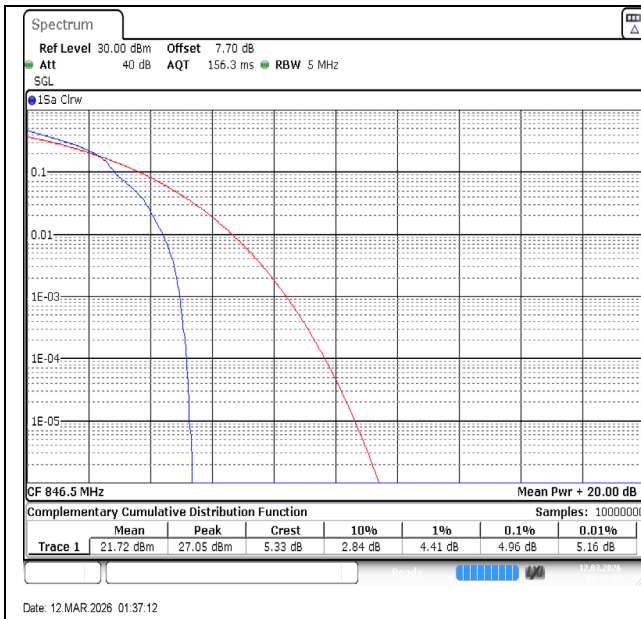
Band5-5MHz-16QAM-20625-1RB#0-PASS
