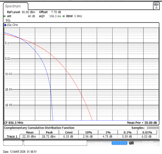
Band5-5MHz-16QAM-20525-25RB#0-PASS
