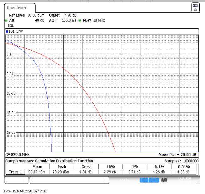
Band5-10MHz-QPSK-20450-50RB#0-PASS
