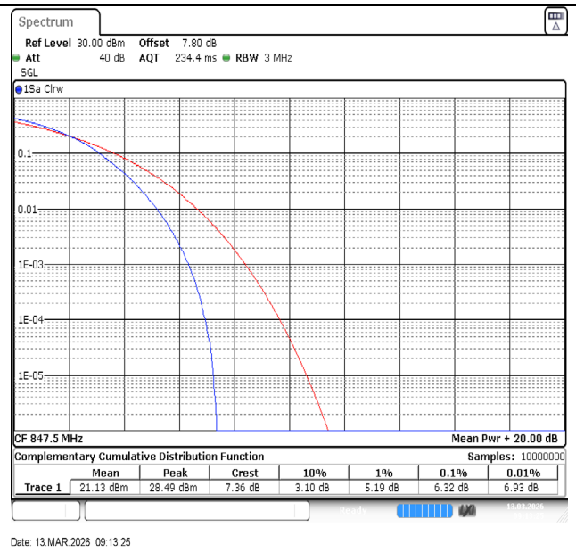
Band5-3MHz-64QAM-20635-15RB#0-PASS
