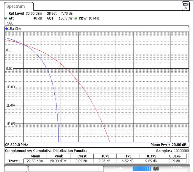
Band5-10MHz-64QAM-20450-50RB#0-PASS
