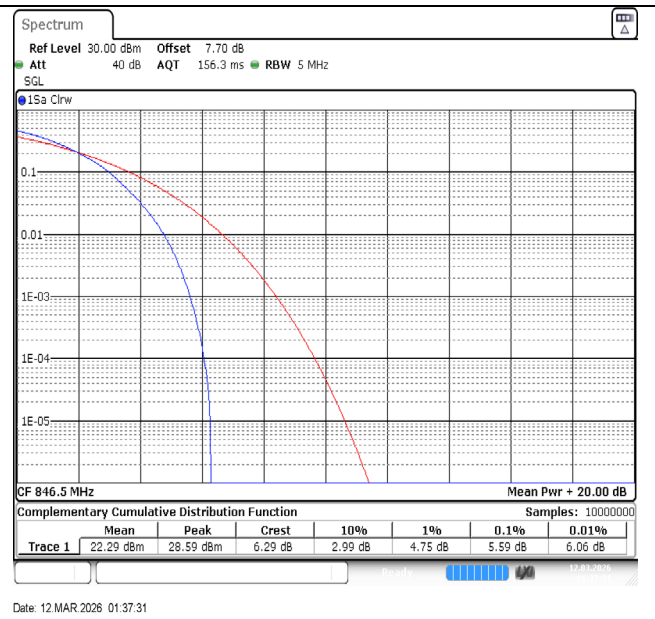
Band5-5MHz-16QAM-20625-25RB#0-PASS
