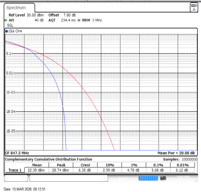
Band5-3MHz-16QAM-20635-15RB#0-PASS
