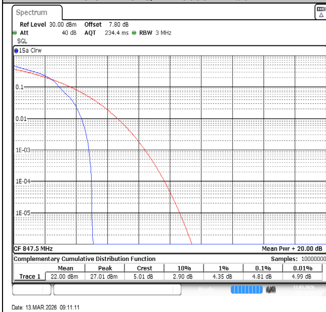
Band5-3MHz-16QAM-20635-1RB#0-PASS
