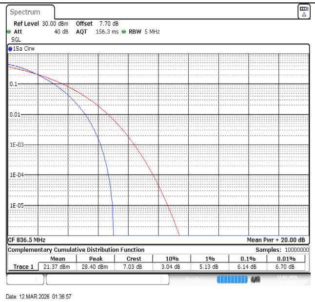
Band5-5MHz-64QAM-20525-25RB#0-PASS
