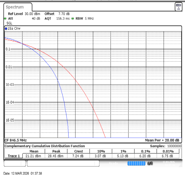
Band5-5MHz-64QAM-20625-25RB#0-PASS
