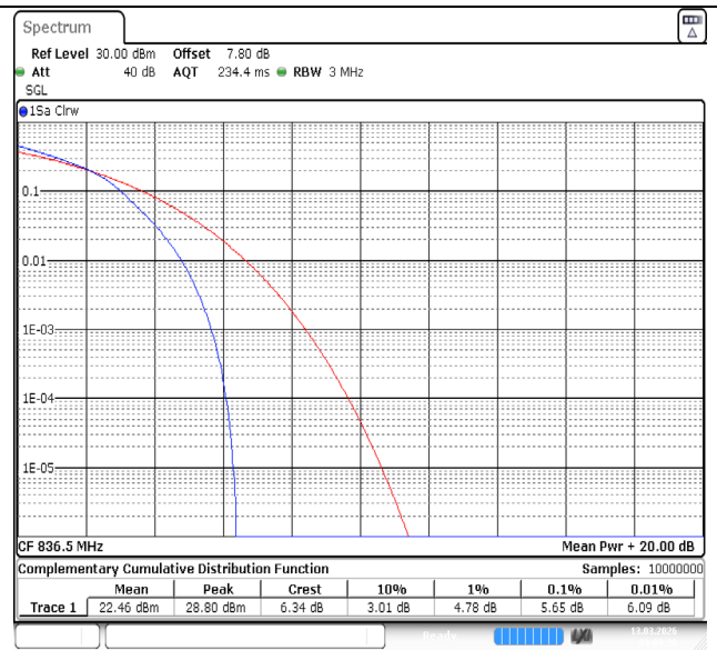
Band5-3MHz-16QAM-20525-15RB#0-PASS
