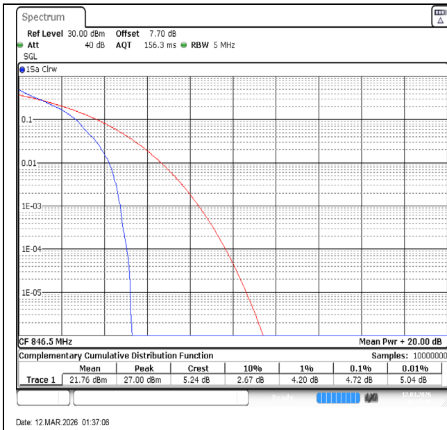
Band5-5MHz-QPSK-20625-1RB#0-PASS
