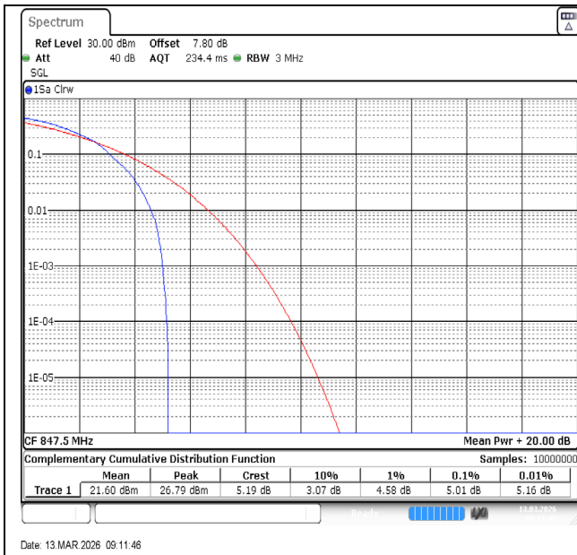
Band5-3MHz-64QAM-20635-1RB#0-PASS
