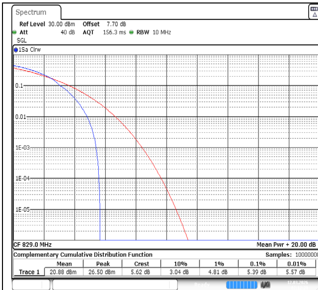
Band5-10MHz-64QAM-20450-1RB#0-PASS
