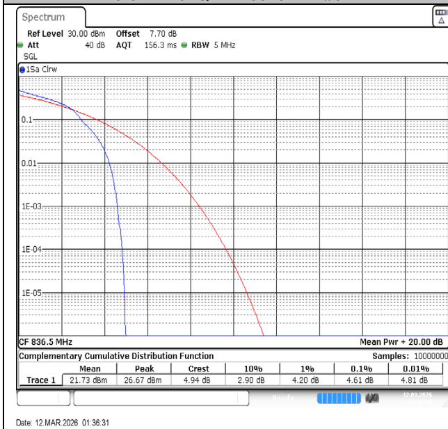
Band5-5MHz-16QAM-20525-1RB#0-PASS
