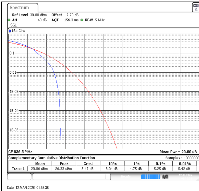
Band5-5MHz-64QAM-20525-1RB#0-PASS
