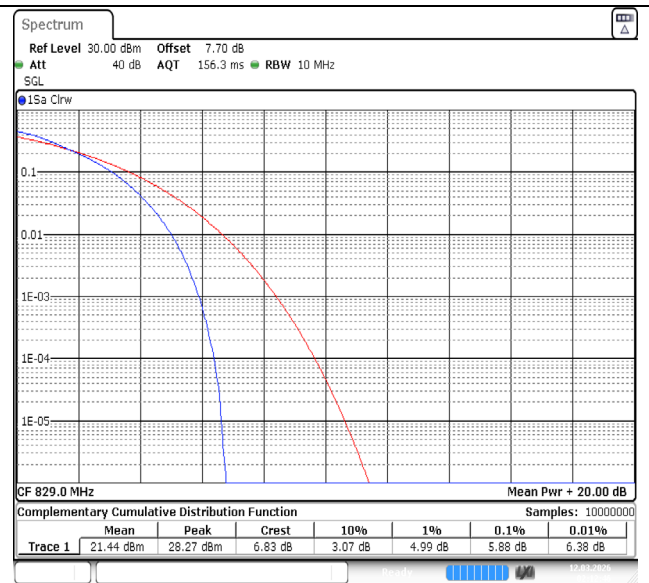
Band5-10MHz-64QAM-20450-50RB#0-PASS
