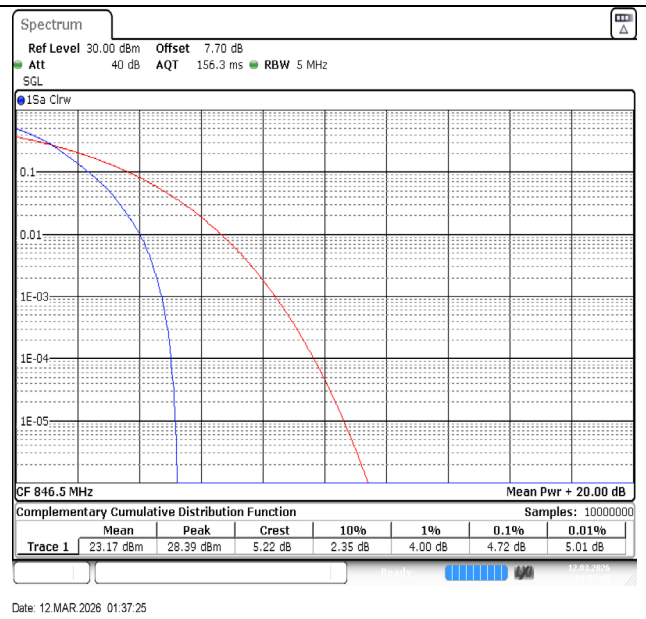
Band5-5MHz-QPSK-20625-25RB#0-PASS
