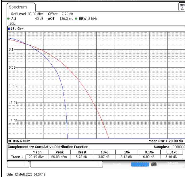
Band5-5MHz-64QAM-20625-1RB#0-PASS
