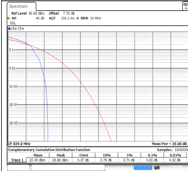
Band5-10MHz-64QAM-20450-1RB#0-PASS
