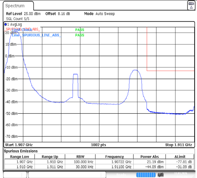
Band2-3MHz-QPSK-19185-1RB#0-PASS
