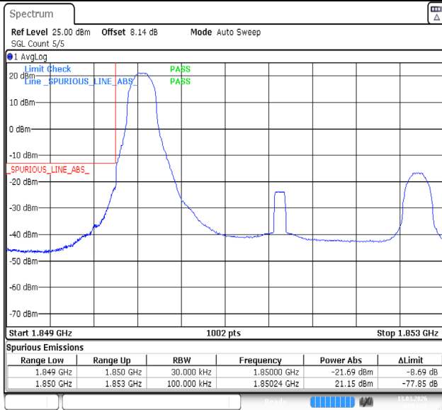
Band2-1.4MHz-16QAM-19193-1RB#5-PASS
