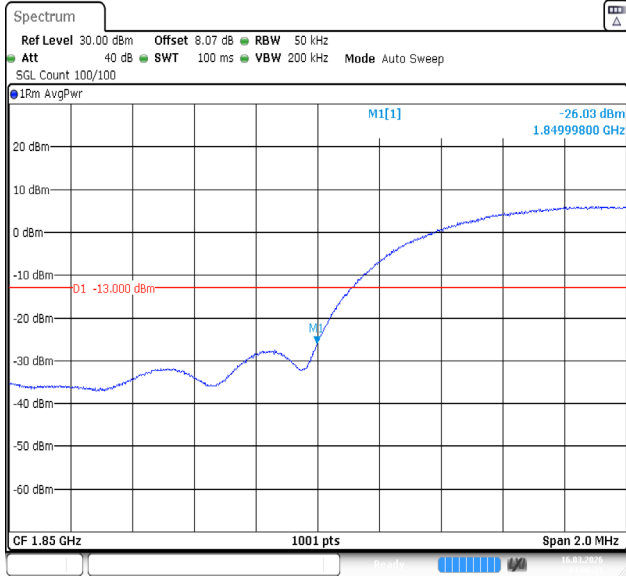
Band2-9262-PASS
