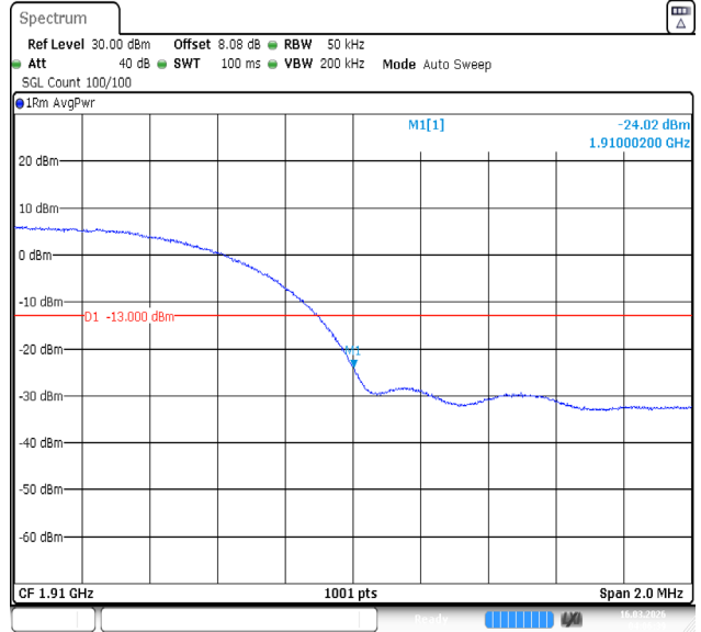
Band2-9538-PASS
