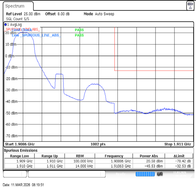
Band2-1.4MHz-16QAM-19193-1RB#0-PASS
