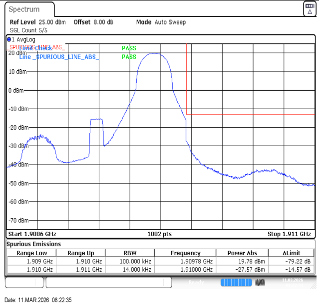
Band2-1.4MHz-64QAM-19193-1RB#5-PASS
