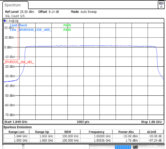
Band2-10MHz-64QAM-18650-1RB#0-PASS
