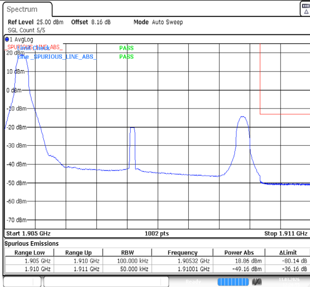
Band2-5MHz-64QAM-19175-1RB#0-PASS
