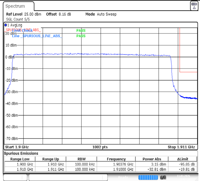
Band2-10MHz-16QAM-19150-1RB#0-PASS
