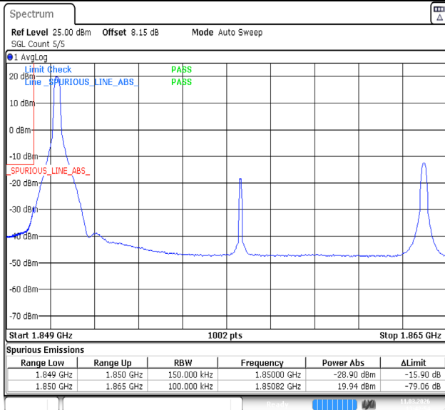
Band2-15MHz-64QAM-18675-1RB#74-PASS
