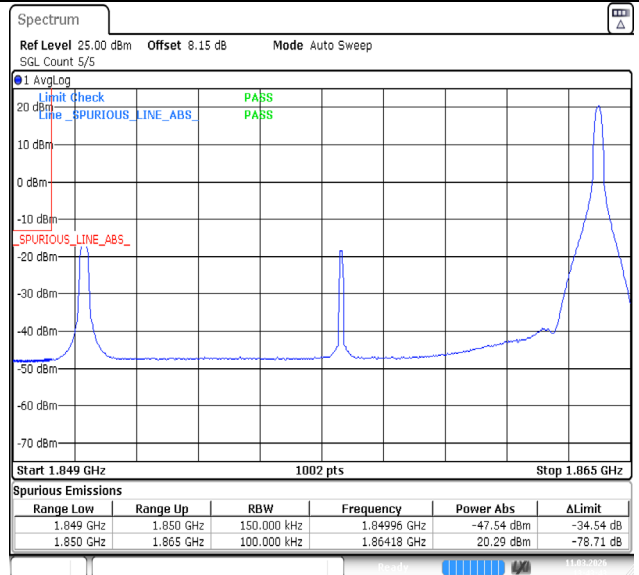
Band2-15MHz-16QAM-18675-1RB#74-PASS
