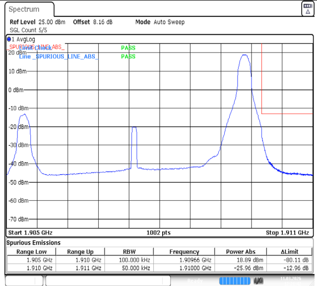
Band2-5MHz-64QAM-19175-1RB#24-PASS
