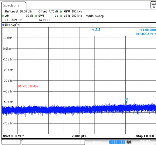
Band38-5MHz-QPSK-37775-1RB#0-30~1000-PASS
