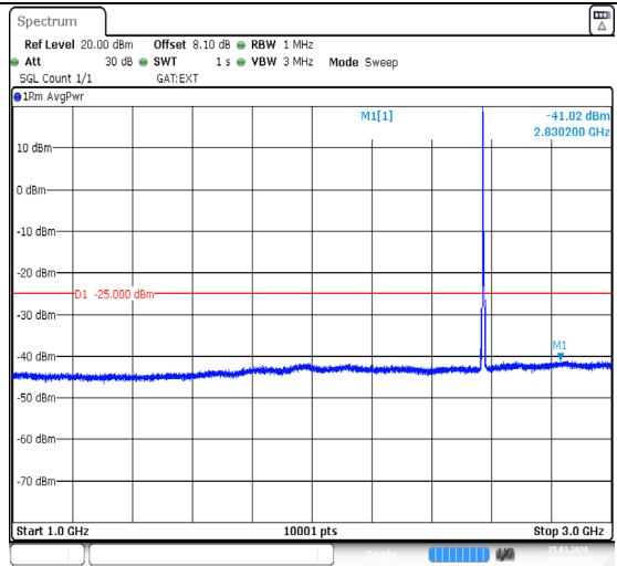
Band38-5MHz-QPSK-37775-1RB#0-1000~3000-PASS
