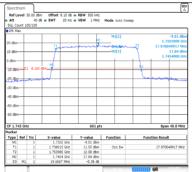
Band4-20MHz-16QAM-20300-100RB#0-PASS
