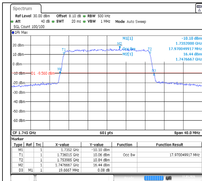
Band4-20MHz-64QAM-20300-100RB#0-PASS
