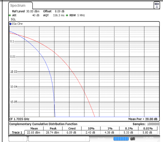
Band4-5MHz-QPSK-20175-25RB#0-PASS
