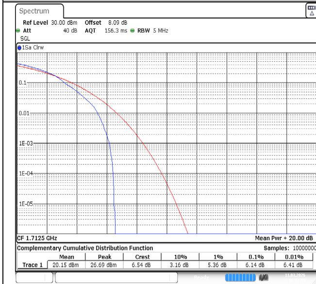
Band4-5MHz-QPSK-19975-1RB#0-PASS
