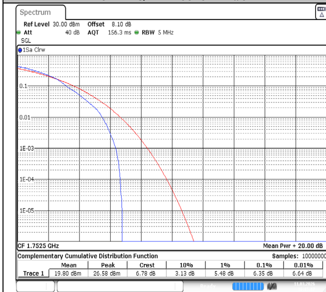
Band4-5MHz-QPSK-20375-1RB#0-PASS
