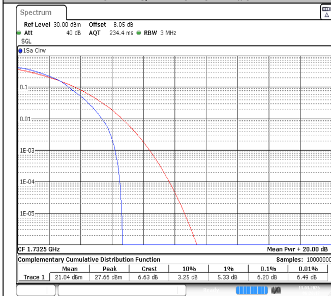
Band4-3MHz-QPSK-20175-1RB#0-PASS
