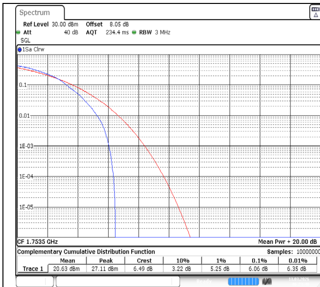
Band4-3MHz-64QAM-20385-1RB#0-PASS
