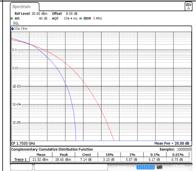
Band4-3MHz-16QAM-20385-15RB#0-PASS
