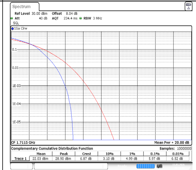
Band4-3MHz-16QAM-19965-15RB#0-PASS
