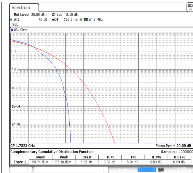
Band4-5MHz-16QAM-20375-1RB#0-PASS
