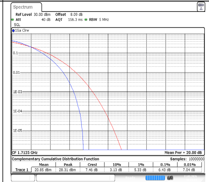
Band4-5MHz-64QAM-19975-25RB#0-PASS
