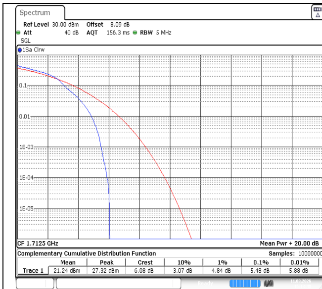
Band4-5MHz-16QAM-19975-1RB#0-PASS
