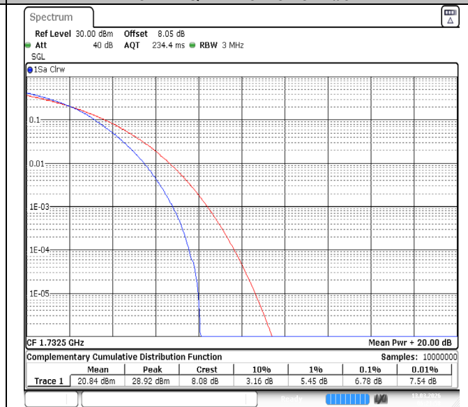
Band4-3MHz-64QAM-20175-15RB#0-PASS
