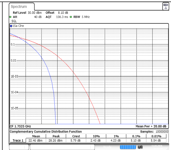
Band4-5MHz-QPSK-20375-25RB#0-PASS
