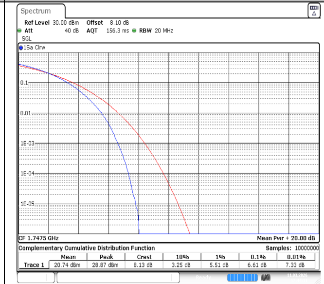
Band4-15MHz-64QAM-20325-75RB#0-PASS
