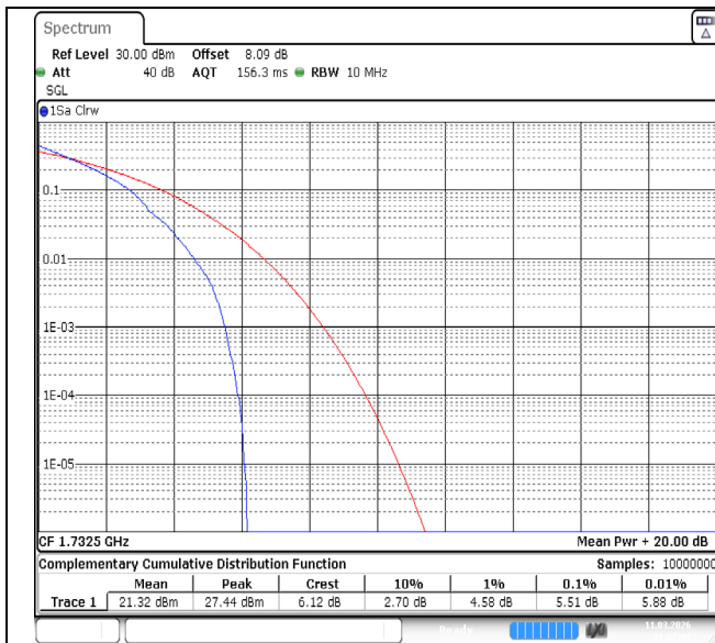
Band4-10MHz-QPSK-20175-1RB#0-PASS
