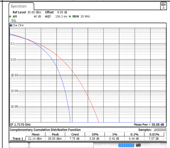
Band4-15MHz-64QAM-20025-75RB#0-PASS
