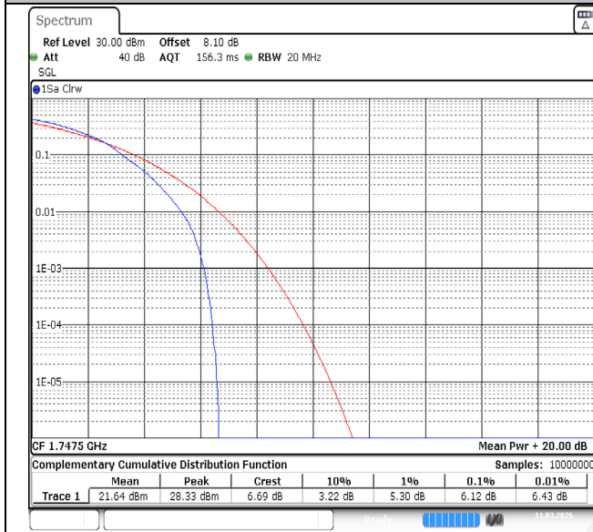
Band4-15MHz-QPSK-20325-1RB#0-PASS
