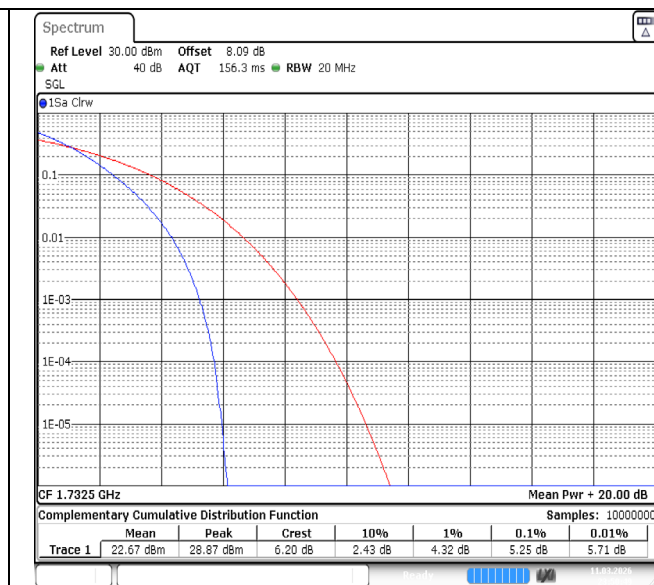
Band4-20MHz-QPSK-20175-100RB#0-PASS
