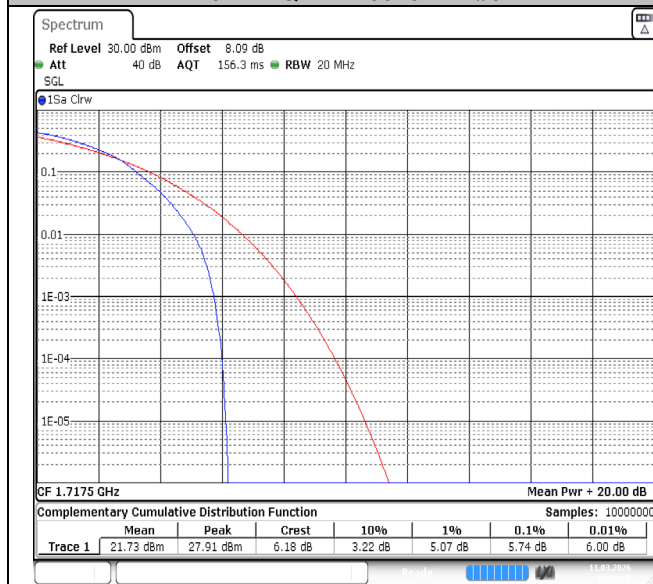
Band4-15MHz-QPSK-20025-1RB#0-PASS
