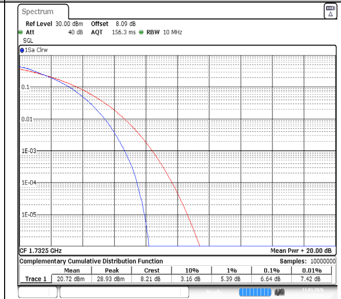
Band4-10MHz-64QAM-20175-50RB#0-PASS
