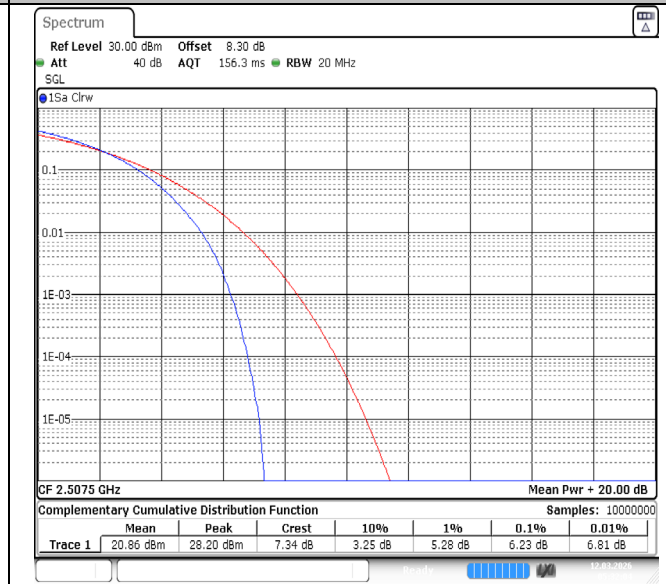
Band7-15MHz-64QAM-20825-75RB#0-PASS
