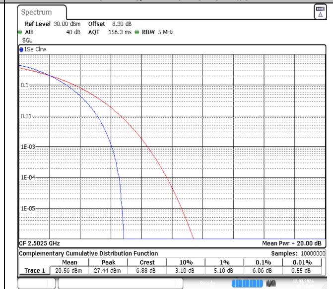
Band7-5MHz-64QAM-20775-25RB#0-PASS
