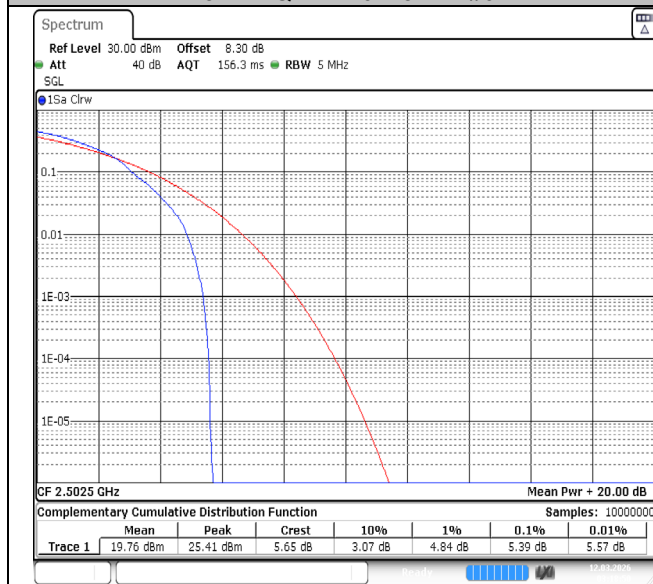
Band7-5MHz-QPSK-20775-1RB#0-PASS
