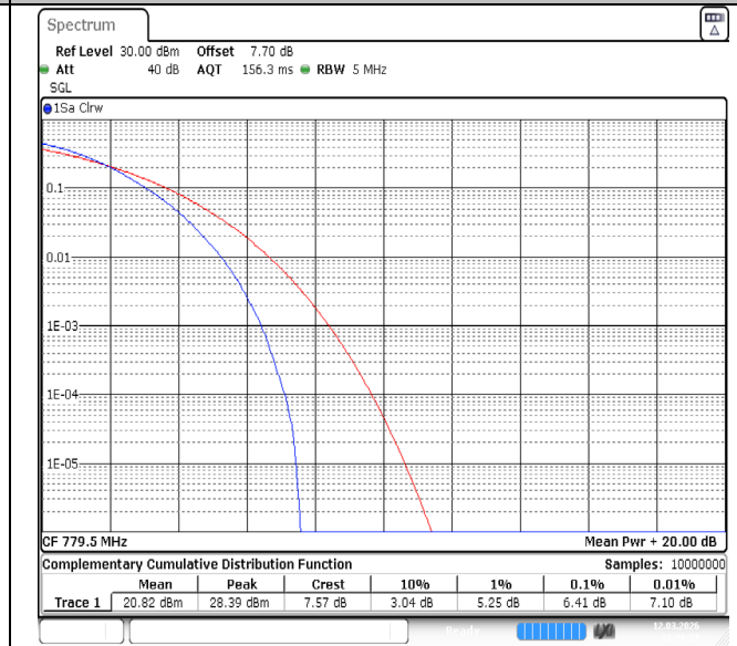
Band13-5MHz-64QAM-23205-25RB#0-PASS
