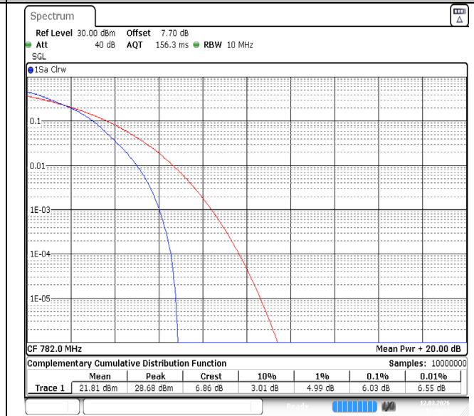
Band13-10MHz-16QAM-23230-50RB#0-PASS
