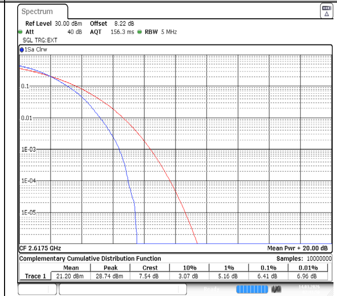
Band38-5MHz-64QAM-38225-25RB#0-PASS
