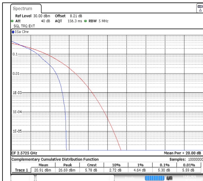
Band38-5MHz-QPSK-37775-1RB#0-PASS
