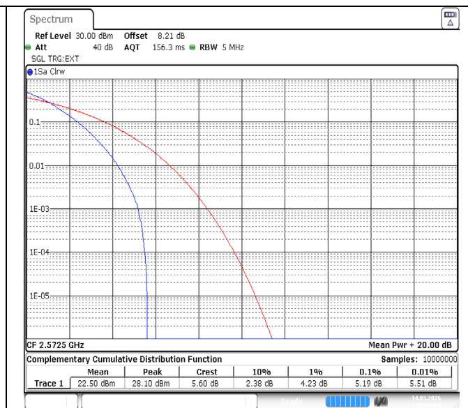
Band38-5MHz-QPSK-37775-25RB#0-PASS
