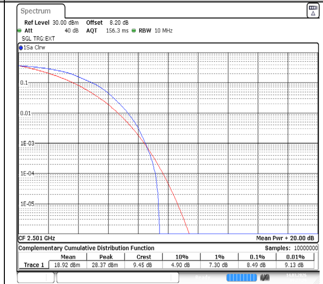
Band41-10MHz-16QAM-39700-50RB#0-PASS
