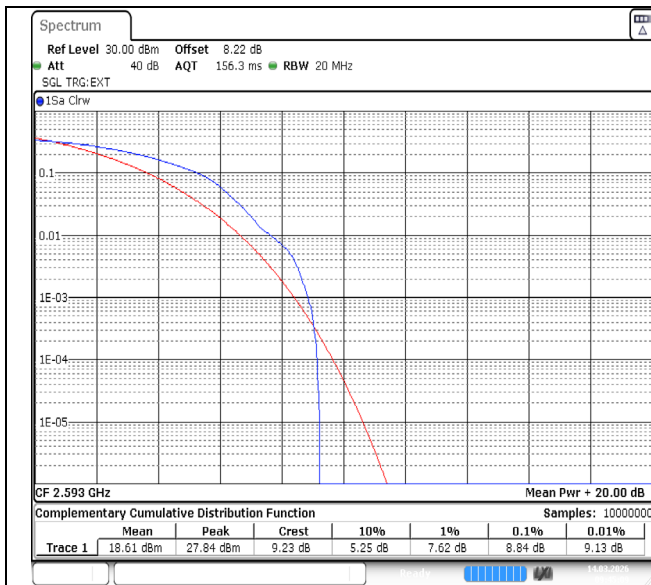
Band41-15MHz-64QAM-40620-1RB#0-PASS
