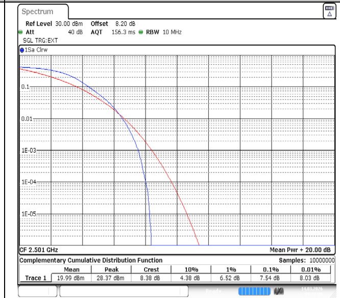
Band41-10MHz-QPSK-39700-50RB#0-PASS
