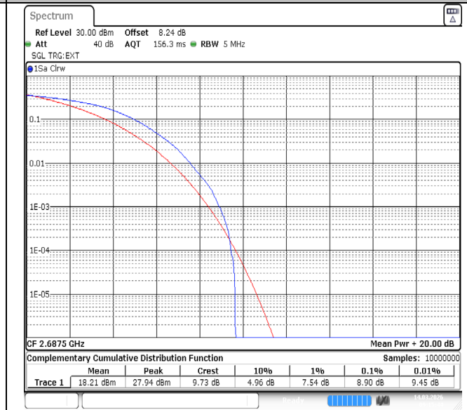
Band41-5MHz-QPSK-41565-25RB#0-PASS
