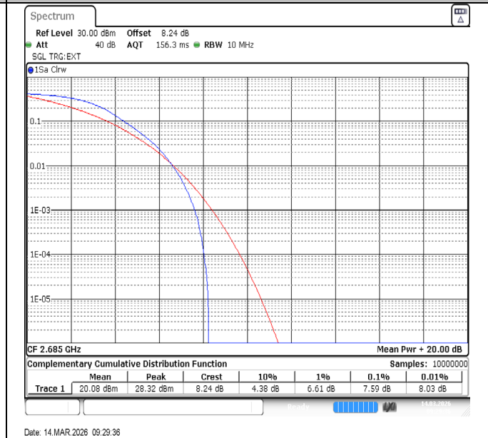
Band41-10MHz-QPSK-41540-50RB#0-PASS
