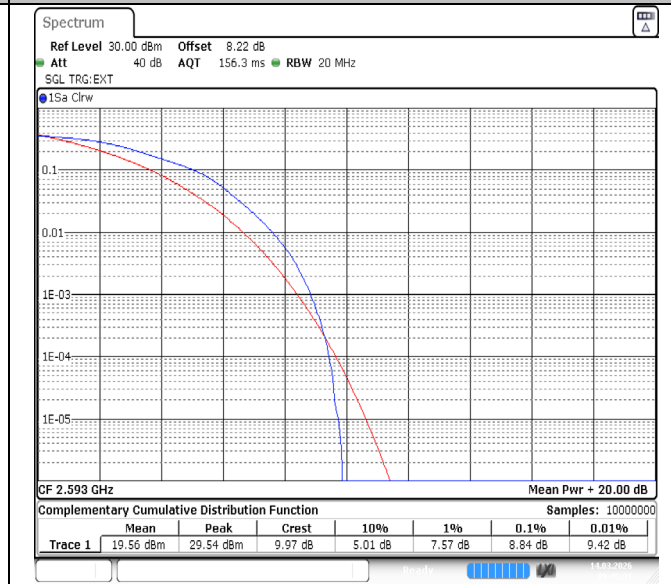
Band41-15MHz-16QAM-40620-75RB#0-PASS
