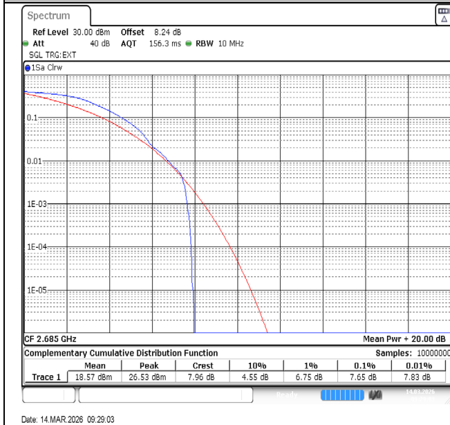
Band41-10MHz-QPSK-41540-1RB#0-PASS
