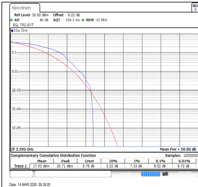
Band41-10MHz-16QAM-40620-1RB#0-PASS
