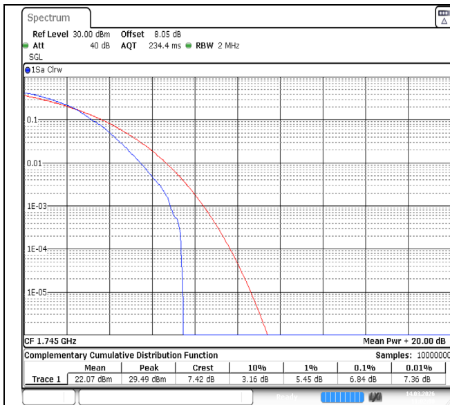
Band66-1.4MHz-64QAM-132322-1RB#0-PASS
