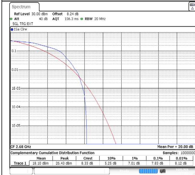
Band41-20MHz-64QAM-41490-1RB#0-PASS
