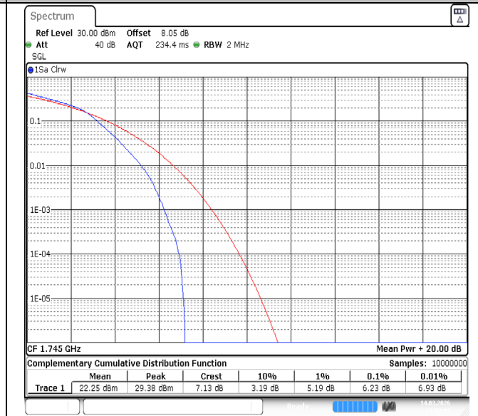
Band66-1.4MHz-64QAM-132322-6RB#0-PASS
