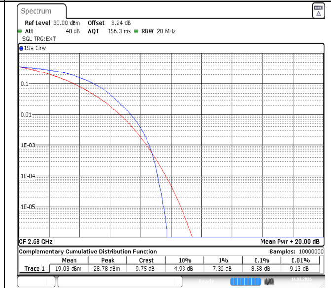
Band41-20MHz-16QAM-41490-100RB#0-PASS
