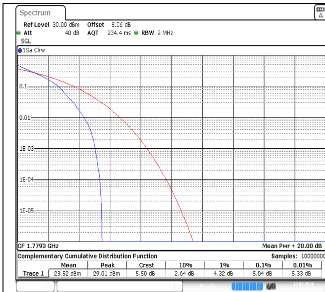
Band66-1.4MHz-QPSK-132665-1RB#0-PASS
