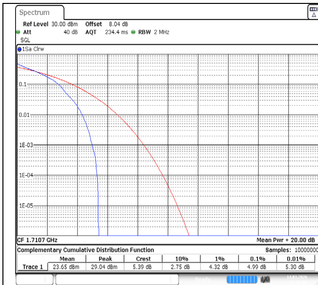
Band66-1.4MHz-QPSK-131979-1RB#0-PASS
