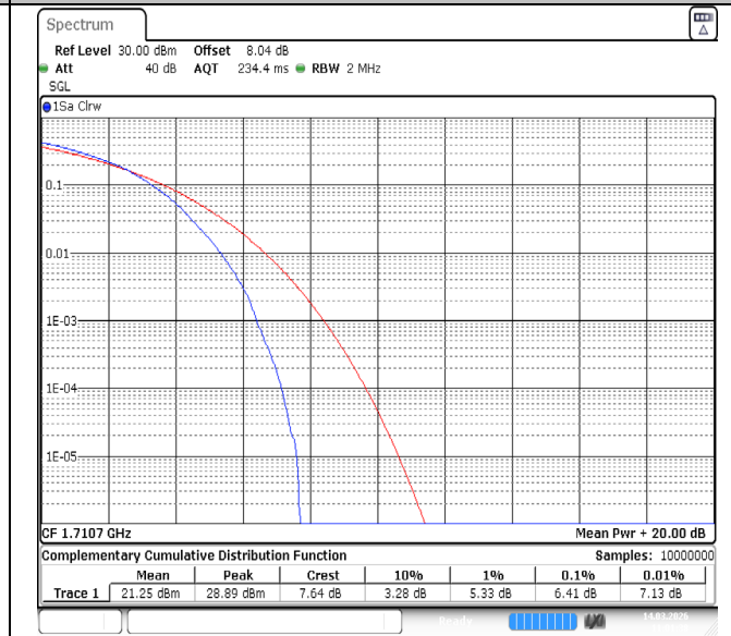
Band66-1.4MHz-64QAM-131979-6RB#0-PASS
