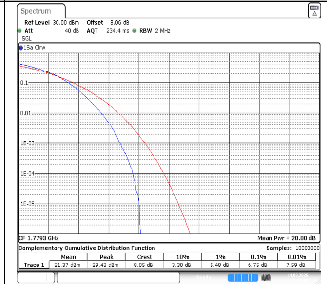
Band66-1.4MHz-64QAM-132665-6RB#0-PASS
