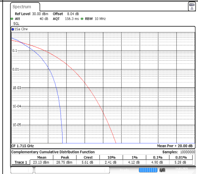
Band66-10MHz-QPSK-132022-50RB#0-PASS
