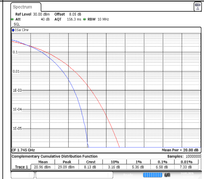
Band66-10MHz-64QAM-132322-50RB#0-PASS
