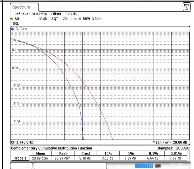
Band66-3MHz-64QAM-132322-15RB#0-PASS
