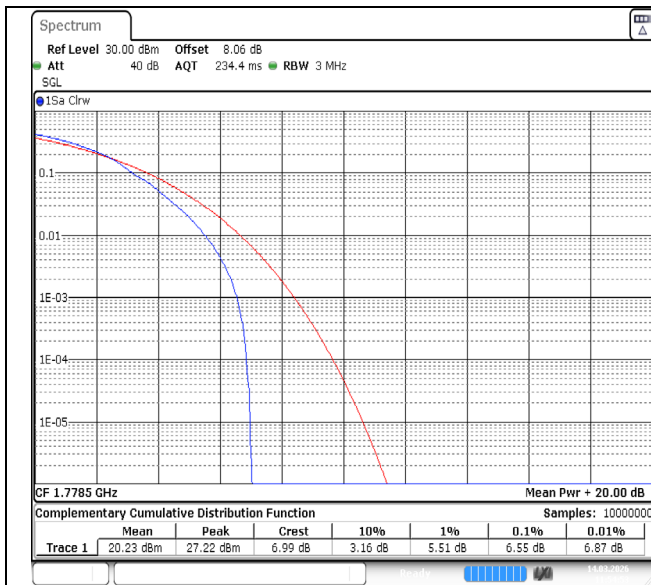
Band66-3MHz-64QAM-132657-1RB#0-PASS
