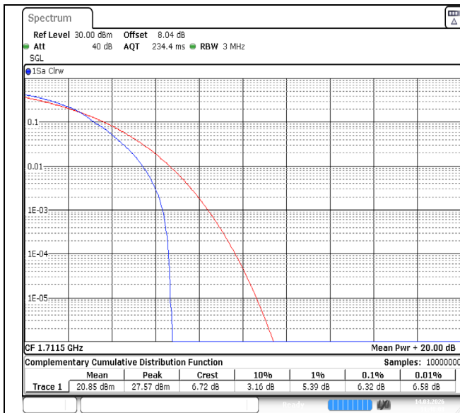
Band66-3MHz-64QAM-131987-1RB#0-PASS
