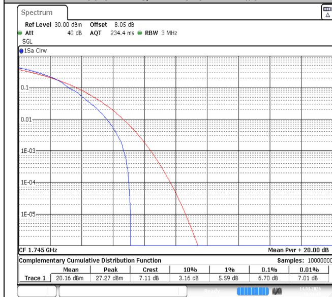
Band66-3MHz-QPSK-132322-1RB#0-PASS
