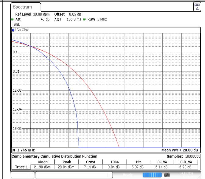
Band66-5MHz-16QAM-132322-25RB#0-PASS
