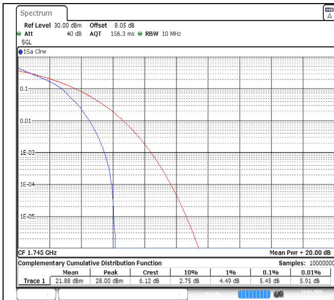
Band66-10MHz-QPSK-132322-1RB#0-PASS
