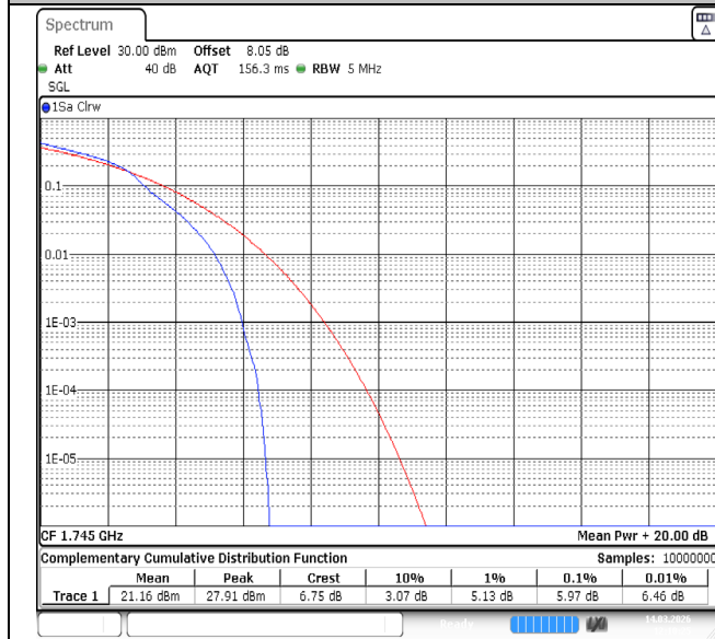
Band66-5MHz-64QAM-132322-1RB#0-PASS
