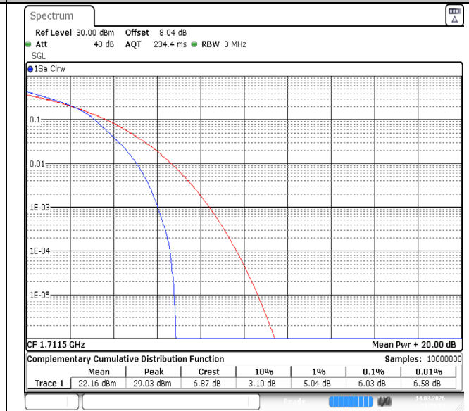
Band66-3MHz-16QAM-131987-15RB#0-PASS
