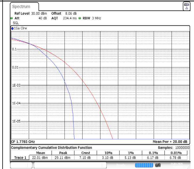
Band66-3MHz-16QAM-132657-15RB#0-PASS
