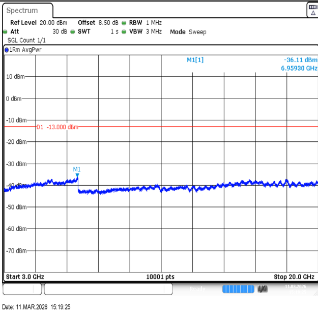
Band4-1.4MHz-QPSK-20393-6RB#0-3000~20000-PASS
