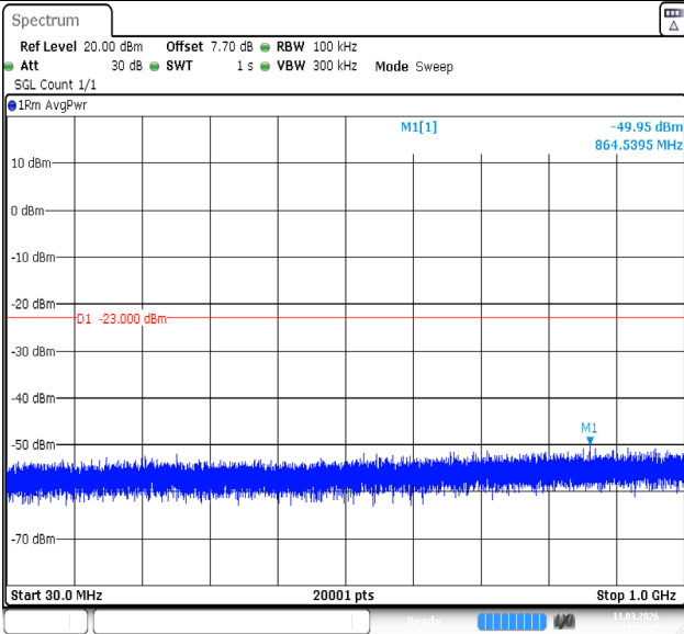
Band4-1.4MHz-QPSK-20175-1RB#5-30~1000-PASS
