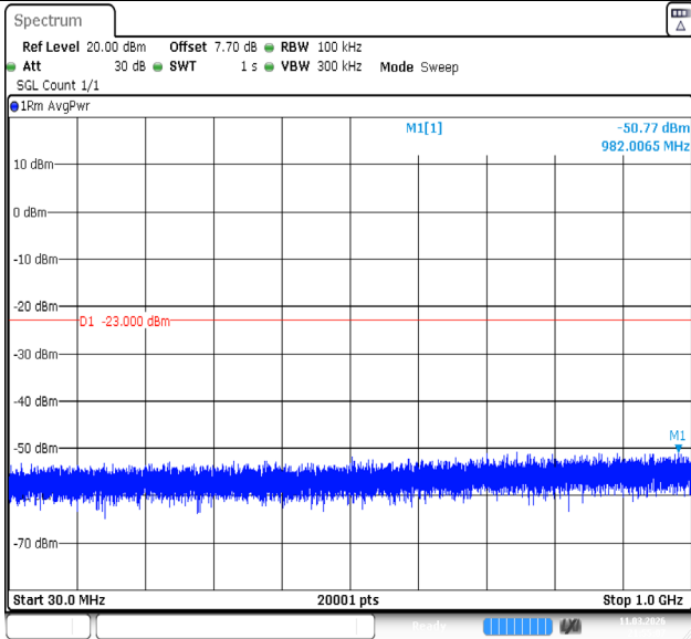
Band4-20MHz-QPSK-20175-1RB#0-30~1000-PASS
