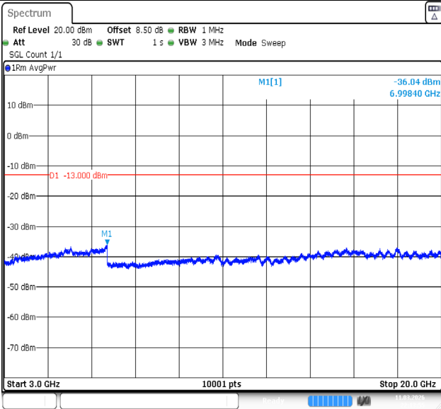
Band4-20MHz-QPSK-20175-100RB#0-3000~20000-PASS
