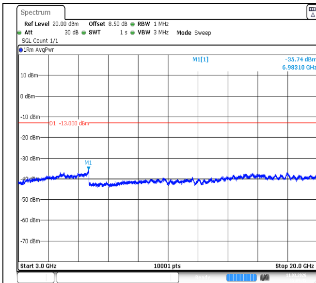
Band4-1.4MHz-QPSK-19957-6RB#0-3000~20000-PASS
