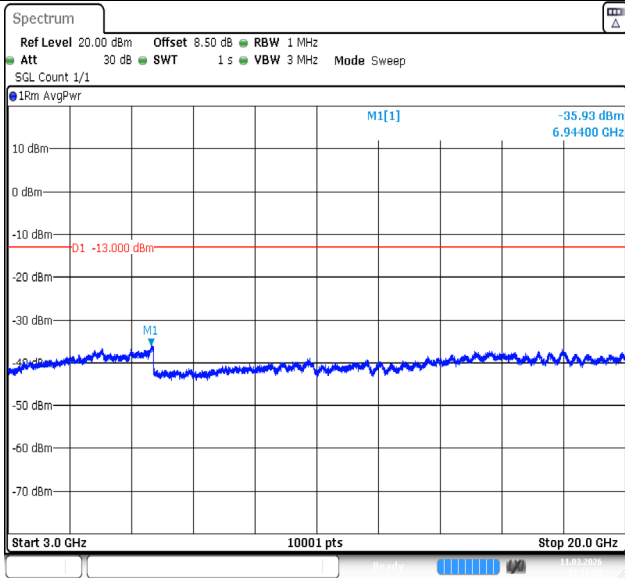
Band4-1.4MHz-QPSK-20393-1RB#0-3000~20000-PASS
