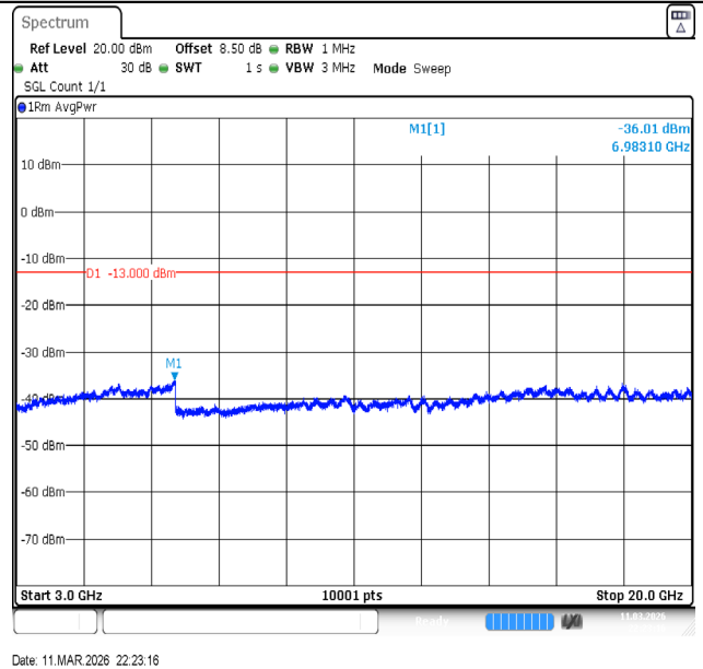
Band4-20MHz-QPSK-20300-1RB#0-3000~20000-PASS
