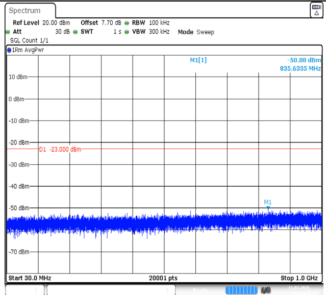
Band4-1.4MHz-QPSK-20175-6RB#0-30~1000-PASS
