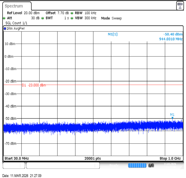
Band4-20MHz-QPSK-20050-1RB#0-30~1000-PASS
