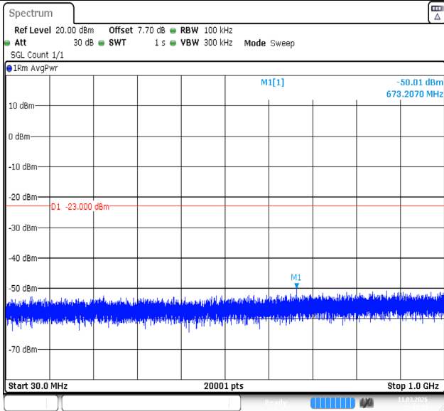
Band4-1.4MHz-QPSK-20393-6RB#0-30~1000-PASS
