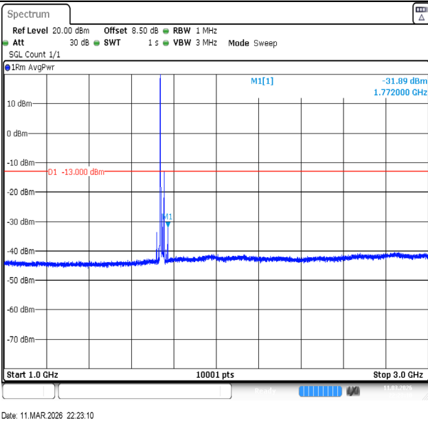
Band4-20MHz-QPSK-20300-1RB#0-1000~3000-PASS
