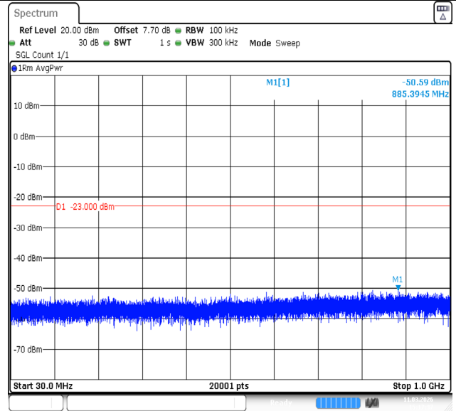
Band4-1.4MHz-QPSK-20393-1RB#5-30~1000-PASS
