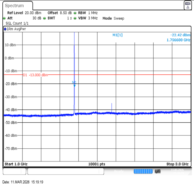
Band4-1.4MHz-QPSK-20393-6RB#0-1000~3000-PASS
