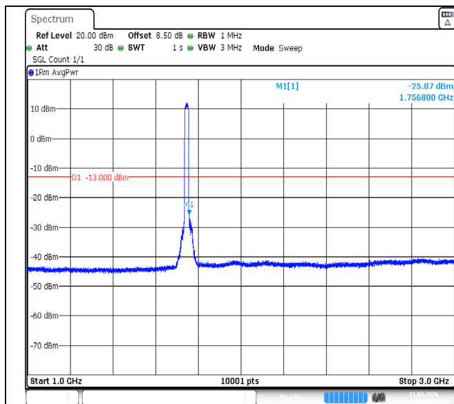
Band4-20MHz-QPSK-20300-100RB#0-1000~3000-PASS
