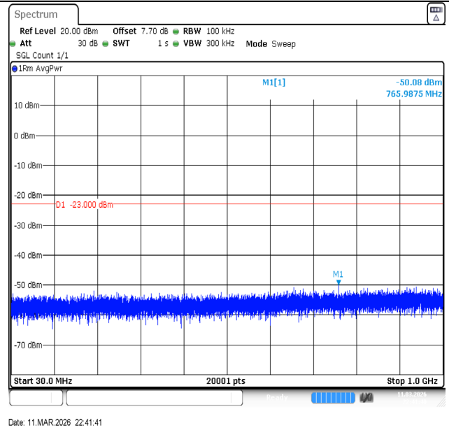
Band4-20MHz-QPSK-20300-100RB#0-30~1000-PASS
