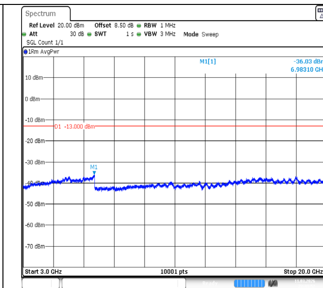
Band4-20MHz-QPSK-20300-100RB#0-3000~20000-PASS
