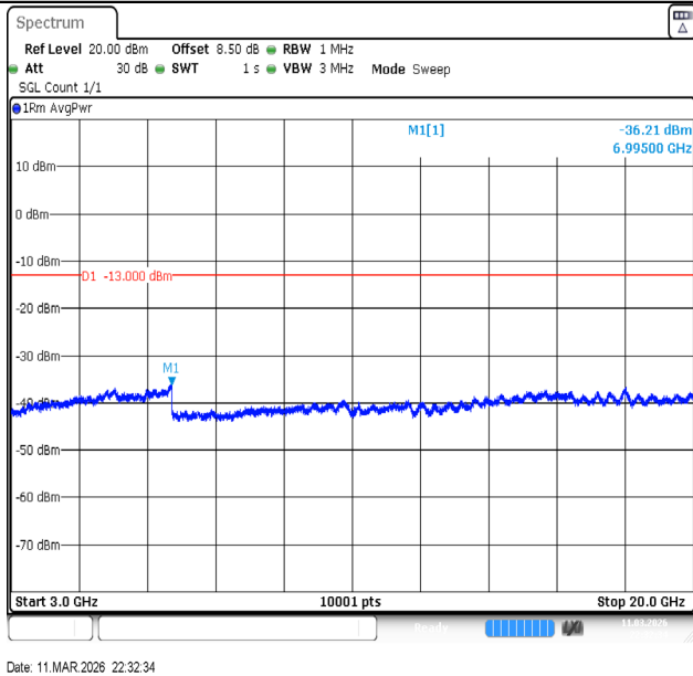
Band4-20MHz-QPSK-20300-1RB#99-3000~20000-PASS
