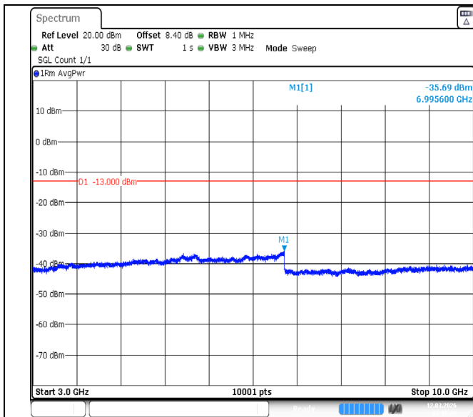
Band13-5MHz-QPSK-23255-1RB#0-3000~10000-PASS
