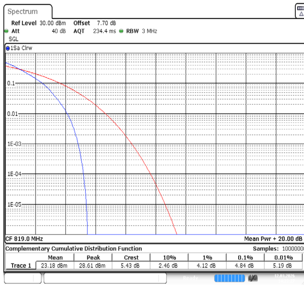
Band26(814-824)-3MHz-QPSK-26740-15RB#0-PASS
