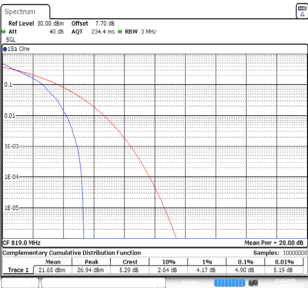
Band26(814-824)-3MHz-QPSK-26740-1RB#0-PASS
