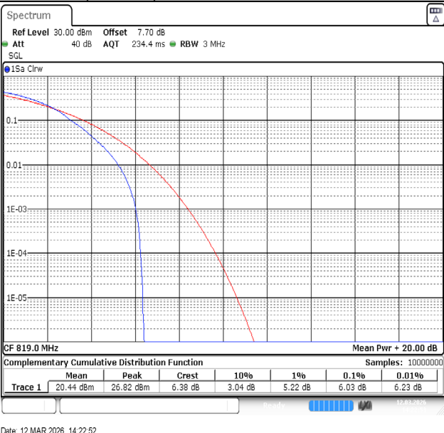
Band26(814-824)-3MHz-64QAM-26740-1RB#0-PASS
