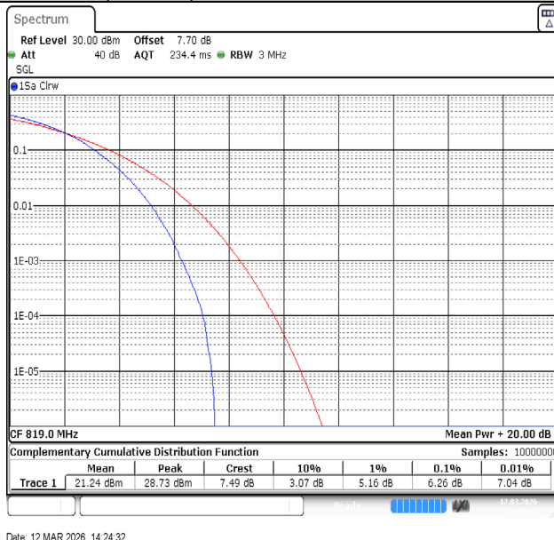
Band26(814-824)-3MHz-64QAM-26740-15RB#0-PASS
