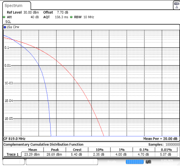
Band26(814-824)-5MHz-16QAM-26765-25RB#0-PASS
