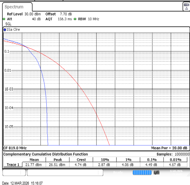
Band26(814-824)-10MHz-16QAM-26740-1RB#0-PASS
