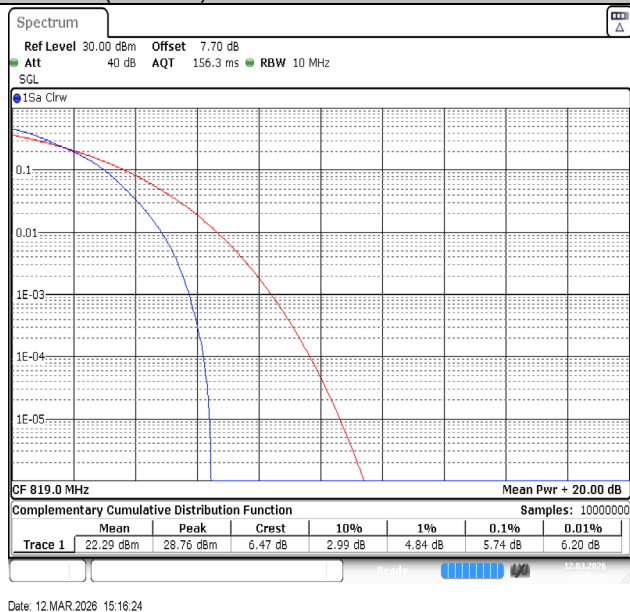
Band26(814-824)-10MHz-16QAM-26740-50RB#0-PASS
