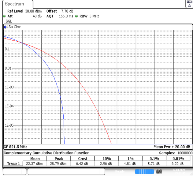
Band26(814-824)-5MHz-16QAM-26765-25RB#0-PASS
