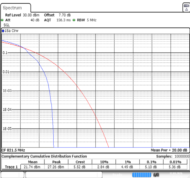
Band26(814-824)-5MHz-16QAM-26765-1RB#0-PASS
