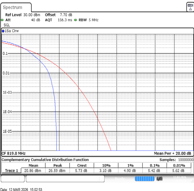
Band26(814-824)-5MHz-64QAM-26740-1RB#0-PASS
