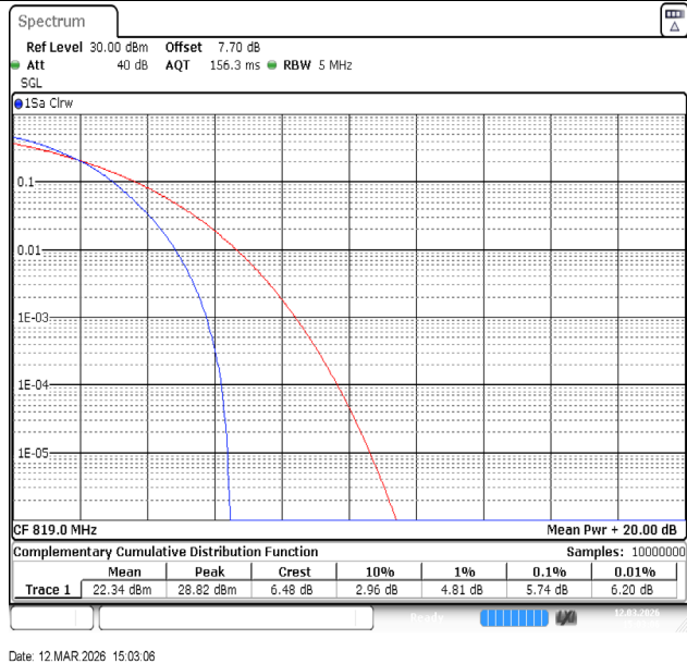
Band26(814-824)-5MHz-16QAM-26740-25RB#0-PASS
