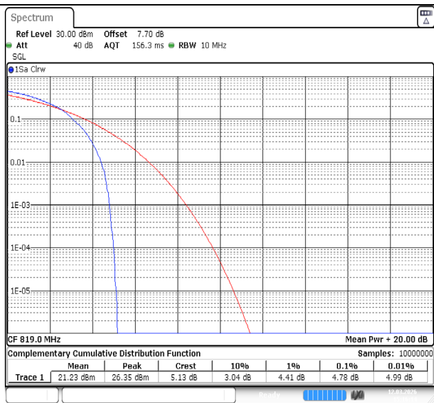
Band26(814-824)-10MHz-64QAM-26740-1RB#0-PASS
