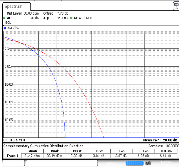
Band26(814-824)-5MHz-64QAM-26715-25RB#0-PASS
