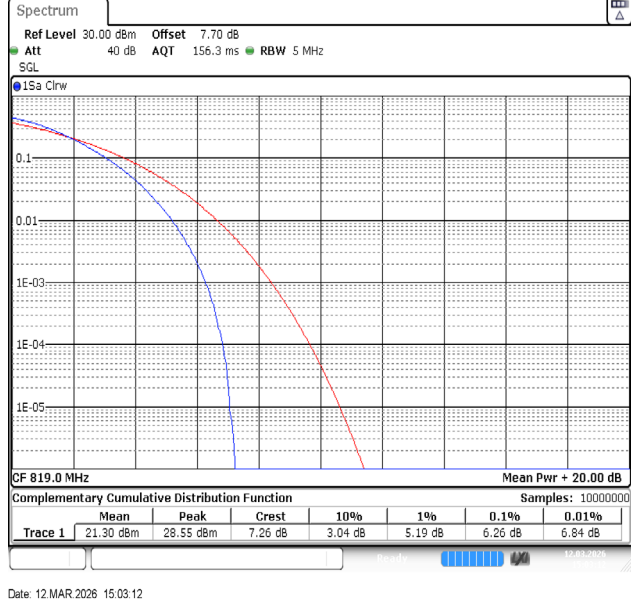
Band26(814-824)-5MHz-64QAM-26740-25RB#0-PASS
