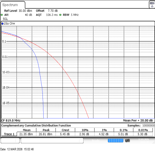
Band26(814-824)-5MHz-16QAM-26740-1RB#0-PASS
