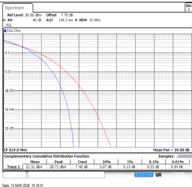
Band26(814-824)-10MHz-64QAM-26740-50RB#0-PASS
