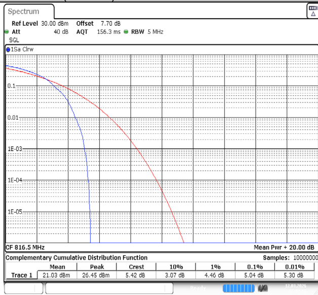
Band26(814-824)-5MHz-QPSK-26715-1RB#0-PASS
