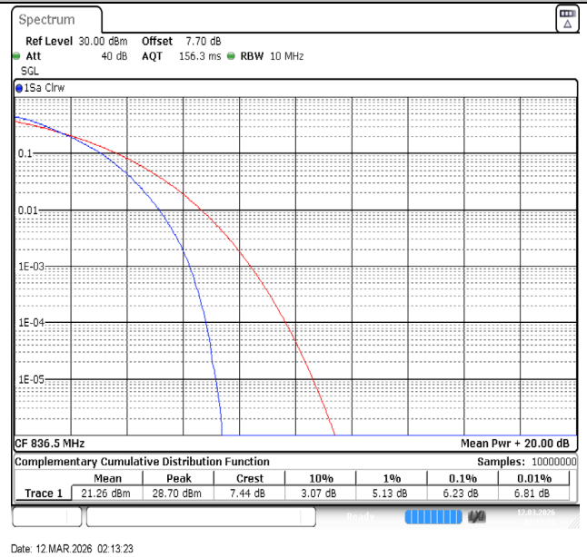
Band5-10MHz-64QAM-20525-50RB#0-PASS
