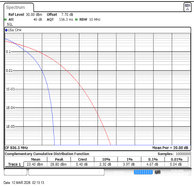
Band5-10MHz-QPSK-20525-50RB#0-PASS
