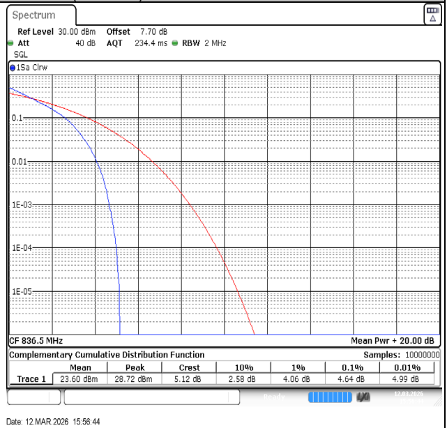
Band26(824-849)-1.4MHz-QPSK-26915-6RB#0-PASS
