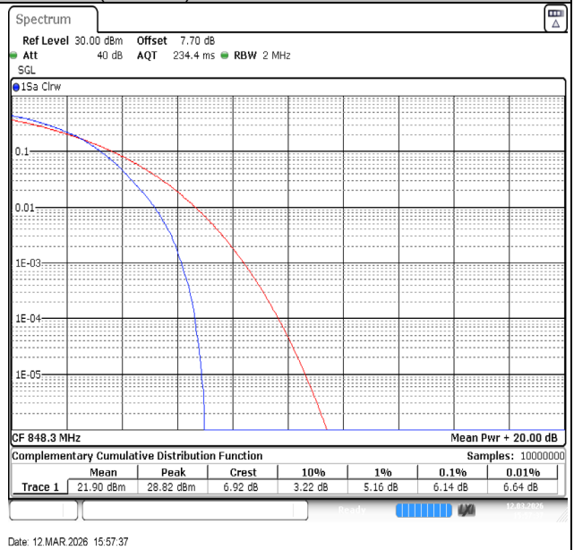
Band26(824-849)-1.4MHz-64QAM-27033-6RB#0-PASS
