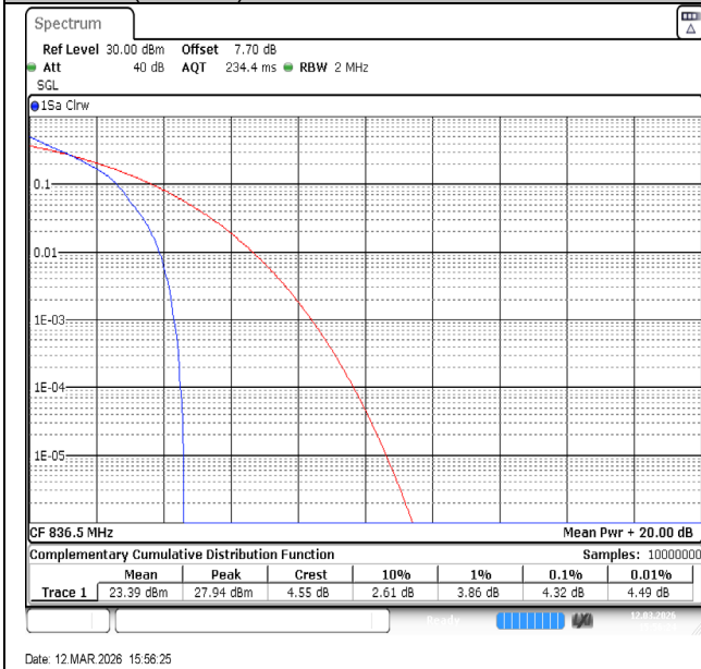
Band26(824-849)-1.4MHz-QPSK-26915-1RB#0-PASS
