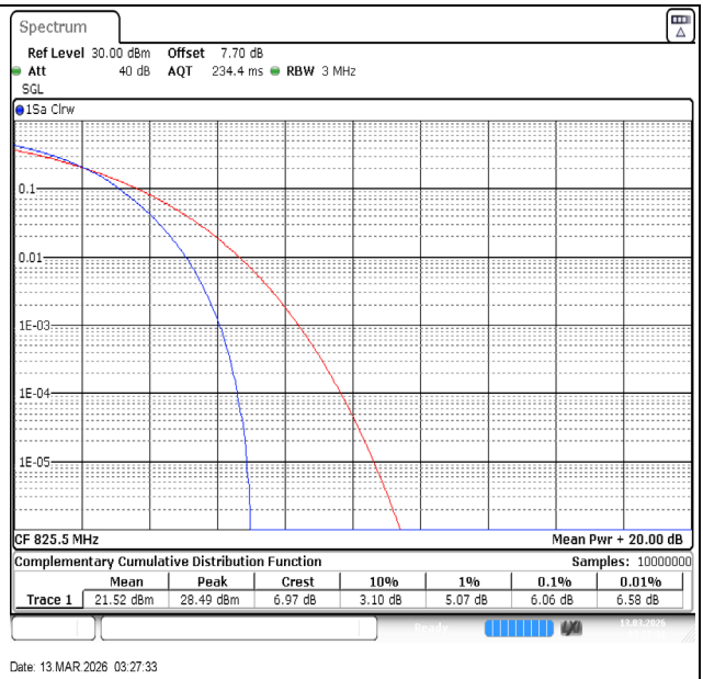
Band26(824-849)-3MHz-64QAM-26805-15RB#0-PASS
