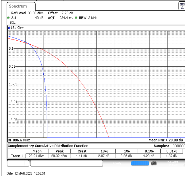
Band26(824-849)-1.4MHz-16QAM-26915-1RB#0-PASS
