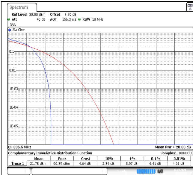
Band5-10MHz-16QAM-20525-1RB#0-PASS
