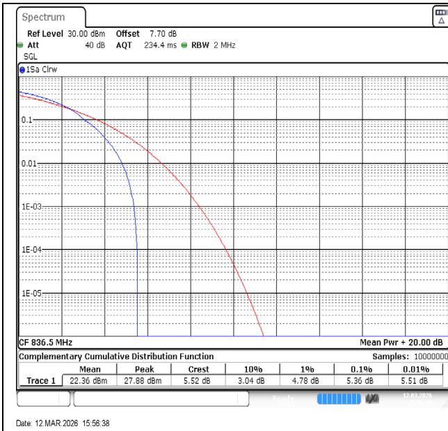
Band26(824-849)-1.4MHz-64QAM-26915-1RB#0-PASS
