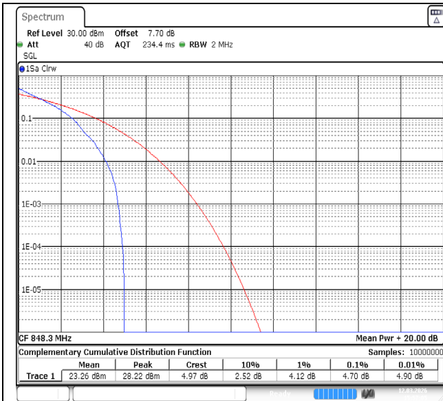
Band26(824-849)-1.4MHz-QPSK-27033-1RB#0-PASS
