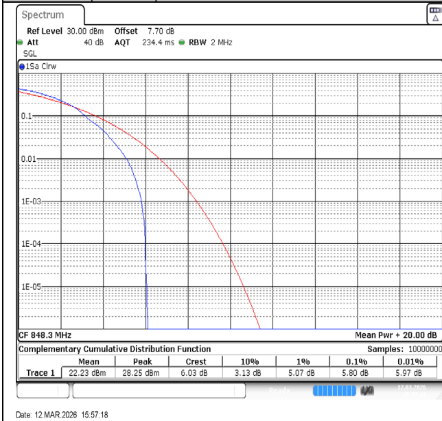
Band26(824-849)-1.4MHz-64QAM-27033-1RB#0-PASS
