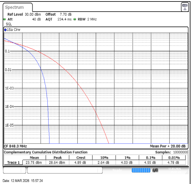
Band26(824-849)-1.4MHz-QPSK-27033-6RB#0-PASS
