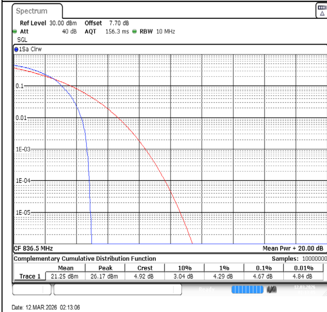
Band5-10MHz-64QAM-20525-1RB#0-PASS
