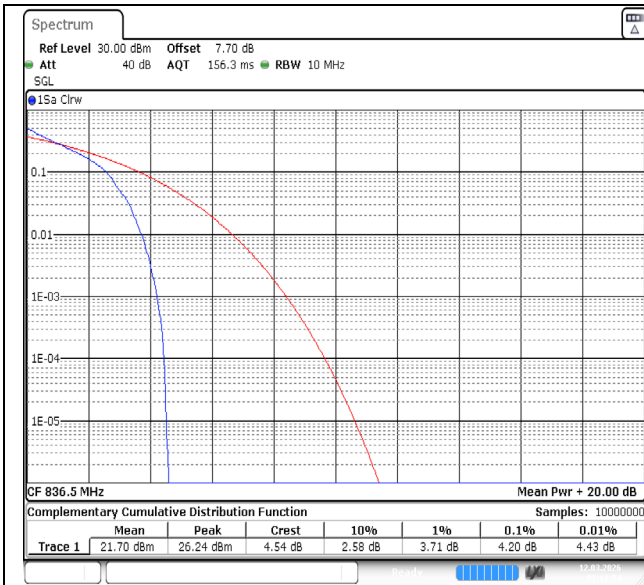
Band5-10MHz-QPSK-20525-1RB#0-PASS
