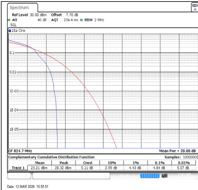
Band26(824-849)-1.4MHz-16QAM-26797-1RB#0-PASS
