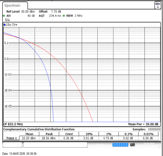
Band26(824-849)-3MHz-16QAM-26805-15RB#0-PASS
