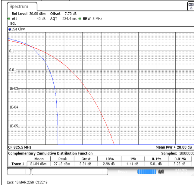
Band26(824-849)-3MHz-16QAM-26805-1RB#0-PASS
