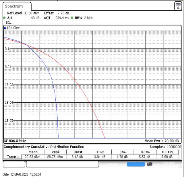
Band26(824-849)-1.4MHz-16QAM-26915-6RB#0-PASS
