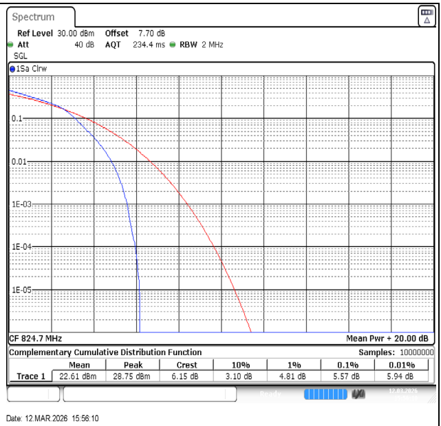
Band26(824-849)-1.4MHz-16QAM-26797-6RB#0-PASS
