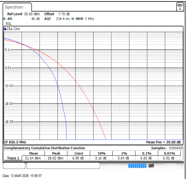
Band26(824-849)-1.4MHz-64QAM-26915-6RB#0-PASS
