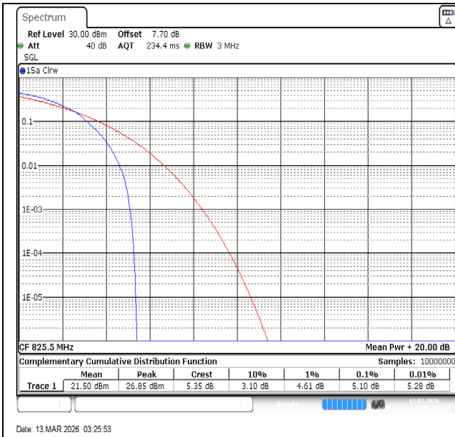
Band26(824-849)-3MHz-64QAM-26805-1RB#0-PASS
