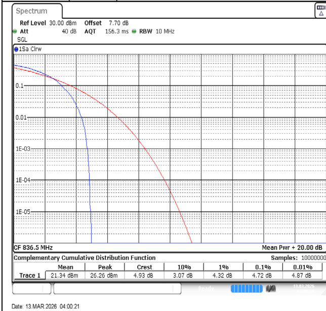
Band26(824-849)-10MHz-64QAM-26915-1RB#0-PASS
