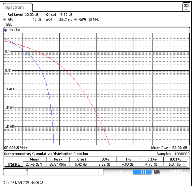
Band26(824-849)-10MHz-QPSK-26915-50RB#0-PASS
