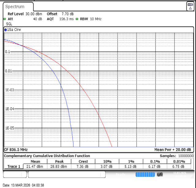
Band26(824-849)-10MHz-64QAM-26915-50RB#0-PASS
