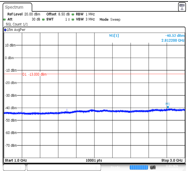
Band5-10MHz-QPSK-20600-1RB#49-1000~3000-PASS
