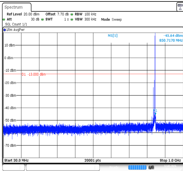
Band5-10MHz-QPSK-20600-1RB#49-30~1000-PASS
