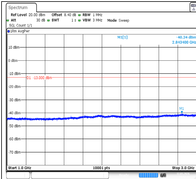
Band26(824-849)-1.4MHz-QPSK-26915-6RB#0-1000~3000-PASS
