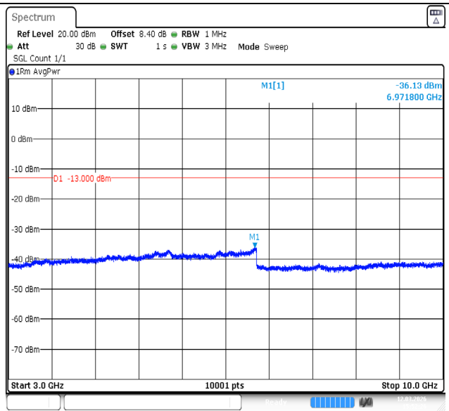
Band26(824-849)-1.4MHz-QPSK-26915-6RB#0-3000~10000-PASS
