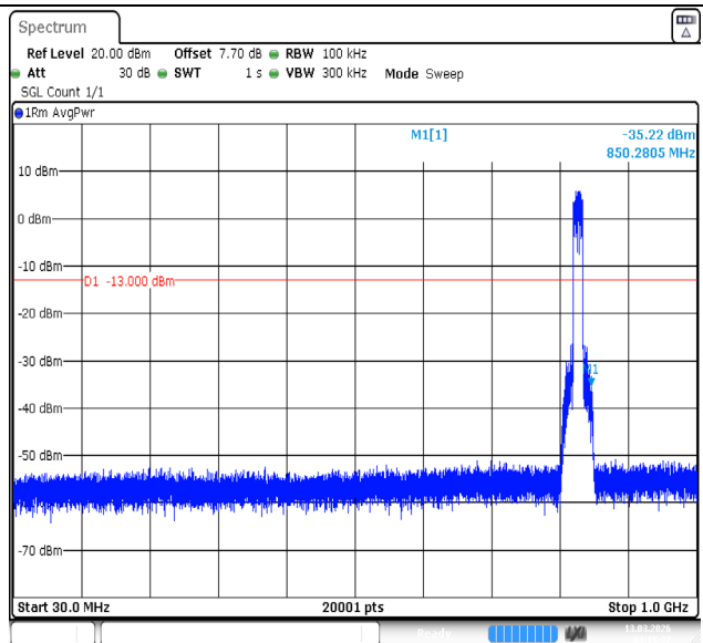
Band26(824-849)-15MHz-QPSK-26865-75RB#0-30~1000-PASS
