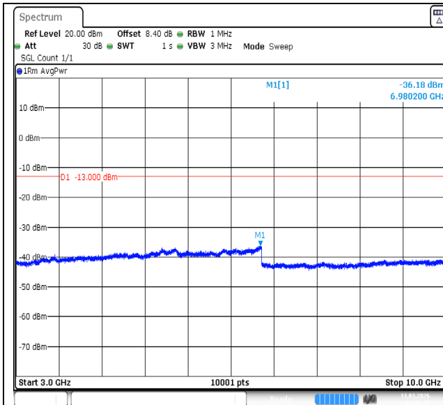
Band26(824-849)-15MHz-QPSK-26865-1RB#74-3000~10000-PASS
