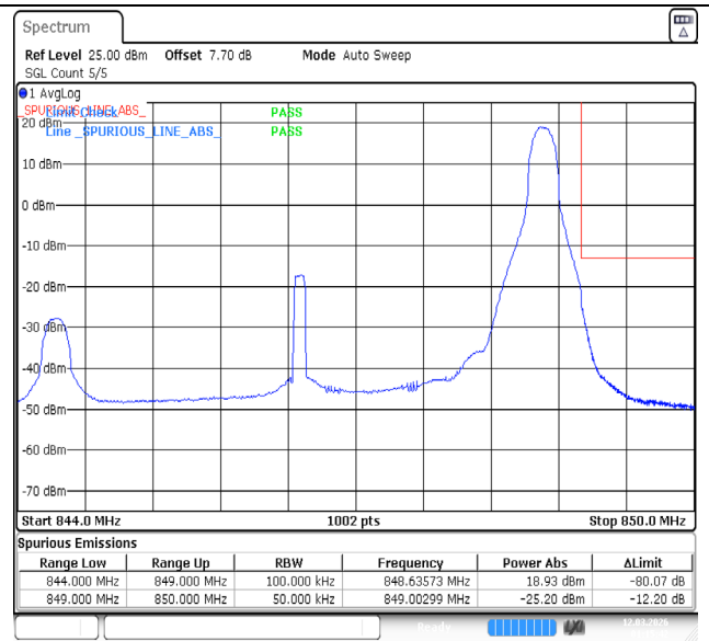
Band5-5MHz-64QAM-20625-1RB#24-PASS
