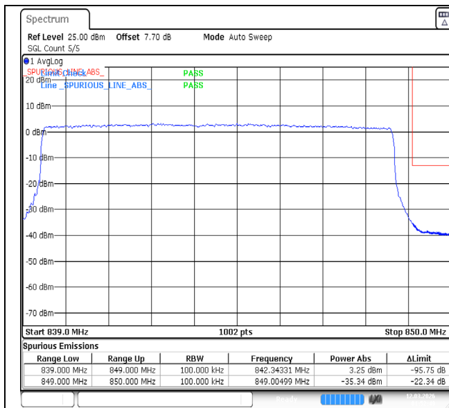
Band5-10MHz-64QAM-20600-50RB#0-PASS
