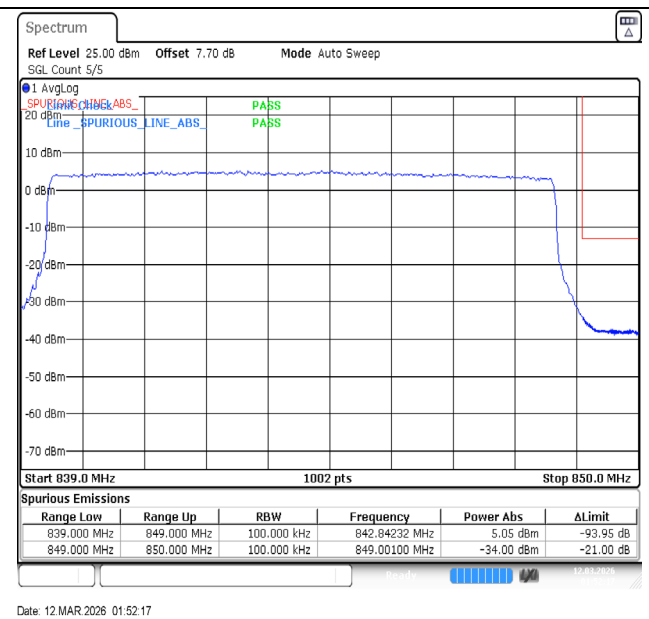
Band5-10MHz-QPSK-20600-50RB#0-PASS
