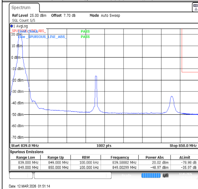
Band5-10MHz-64QAM-20600-1RB#0-PASS
