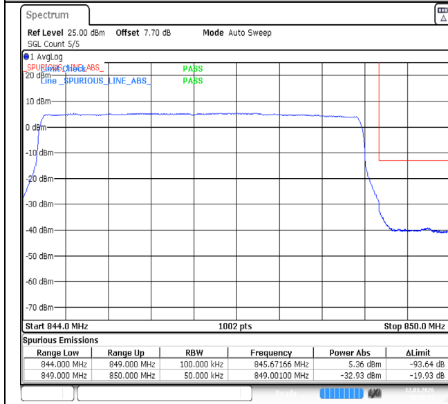
Band5-5MHz-64QAM-20625-1RB#0-PASS
