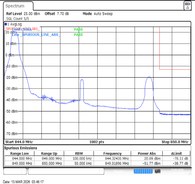
Band26(824-849)-5MHz-QPSK-27015-1RB#0-PASS
