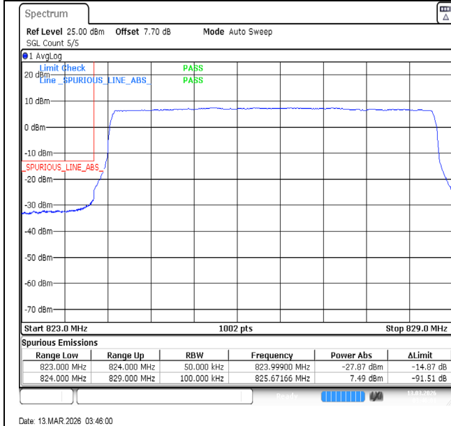
Band26(824-849)-5MHz-QPSK-26815-25RB#0-PASS
