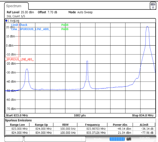
Band5-10MHz-16QAM-20450-1RB#49-PASS
