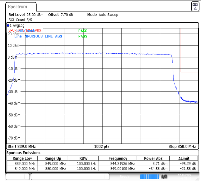
Band5-10MHz-16QAM-20600-1RB#0-PASS
