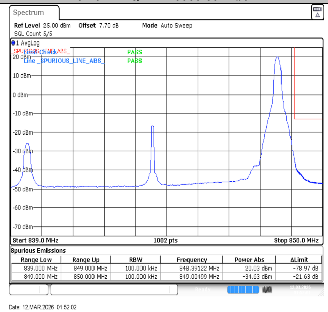
Band5-10MHz-64QAM-20600-1RB#49-PASS
