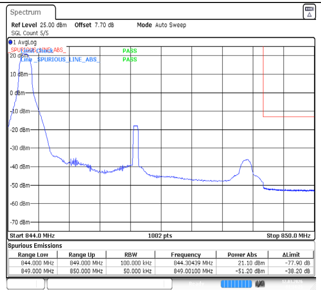
Band5-5MHz-QPSK-20625-1RB#0-PASS
