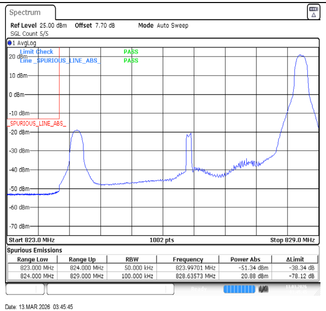
Band26(824-849)-5MHz-QPSK-26815-1RB#24-PASS
