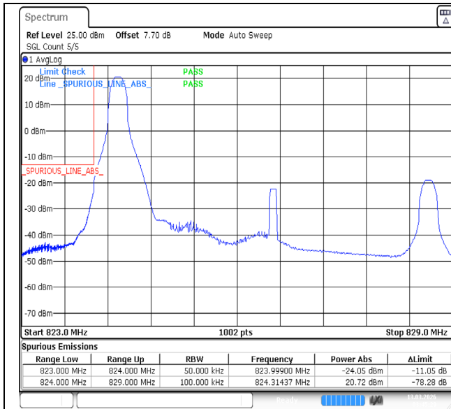
Band26(824-849)-5MHz-QPSK-26815-1RB#0-PASS
