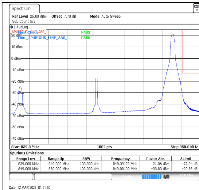
Band5-10MHz-QPSK-20600-1RB#49-PASS
