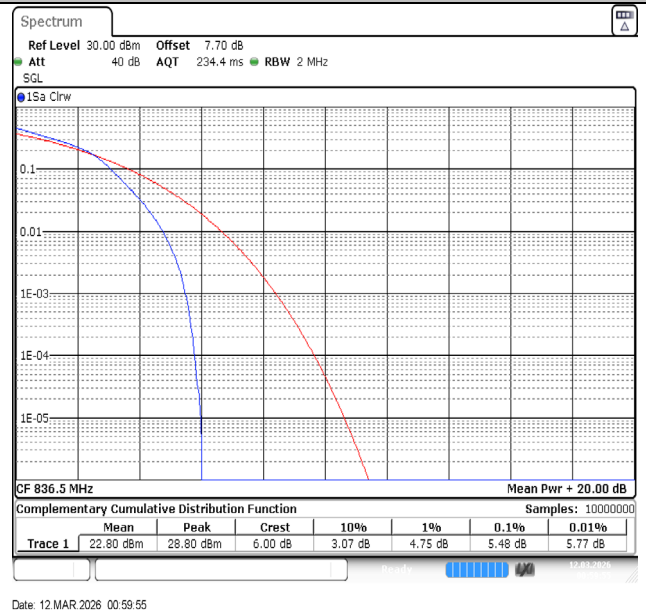
Band5-1.4MHz-16QAM-20525-6RB#0-PASS
