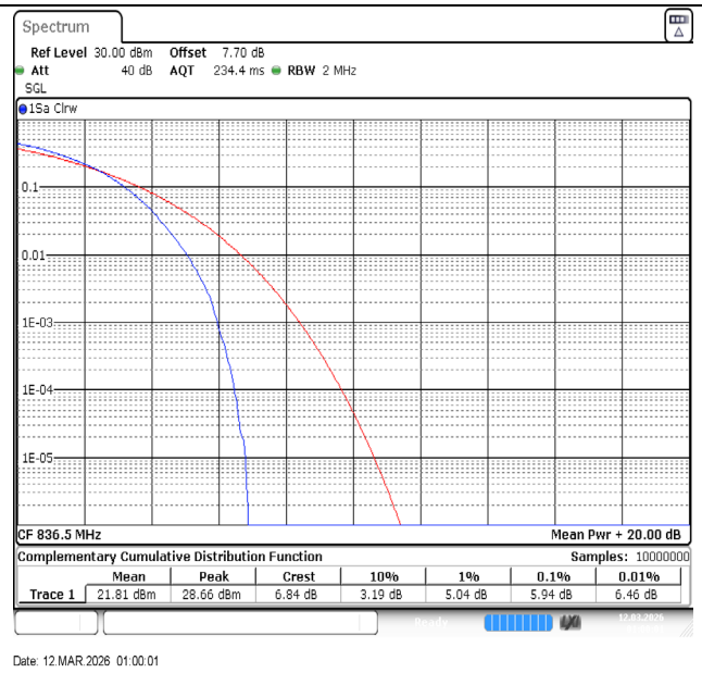
Band5-1.4MHz-64QAM-20525-6RB#0-PASS
