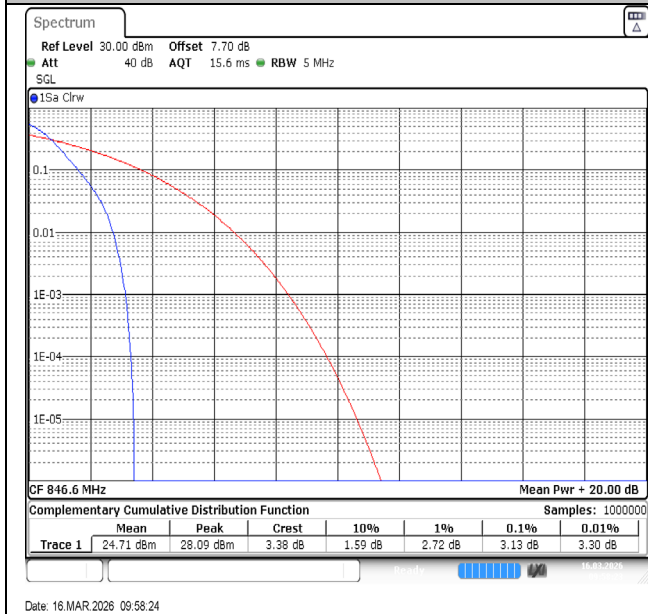
Band5-4233-PASS
