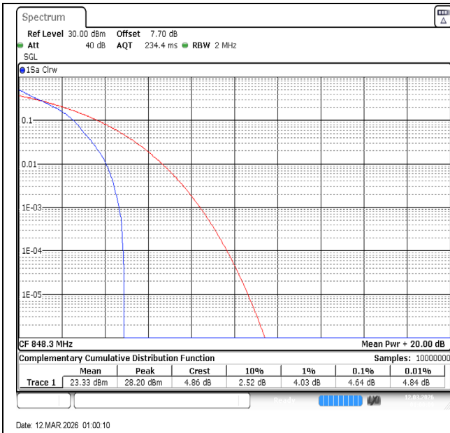
Band5-1.4MHz-QPSK-20643-1RB#0-PASS
