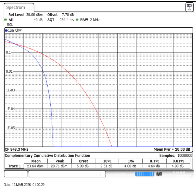
Band5-1.4MHz-QPSK-20643-6RB#0-PASS
