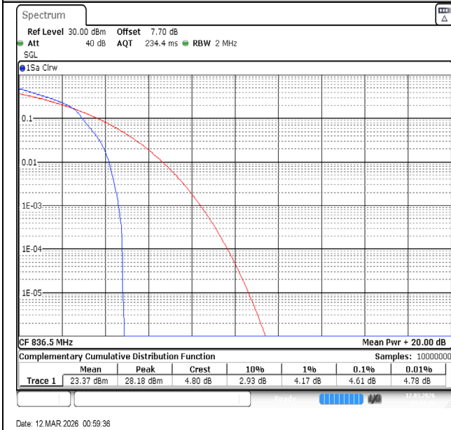
Band5-1.4MHz-16QAM-20525-1RB#0-PASS
