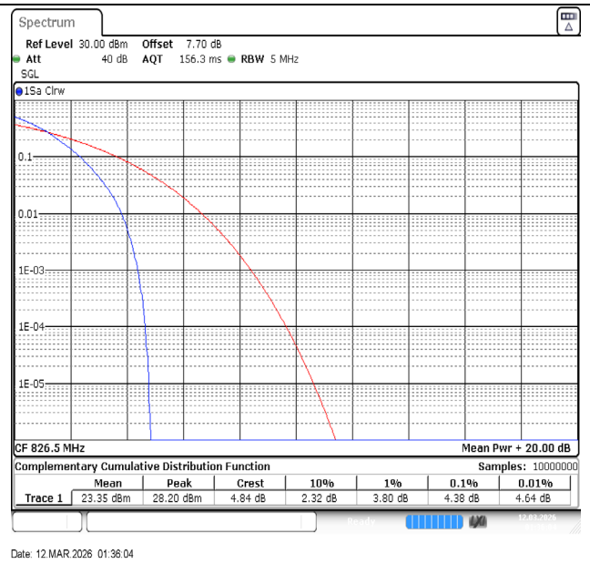
Band5-5MHz-QPSK-20425-25RB#0-PASS
