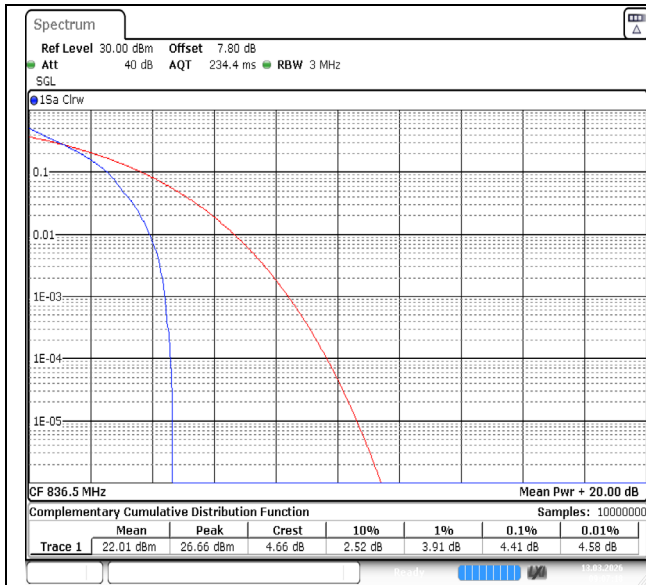
Band5-3MHz-QPSK-20525-1RB#0-PASS
