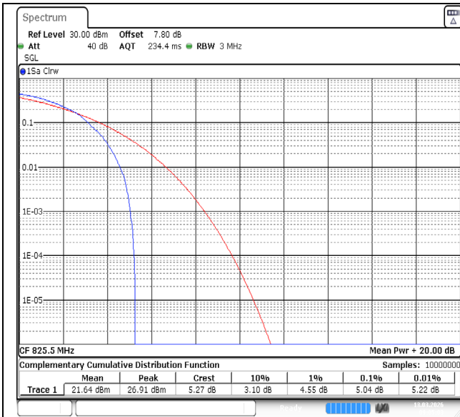
Band5-3MHz-64QAM-20415-1RB#0-PASS
