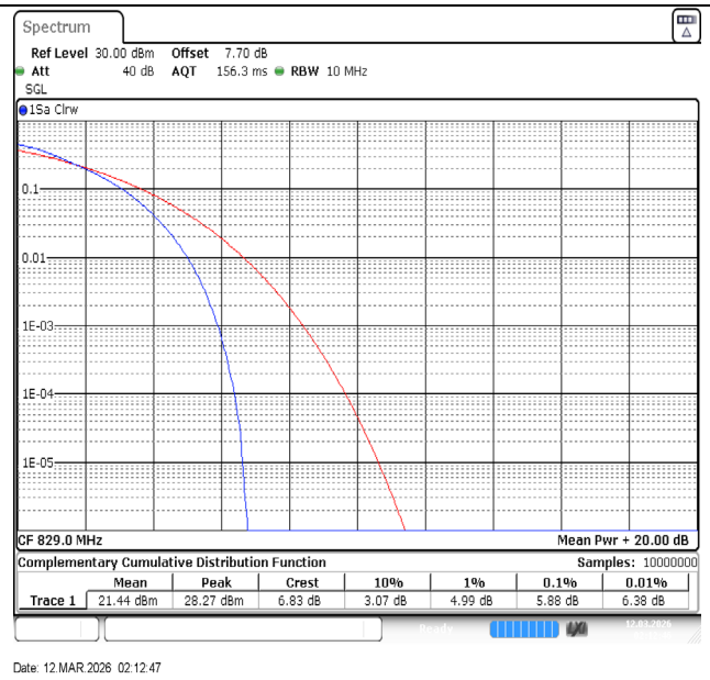
Band5-10MHz-64QAM-20450-50RB#0-PASS
