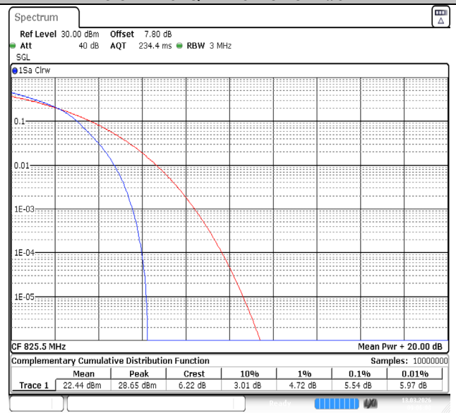
Band5-3MHz-64QAM-20415-15RB#0-PASS
