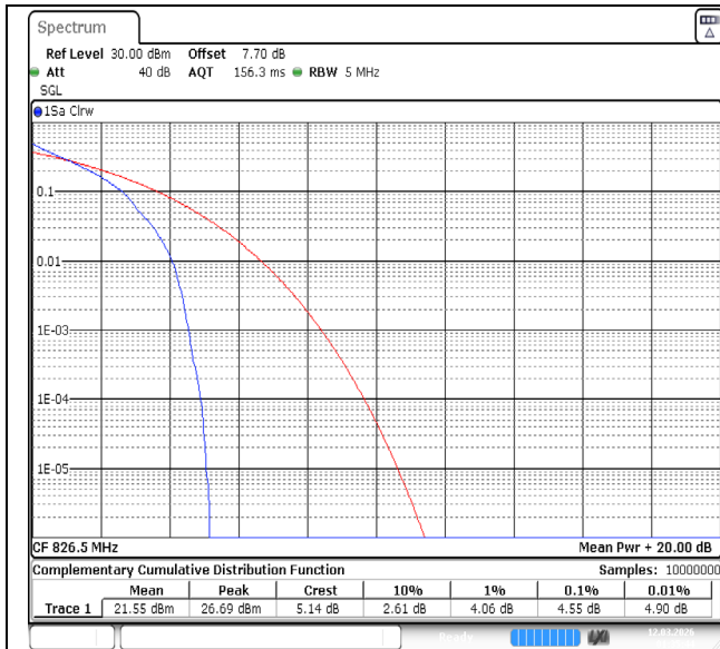
Band5-5MHz-QPSK-20425-1RB#0-PASS
