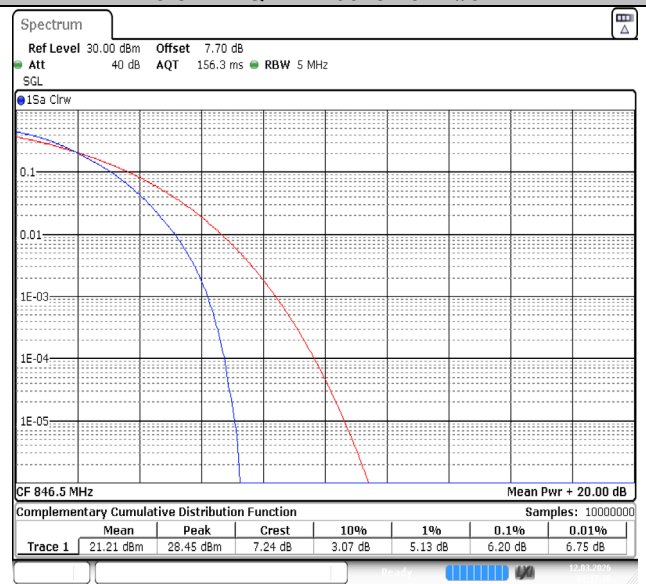
Band5-5MHz-QPSK-20625-25RB#0-PASS
