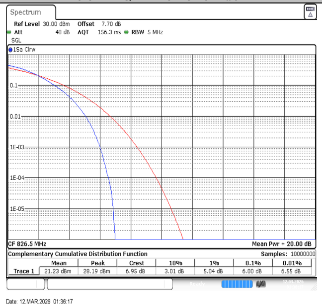
Band5-5MHz-64QAM-20425-25RB#0-PASS
