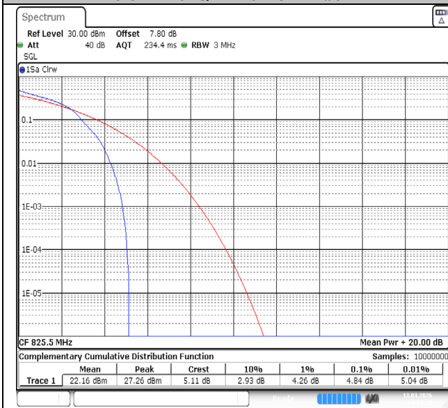
Band5-3MHz-64QAM-20415-1RB#0-PASS
