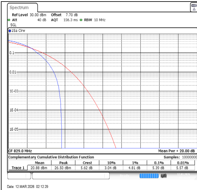
Band5-10MHz-64QAM-20450-1RB#0-PASS
