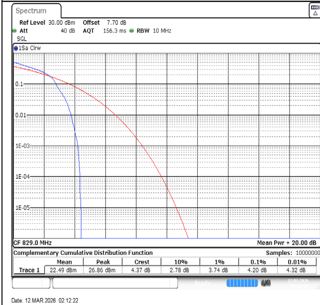
Band5-10MHz-16QAM-20450-1RB#0-PASS
