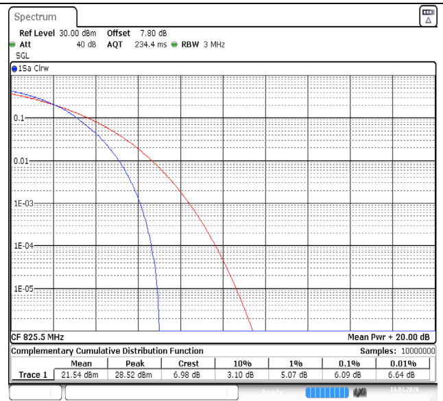
Band5-3MHz-64QAM-20415-15RB#0-PASS
