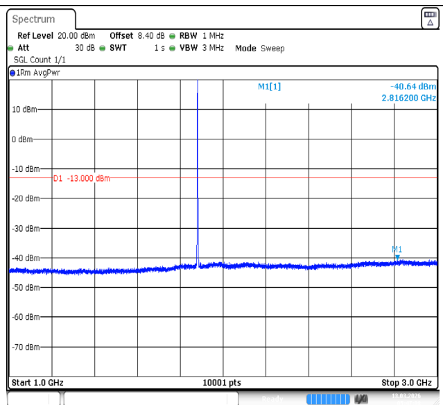
Band2-1.4MHz-QPSK-18900-1RB#5-1000~3000-PASS
