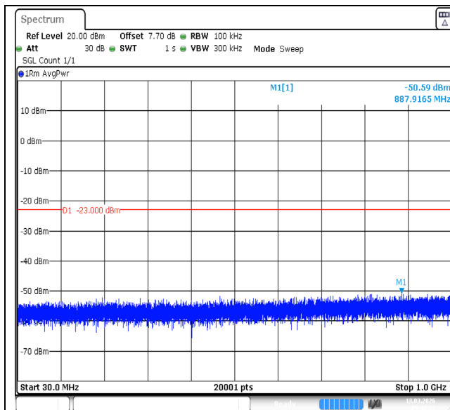
Band2-1.4MHz-QPSK-18900-1RB#5-30~1000-PASS
