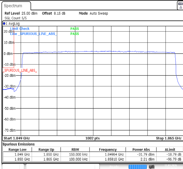
Band2-15MHz-QPSK-18675-1RB#0-PASS
