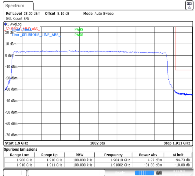
Band2-10MHz-QPSK-19150-50RB#0-PASS
