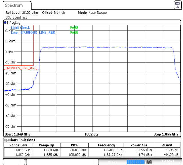
Band2-5MHz-64QAM-18625-25RB#0-PASS
