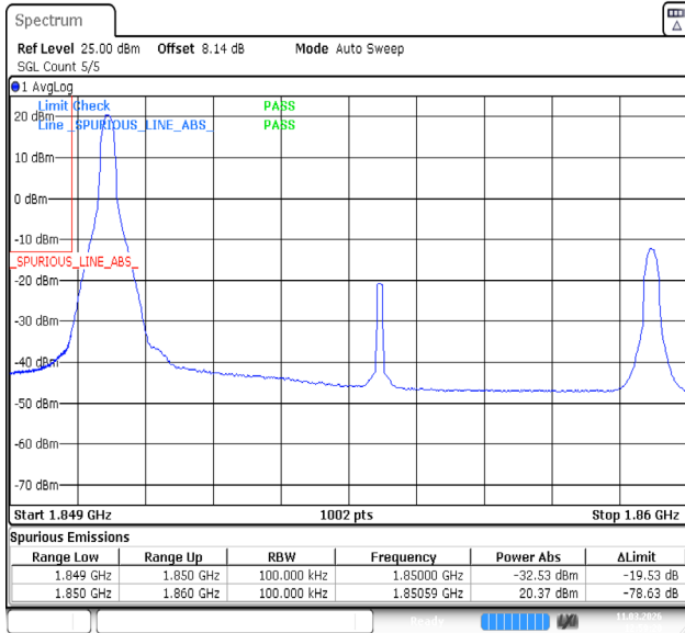
Band2-10MHz-16QAM-18650-1RB#0-PASS
