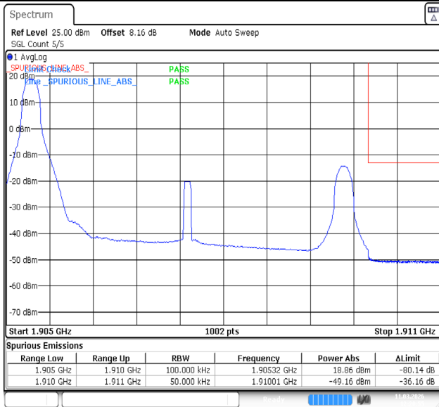
Band2-5MHz-64QAM-19175-1RB#0-PASS
