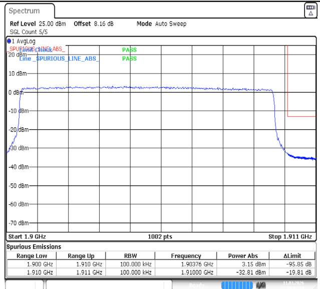
Band2-10MHz-16QAM-19150-50RB#0-PASS
