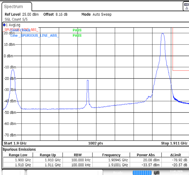
Band2-10MHz-64QAM-19150-50RB#0-PASS
