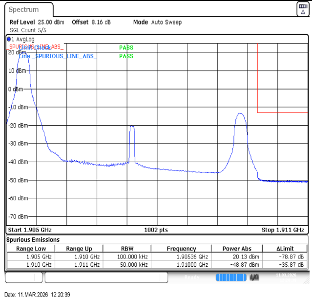
Band2-5MHz-16QAM-19175-1RB#0-PASS
