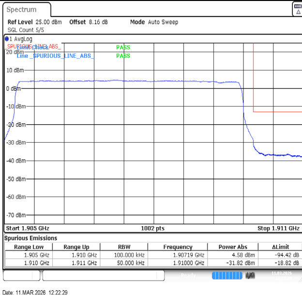
Band2-5MHz-64QAM-19175-25RB#0-PASS
