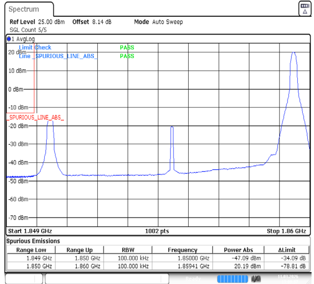
Band2-10MHz-16QAM-18650-1RB#49-PASS
