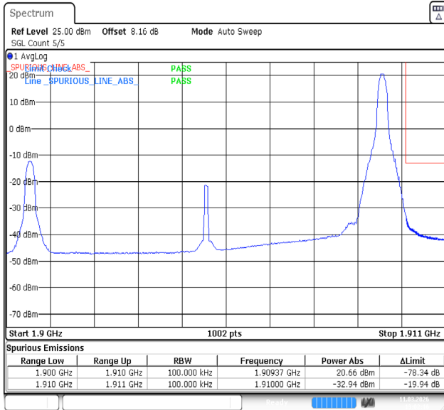
Band2-10MHz-QPSK-19150-1RB#49-PASS
