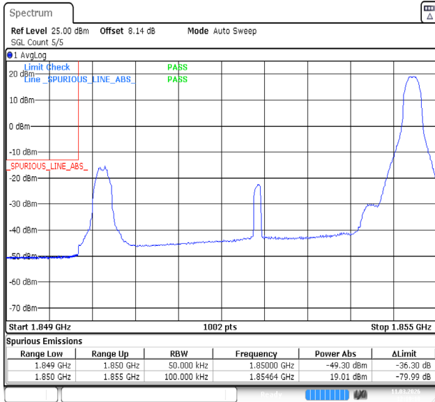
Band2-5MHz-64QAM-18625-1RB#24-PASS
