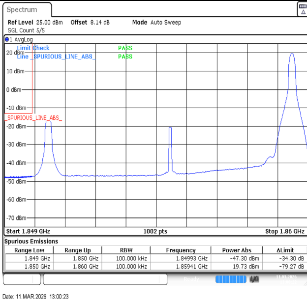
Band2-10MHz-64QAM-18650-1RB#49-PASS
