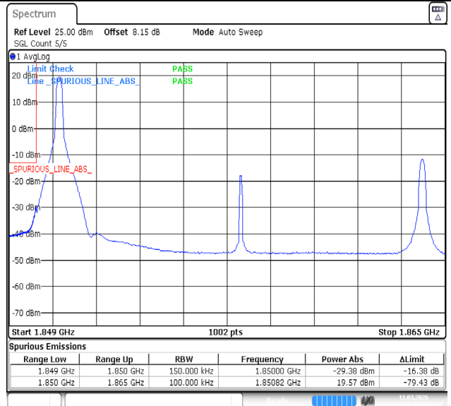
Band2-15MHz-QPSK-18675-1RB#74-PASS
