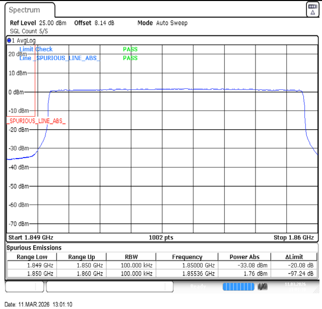
Band2-10MHz-64QAM-18650-50RB#0-PASS
