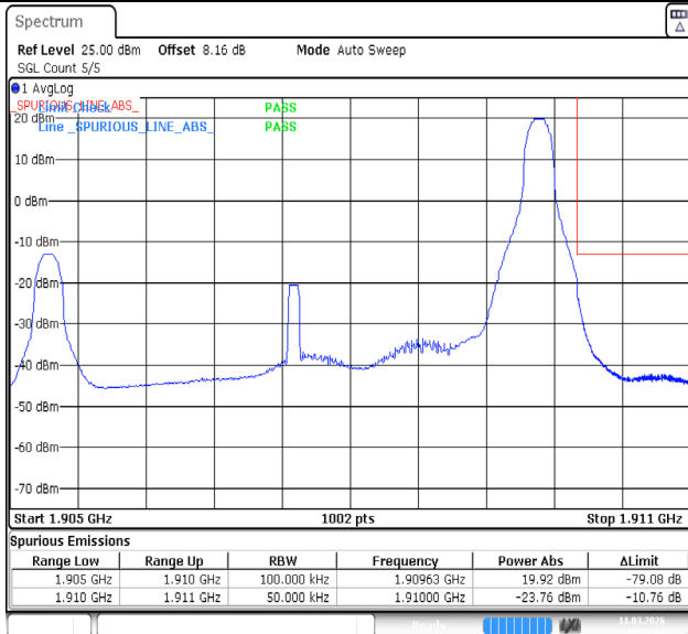
Band2-5MHz-16QAM-18625-25RB#0-PASS
