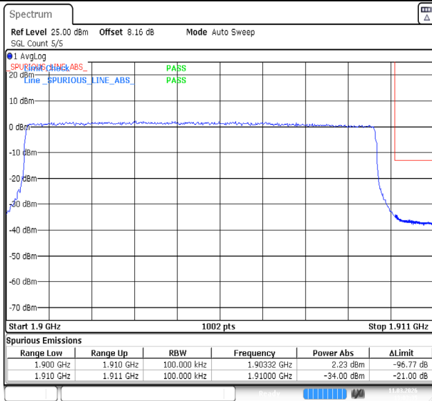
Band2-10MHz-64QAM-19150-50RB#0-PASS
