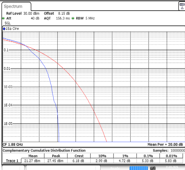
Band2-5MHz-64QAM-18900-1RB#0-PASS
