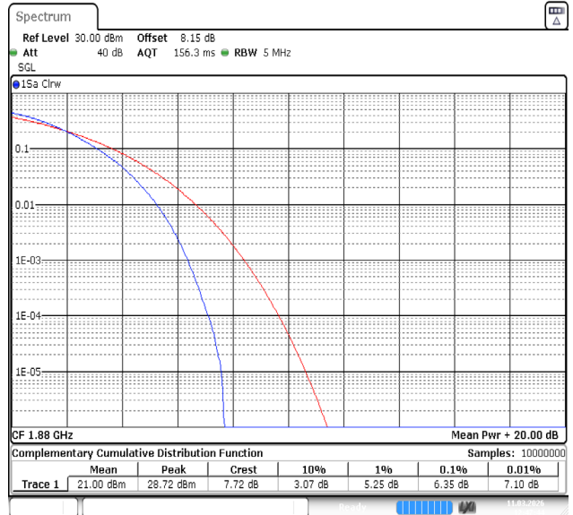
Band2-5MHz-64QAM-18900-25RB#0-PASS
