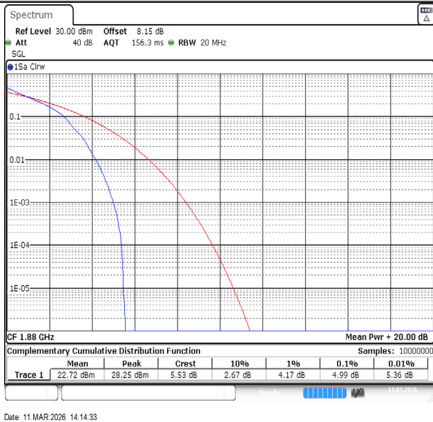
Band2-15MHz-QPSK-18900-1RB#0-PASS
