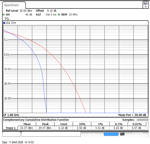
Band2-15MHz-QPSK-18900-75RB#0-PASS
