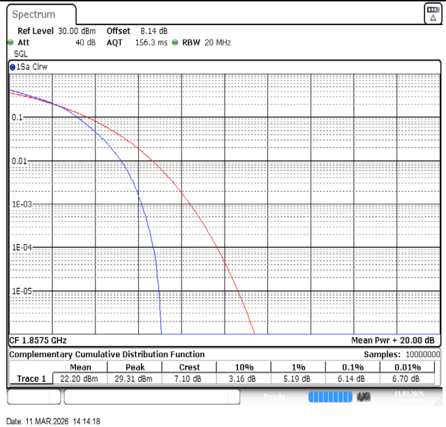
Band2-15MHz-16QAM-18675-75RB#0-PASS
