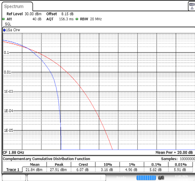
Band2-15MHz-64QAM-18900-1RB#0-PASS
