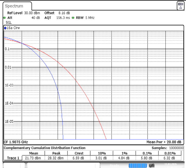
Band2-5MHz-16QAM-19175-25RB#0-PASS
