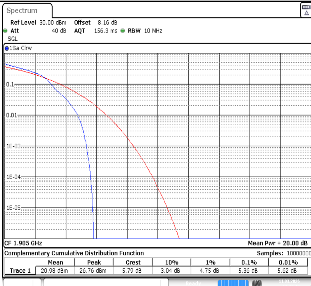
Band2-10MHz-64QAM-19150-1RB#0-PASS
