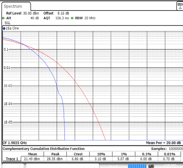
Band2-15MHz-QPSK-19125-1RB#0-PASS
