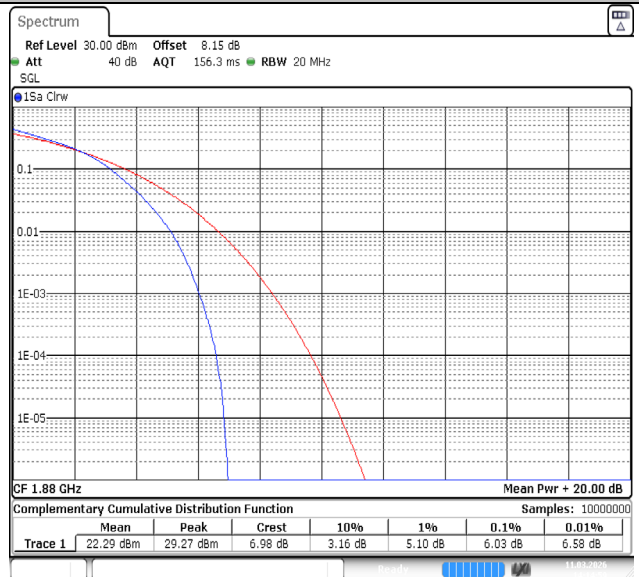
Band2-15MHz-64QAM-18900-75RB#0-PASS
