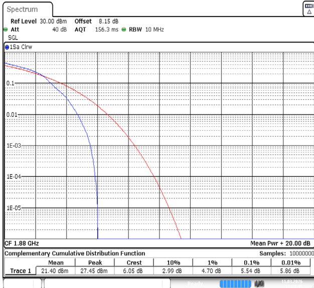
Band2-10MHz-16QAM-18900-1RB#0-PASS
