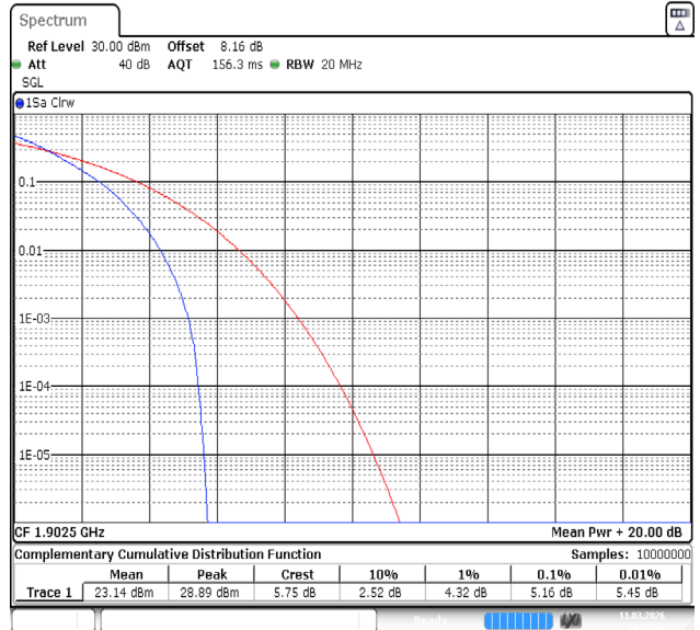
Band2-15MHz-QPSK-19125-75RB#0-PASS
