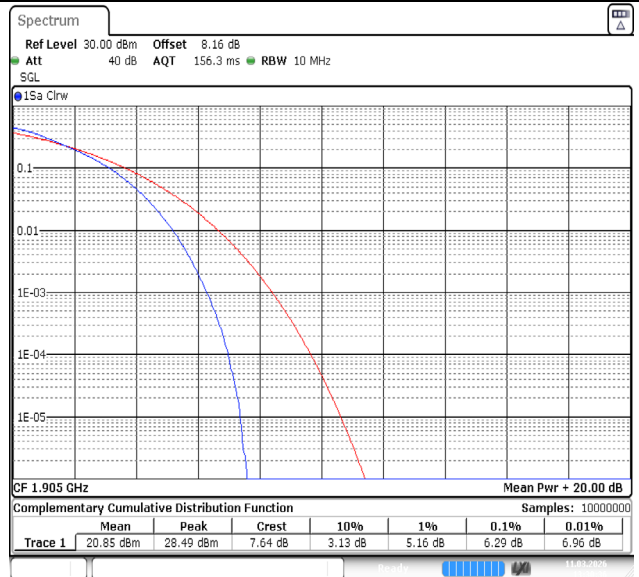
Band2-10MHz-64QAM-19150-50RB#0-PASS
