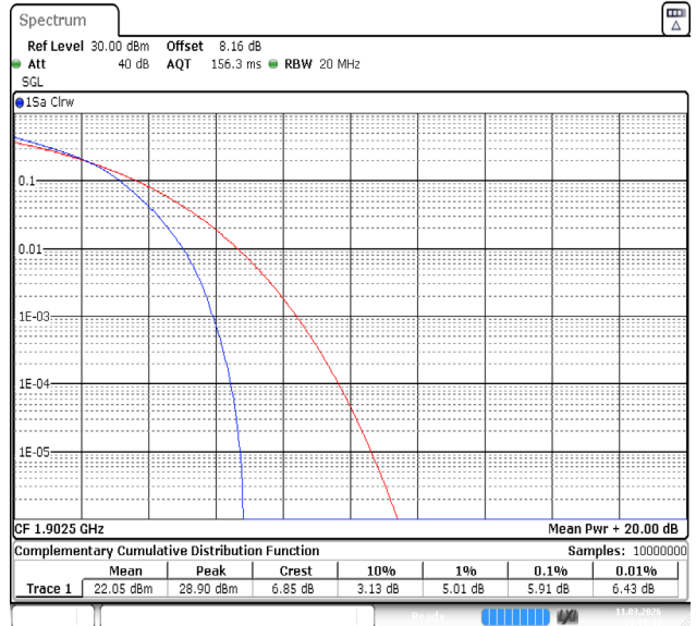
Band2-15MHz-16QAM-19125-75RB#0-PASS
