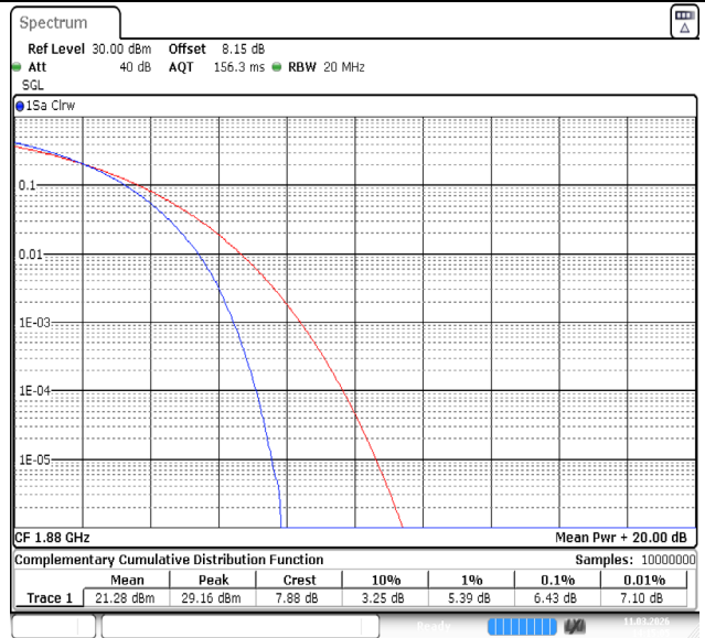
Band2-15MHz-64QAM-18900-75RB#0-PASS
