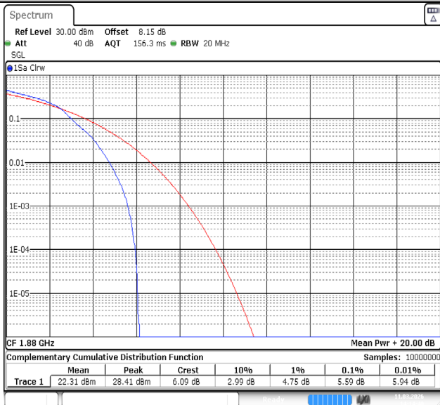
Band2-15MHz-64QAM-18900-1RB#0-PASS
