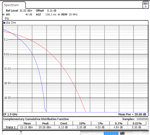
Band2-20MHz-16QAM-18900-100RB#0-PASS
