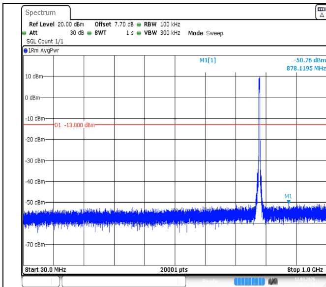
Band13-5MHz-QPSK-23255-25RB#0-30~1000-PASS
