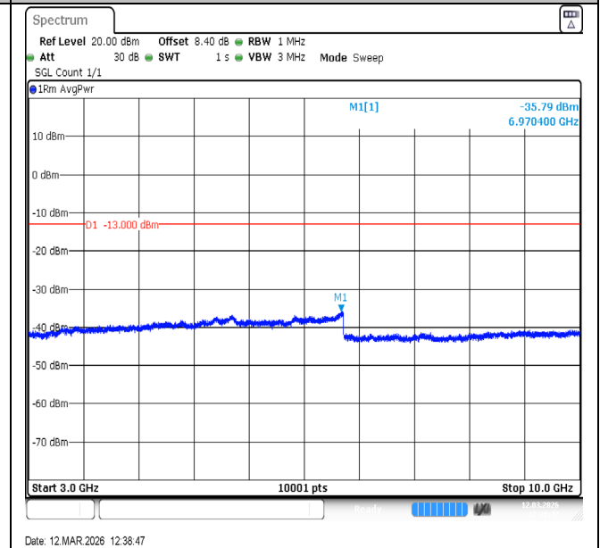
Band13-10MHz-QPSK-23230-50RB#0-3000~10000-PASS
