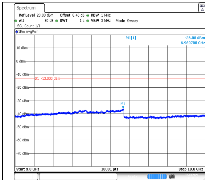
Band13-10MHz-QPSK-23230-1RB#49-3000~10000-PASS
