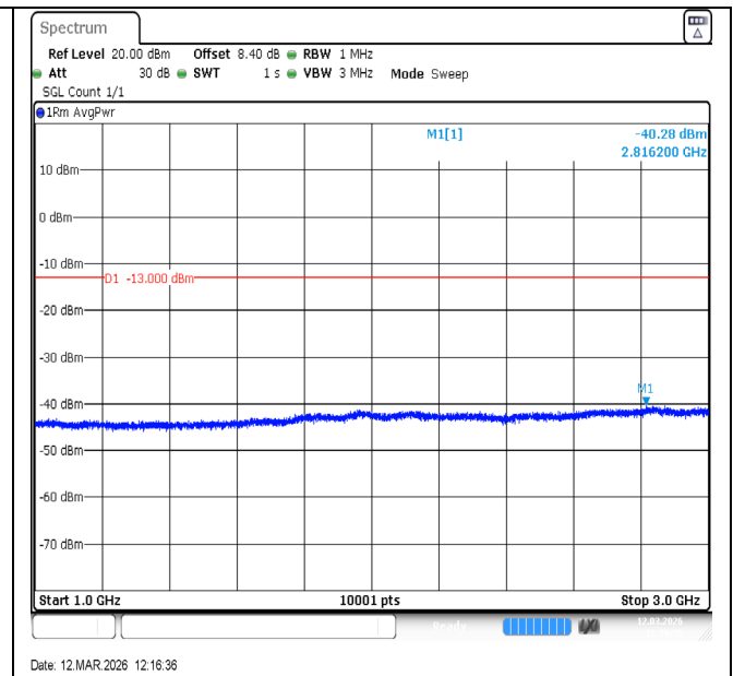
Band13-5MHz-QPSK-23255-25RB#0-1000~3000-PASS
