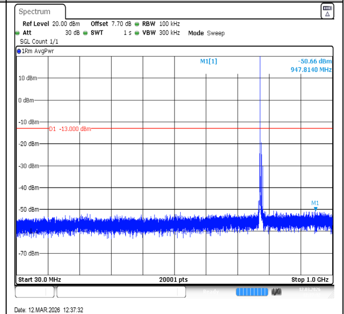
Band13-10MHz-QPSK-23230-1RB#0-30~1000-PASS
