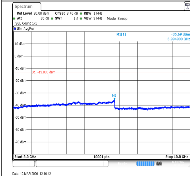
Band13-5MHz-QPSK-23255-25RB#0-3000~10000-PASS
