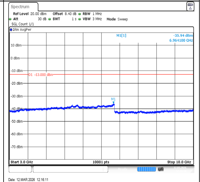
Band13-5MHz-QPSK-23255-1RB#24-3000~10000-PASS
