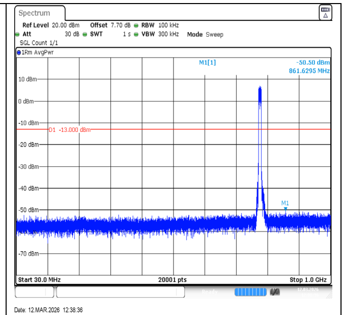
Band13-10MHz-QPSK-23230-50RB#0-30~1000-PASS
