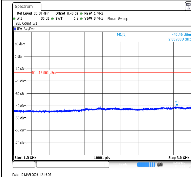
Band13-5MHz-QPSK-23255-1RB#24-1000~3000-PASS
