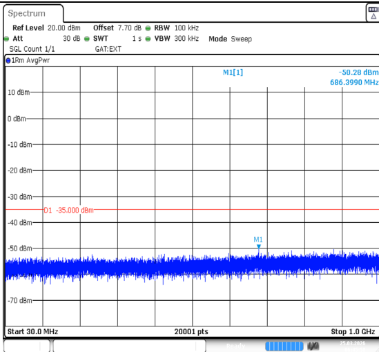
Band38-5MHz-QPSK-38000-1RB#0-30~1000-PASS
