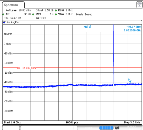
Band38-5MHz-QPSK-38000-1RB#0-1000~3000-PASS
