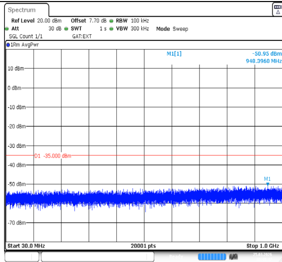
Band38-5MHz-QPSK-38225-1RB#0-30~1000-PASS
