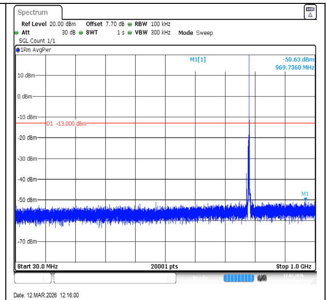
Band13-5MHz-QPSK-23255-1RB#24-30~1000-PASS
