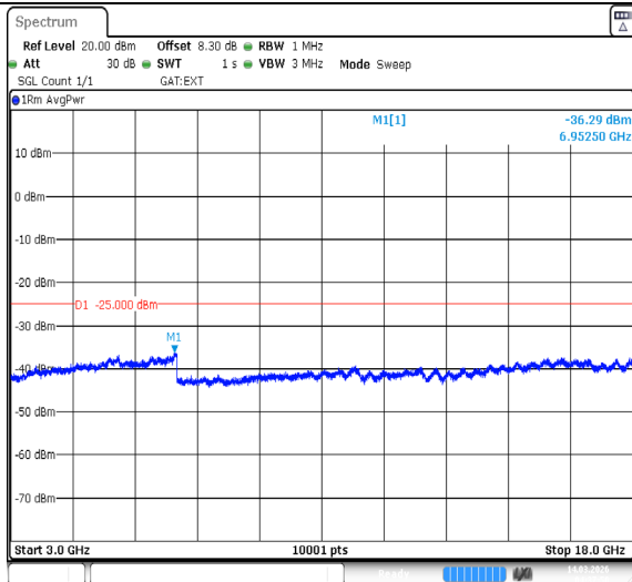
Band38-20MHz-QPSK-38150-1RB#99-3000~18000-PASS
