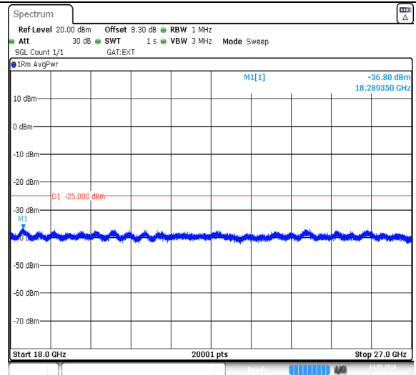
Band38-20MHz-QPSK-38150-1RB#99-18000~27000-PASS
