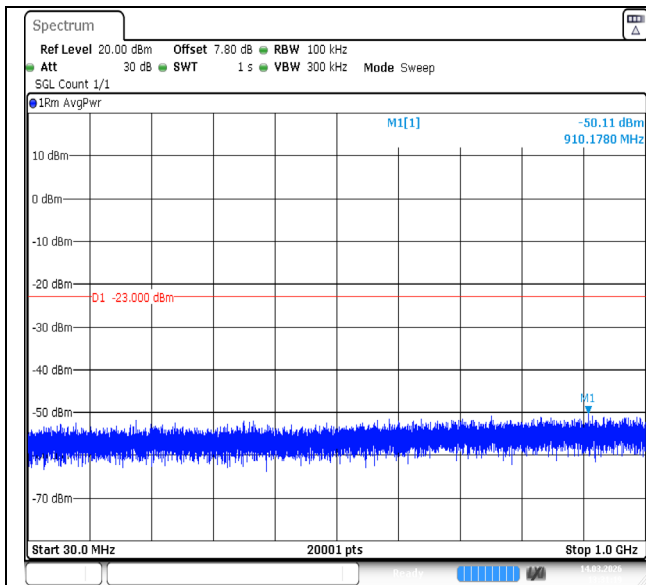
Band66-20MHz-QPSK-132322-1RB#0-30~1000-PASS
