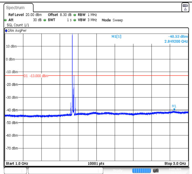
Band66-20MHz-QPSK-132322-1RB#0-1000~3000-PASS
