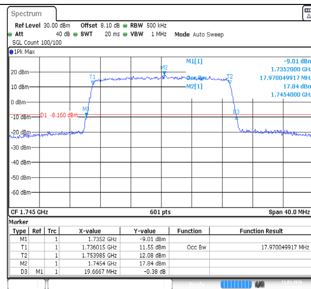
Band4-20MHz-16QAM-20300-100RB#0-PASS
